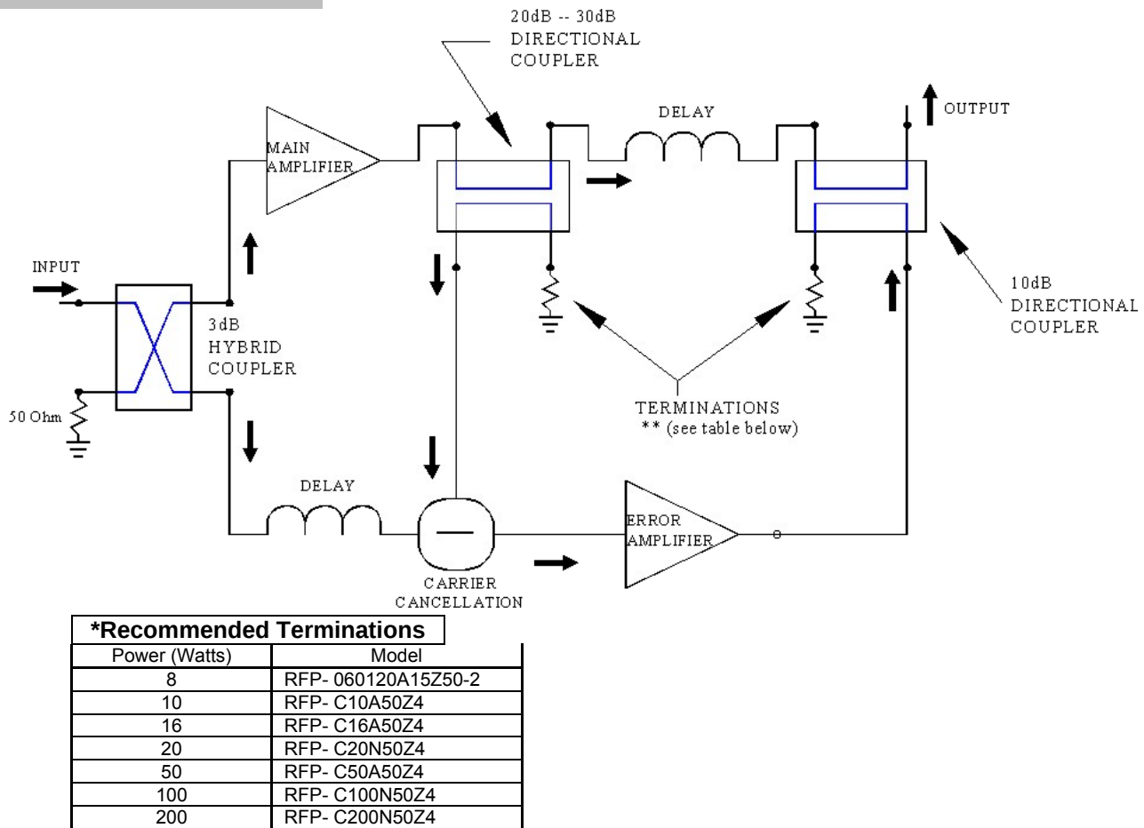
Figure ap.n.2-1. Generic Feed Forward Circuit Schematic
