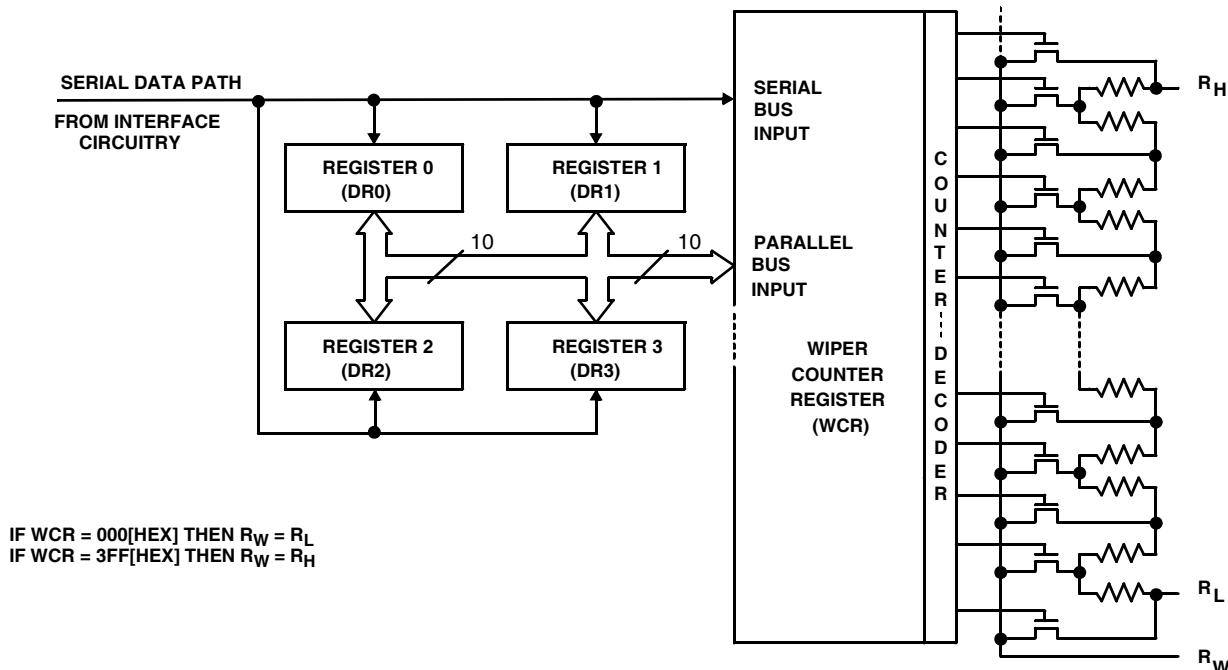
FIGURE 1. DETAILED POTENTIOMETER BLOCK DIAGRAM SERIAL INTERFACE DESCRIPTION
