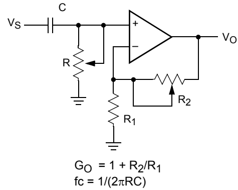
FIGURE 12. FILTER
