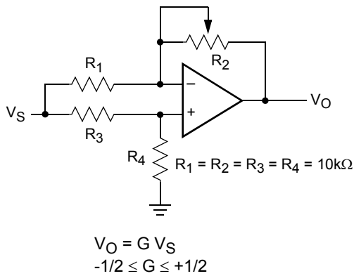
FIGURE 11. ATTENUATOR
