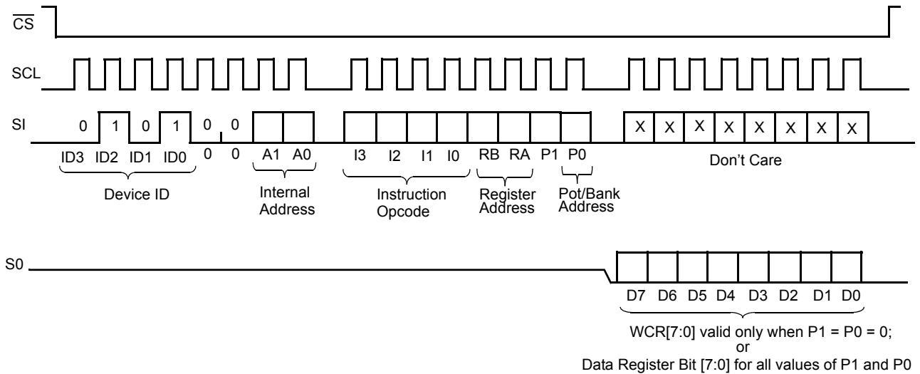
FIGURE 3. THREE-BYTE INSTRUCTION SEQUENCE (READ)
