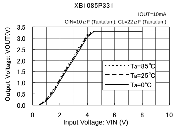
(2) Output Voltage vs. Input Voltage
