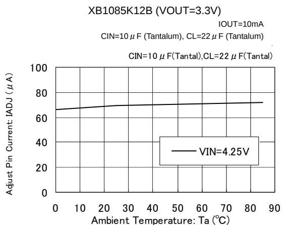
1(6) Adjust Pin Current vs. Ambient Temperature
