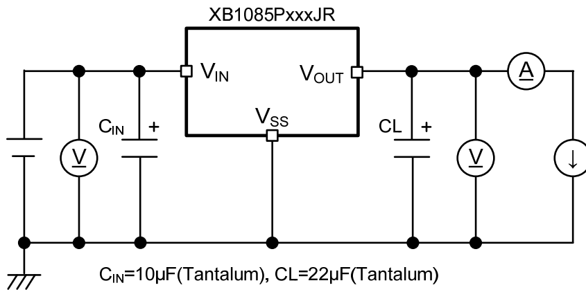
< Circuit ① >
