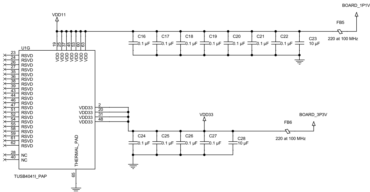
Figure 33. TUSB4041I-Q1 Power Implementation
