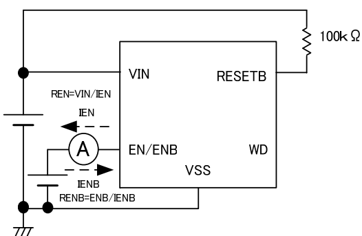
Circuit
