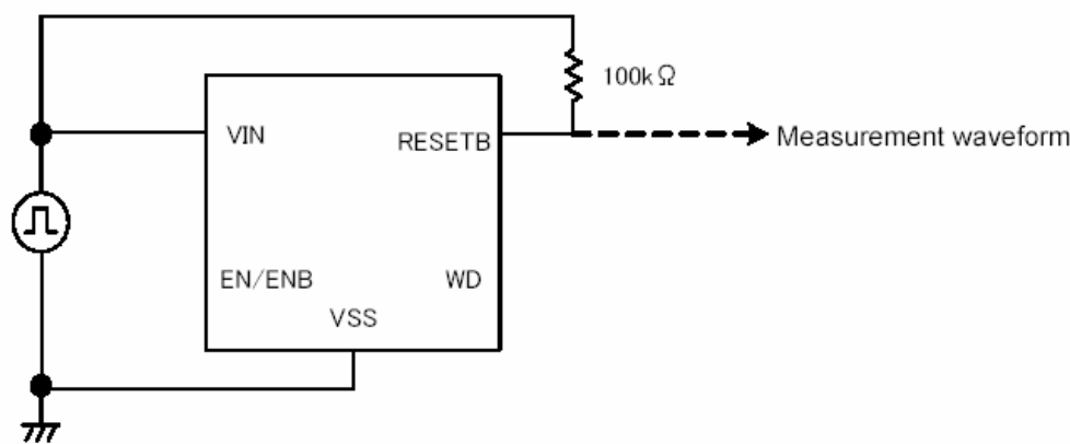
Circuit
