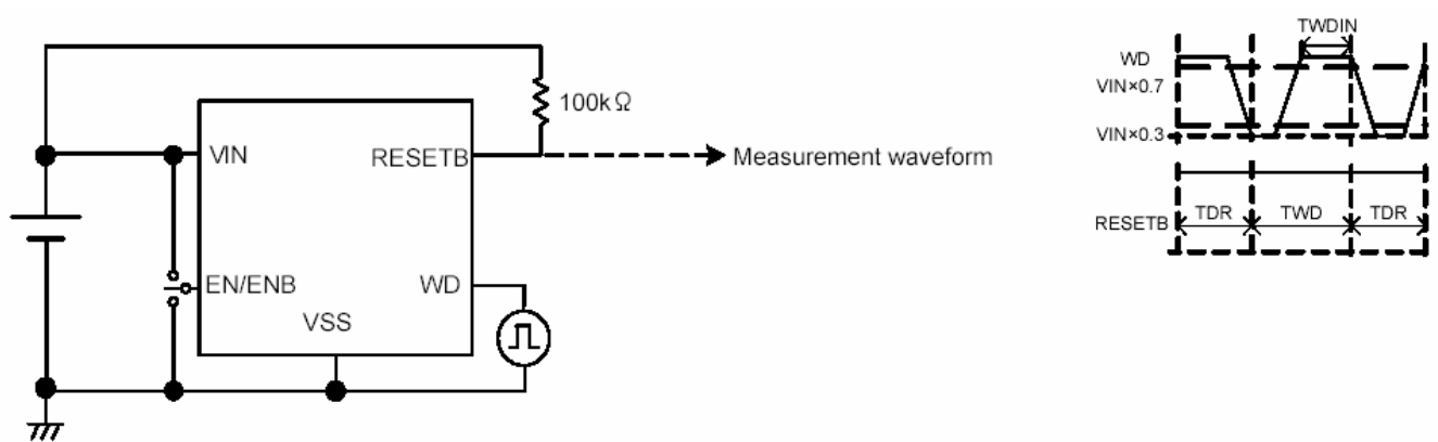
Circuit
