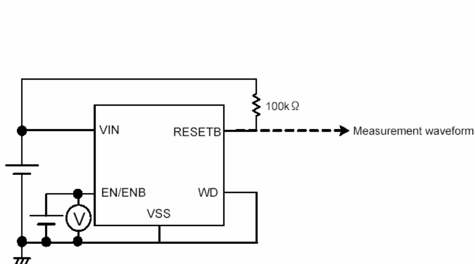
Circuit
