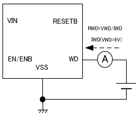
Circuit
