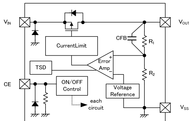
XC6223C/M series
