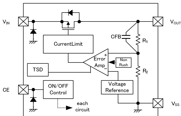
XC6223E/P series
