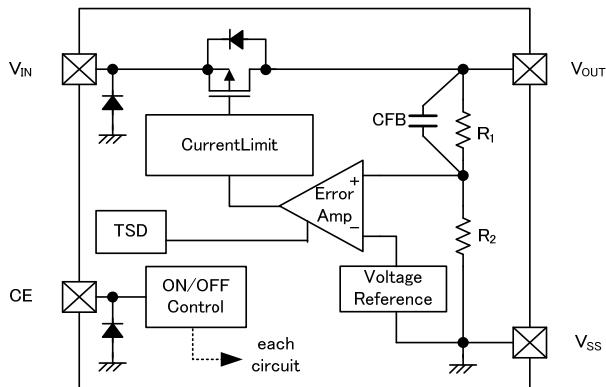
XC6223A/J series
