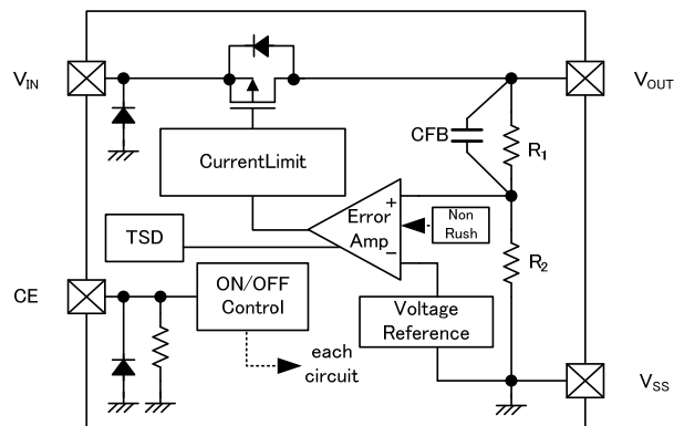
XC6223G/R series
