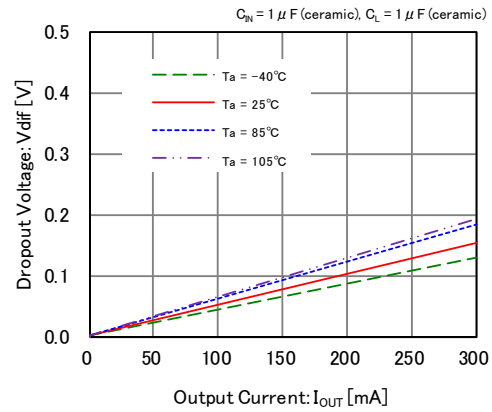
XC6223x401
