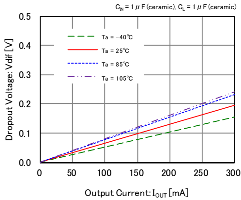
XC6223x251
