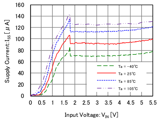
XC6223x181
