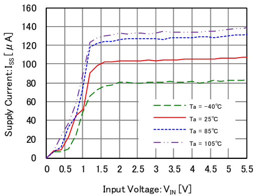
XC6223x121
