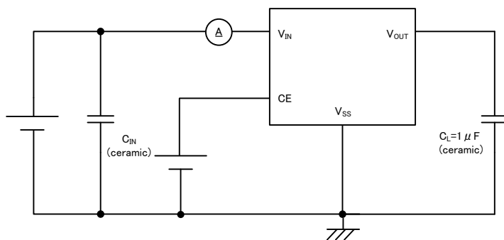
● Circuit ⑤
