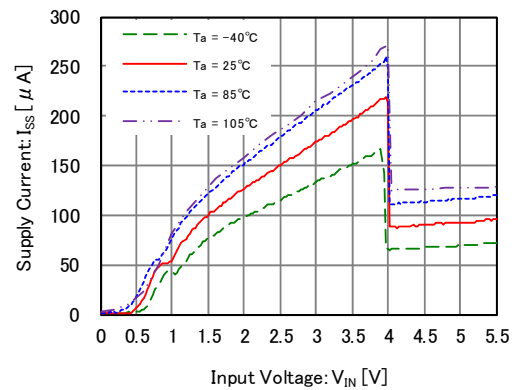
XC6223x401
