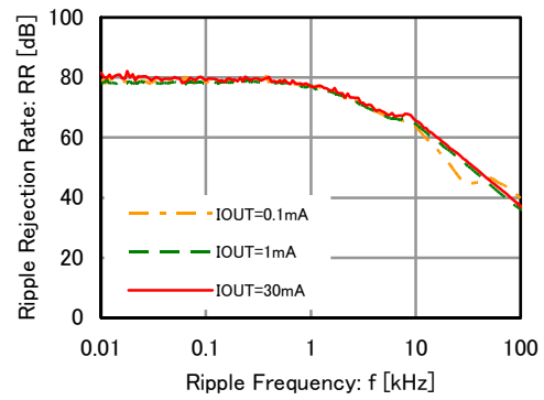
XC6223x181
