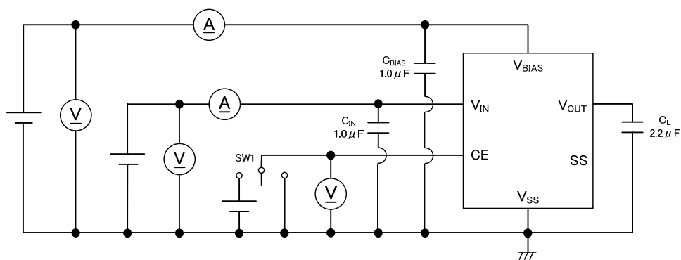
CIRCUIT②
