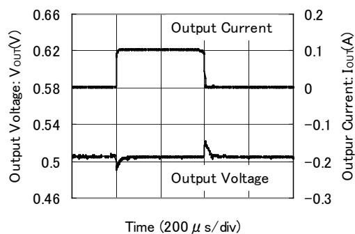
XC6603A121xR-G
