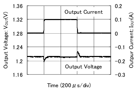
XC6603A181xR-G
