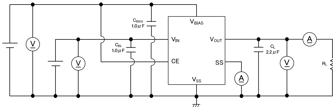
CIRCUIT⑤
