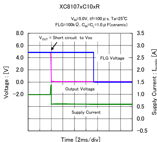
(29) Short-Circuit Transient Response ( V_{OUT}=\text{open} \rightarrow \text{short} , C_L=1.0\mu\text{F} )
