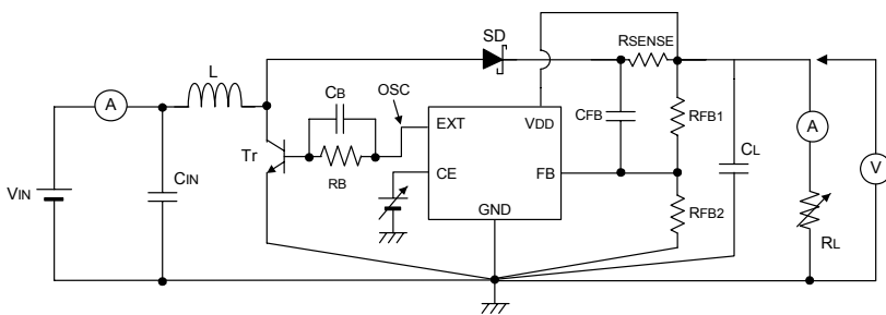
Circuit ③
