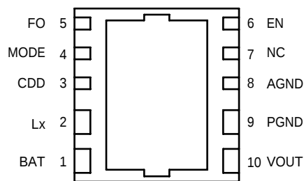
USP-10B ( BOTTOM VIEW ) XC9136 Series
