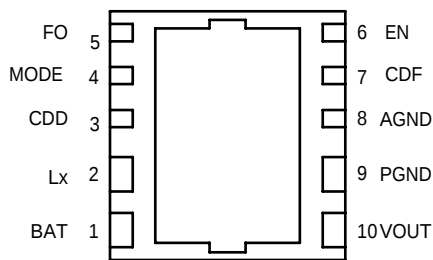
USP-10B ( BOTTOM VIEW ) XC9135 Series
