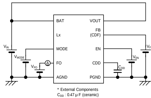
<Circuit No.7 >
