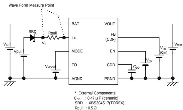
<Circuit No.9 >
