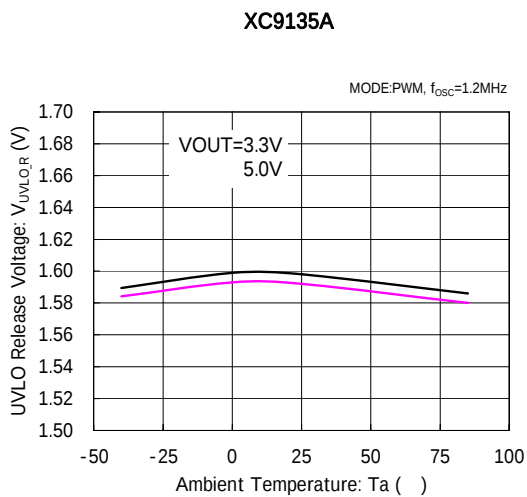
(22) UVLO Release Voltage vs. Ambient Temperature
