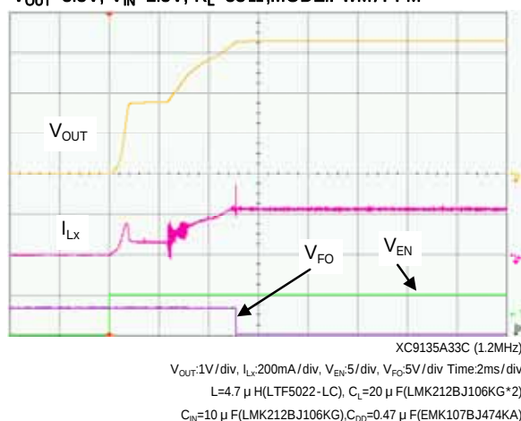
V_{OUT}=3.3V , V_{IN}=1.8V , R_L=33\Omega , MODE:PWM/PFM
