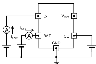
< Circuit No.⑦ >
