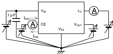
< Circuit No.5 >
