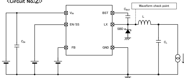
<Circuit No.②>
