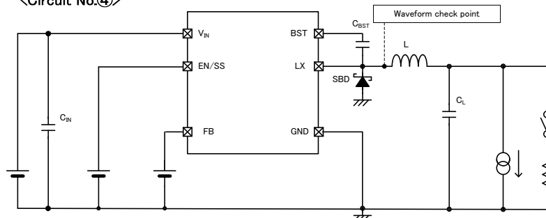
<Circuit No.④>
