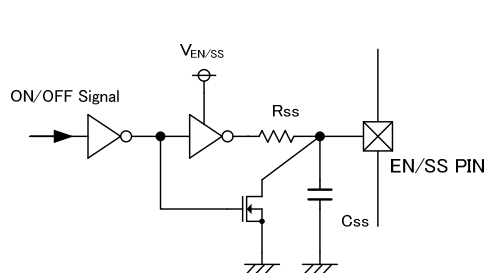
> Circuit Example3 : CMOS logic (low current dissipation, quick off)
