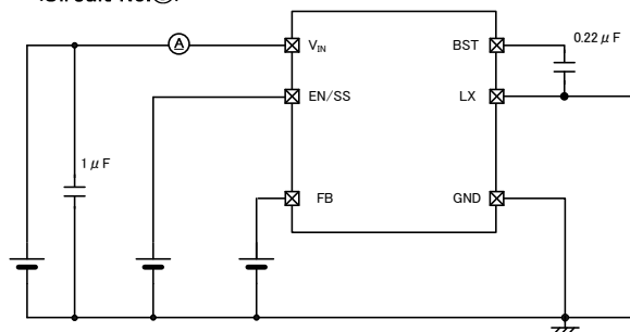
<Circuit No.③>
