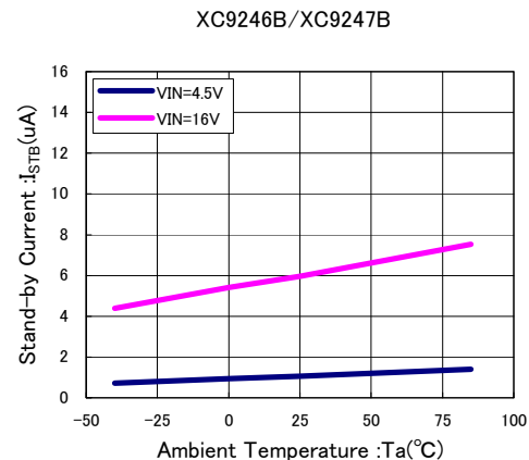
(8) Stand-by Current vs. Ambient Temperature
