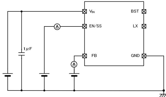
<Circuit No.⑥>
