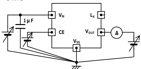
< Circuit No.⑦ >
