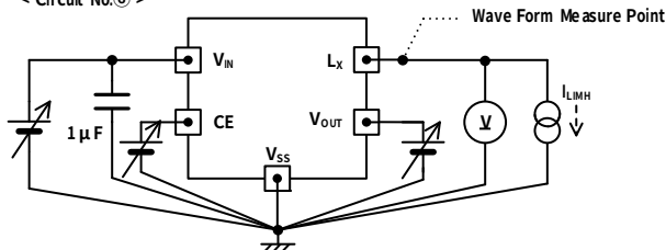
< Circuit No.⑥ >
