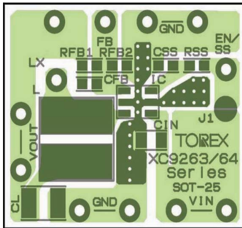
SOT-25 (Front)
