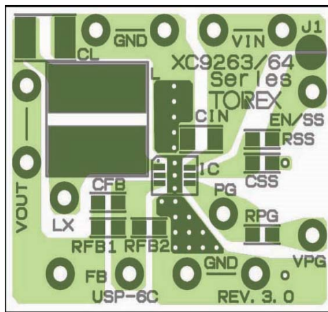
USP-6C (Front)
