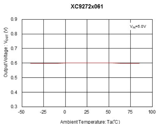
(4) Output Voltage vs. Ambient Temperature
