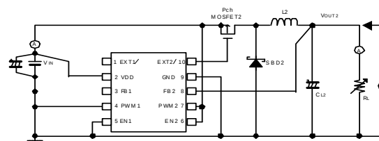
Circuit
