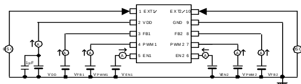
Circuit
