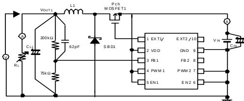
Circuit
