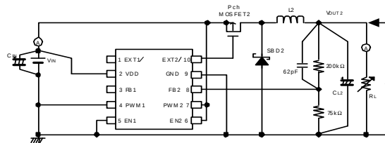
Circuit
