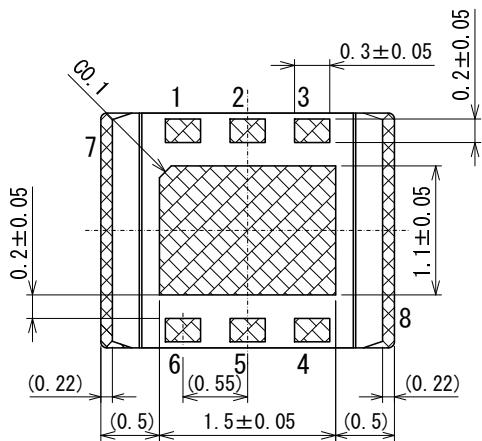
●Reference Pattern Layout (unit:mm)
