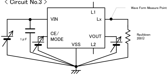
< Circuit No.3 >
