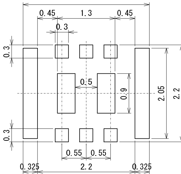
●Reference Metal Mask Design (unit:mm)
