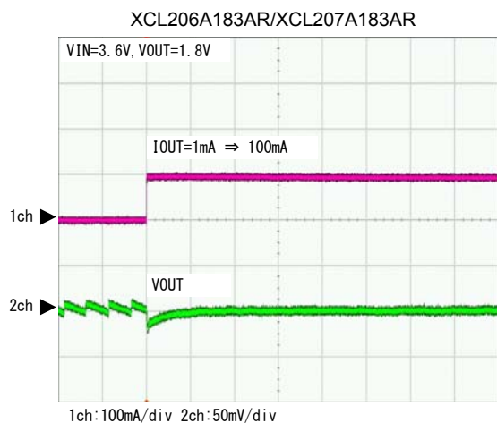
(15) Load Transient Response 1
