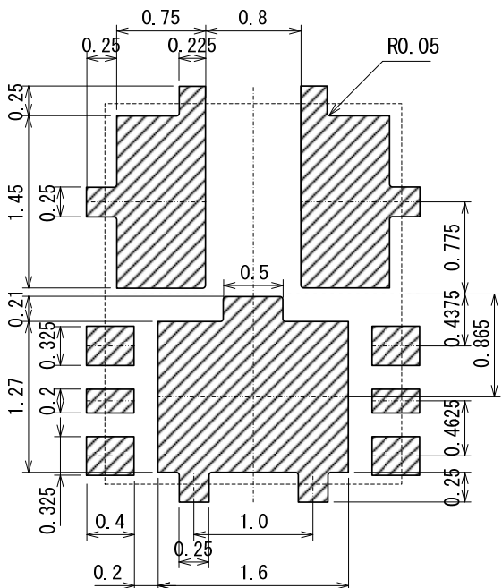
●USP-9B01 Reference Pattern Layout (unit: mm)
