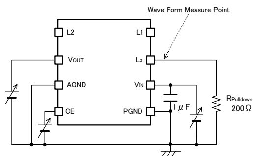
< Circuit No.⑤ >
