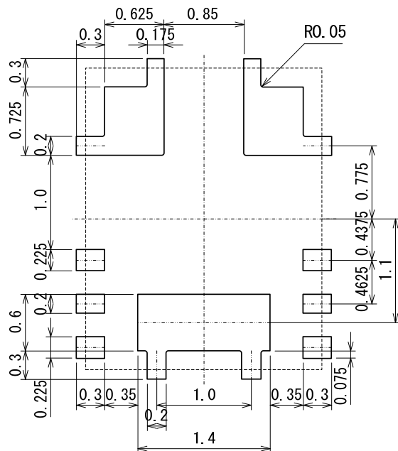
●USP-9B01 Reference Metal Mask Design (unit: mm)
