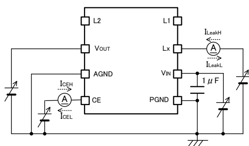
< Circuit No.⑦ >
