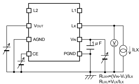
< Circuit No.⑥ >
