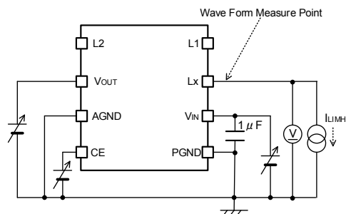
< Circuit No.⑥ >
