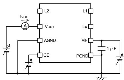
< Circuit No.⑦ >
