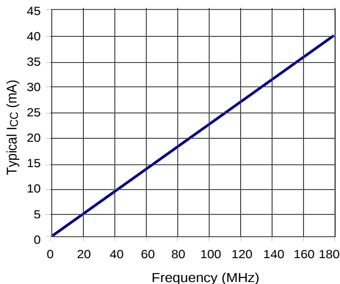
Figure 1: I_{CC} vs. Frequency at V_{CC} = 3.3V , 25^{\circ}C
