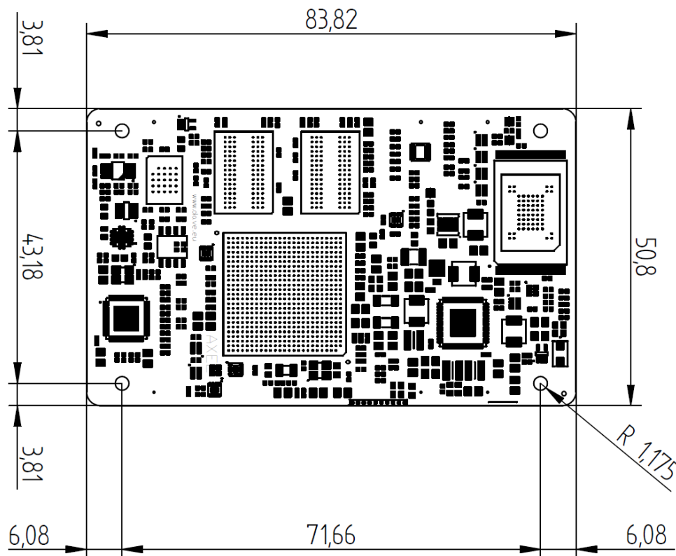
Fig. 4: Board layout - Top view
