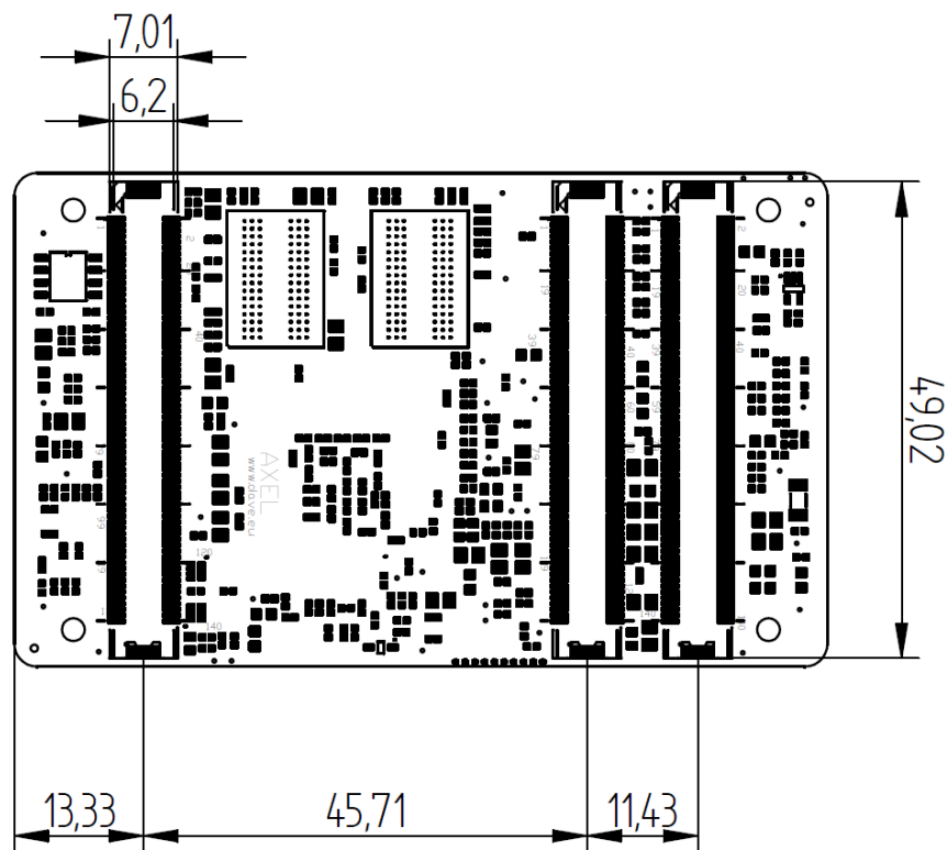
Fig. 6: Connectors layout
