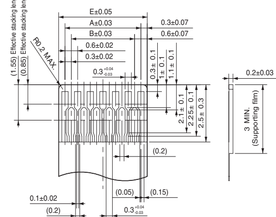
Recommended FPC Dimensions
