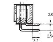
Right-angle DIP terminals
