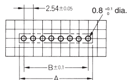
Mounting holes (bottom view)
