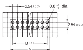
Mounting view (bottom view)
