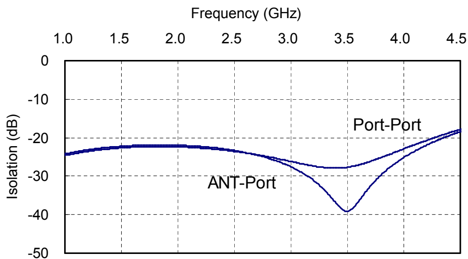
Fig.9 Isolation vs. Frequency
