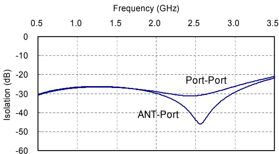
Fig.6 Isolation vs. Frequency
