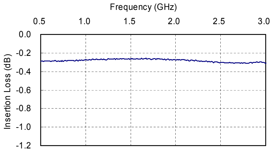
Fig.1 Insertion Loss vs. Frequency
