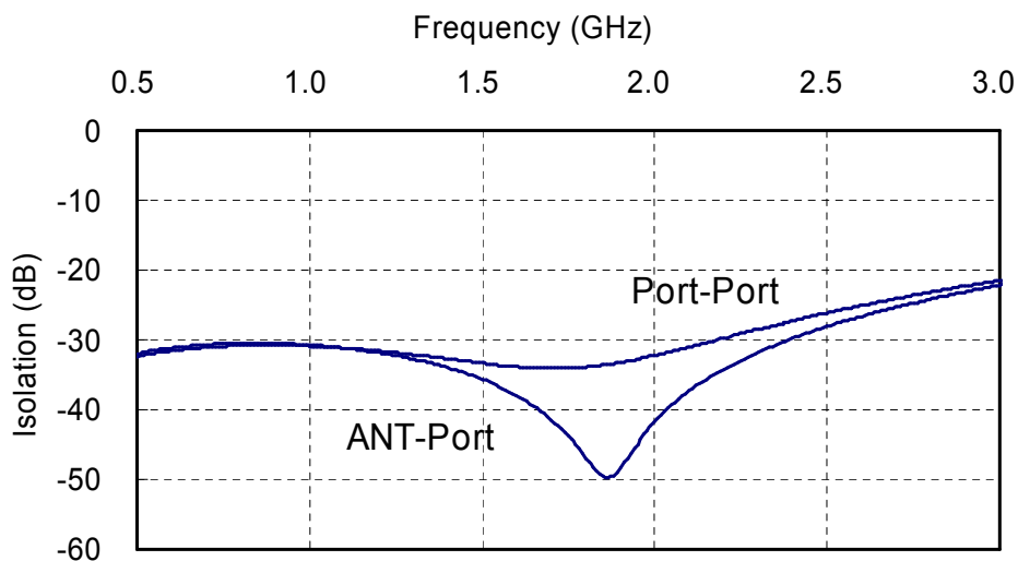
Fig.2 Isolation vs. Frequency
