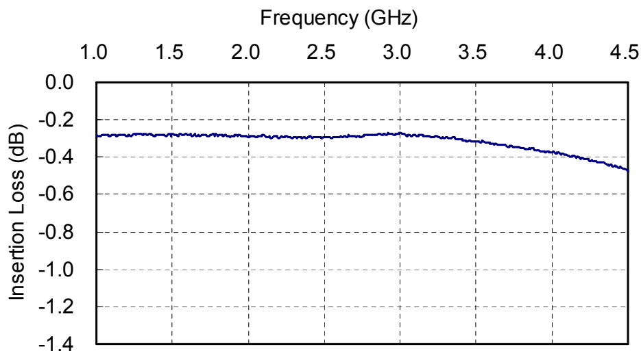
Fig.8 Insertion Loss vs. Frequency
