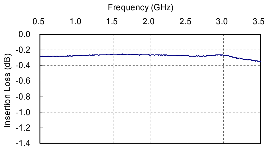
Fig.5 Insertion Loss vs. Frequency
