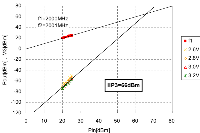
Fig.4 Input IIP3 (f=2.0GHz)
