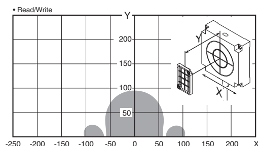
V680-HS63 (mounted on non-metallic material) & V680-D8KF67 (mounted on non-metallic material)
