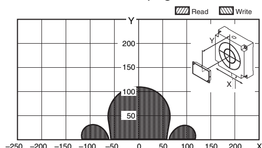
V680-HS65 (mounted on metallic material) & V680-D8KF68/-D32KF68 (Tag direction: Horizontal)
