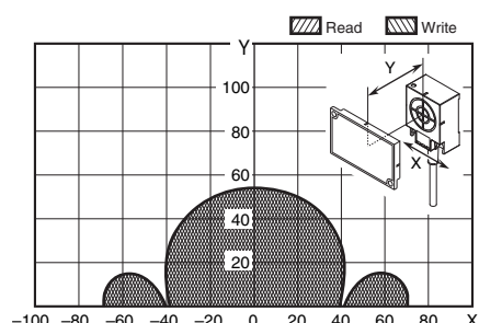
V680-HS65 (mounted on metallic material) & V680-D8KF68/-D32KF68 (Tag direction: Horizontal)
