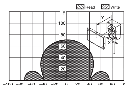
V680-HS63 (mounted on metallic material) & V680-D8KF68/-D32KF68 (mounted on metallic surface: steel) (Tag direction: Horizontal) When the V680-A81 attachment is mounted on RF Tag
