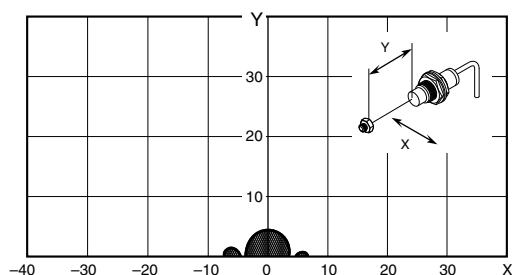
V680-HS51 (embedded in metallic material) & V680-D2KF52M-BT01 (mounted in metal/non-metallic material) V680-HS51 (embedded in metallic material) & V680-D2KF52M-BT11 (mounted in metal/non-metallic material)
