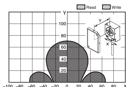
V680-HS63 (mounted on metallic material) & V680-D8KF68/-D32KF68 (mounted on metallic surface: steel) (Tag direction: Vertical) When the V680-A81 attachment is mounted on RF Tag
