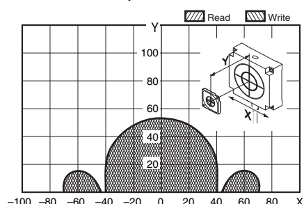
V680-HS63 (mounted on metallic material) & V680-D8KF68/-D32KF68 (mounted on non-metallic material) (Tag direction: Horizontal)
