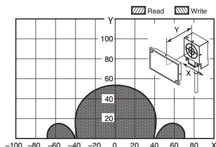
V680-HS65 (mounted on metallic material) & V680-D8KF68/-D32KF68 (mounted on non-metallic material) (Tag direction: Horizontal)
