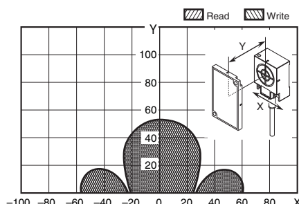
V680-HS65 (mounted on metallic material) & V680-D8KF68/-D32KF68 (mounted on non-metallic material) (Tag direction: Vertical)
