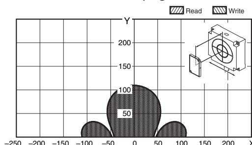
V680-HS65 (mounted on metallic material) & V680-D8KF68/-D32KF68 (Tag direction: Vertical)
