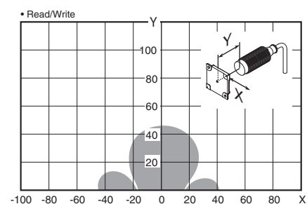
V680-HS52 (embedded on non-metallic material) & V680S-D8KF67
