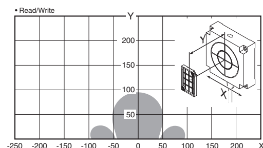
V680-HS63 (mounted on metallic material) & V680-D8KF68/-D32KF68 (mounted on non-metallic material) (Tag direction: Vertical)
