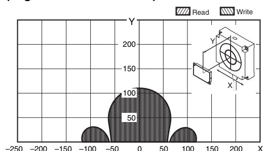
V680-HS65 (mounted on metallic material) & V680-D8KF68/-D32KF68 (mounted on non-metallic material) (Tag direction: Horizontal)
