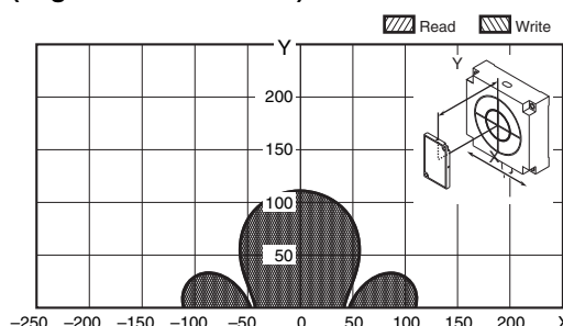
V680-HS65 (mounted on metallic material) & V680-D8KF68/-D32KF68 (mounted on non-metallic material) (Tag direction: Vertical)
