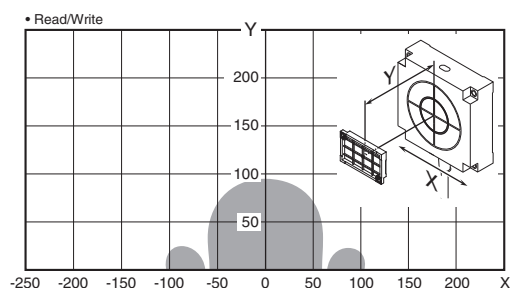
V680-HS52 (embedded in non-metallic material) & V680-D8KF67 (mounted on non-metallic material)
