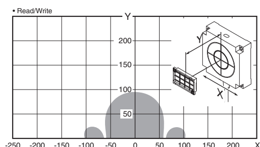
V680-HS63 (mounted on metallic material) & V680-D8KF68/-D32KF68 (mounted on non-metallic material) (Tag direction: Horizontal)
