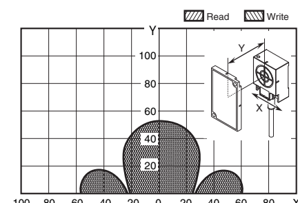
V680-HS65 (mounted on metallic material) & V680-D8KF68/-D32KF68 (Tag direction: Vertical)
