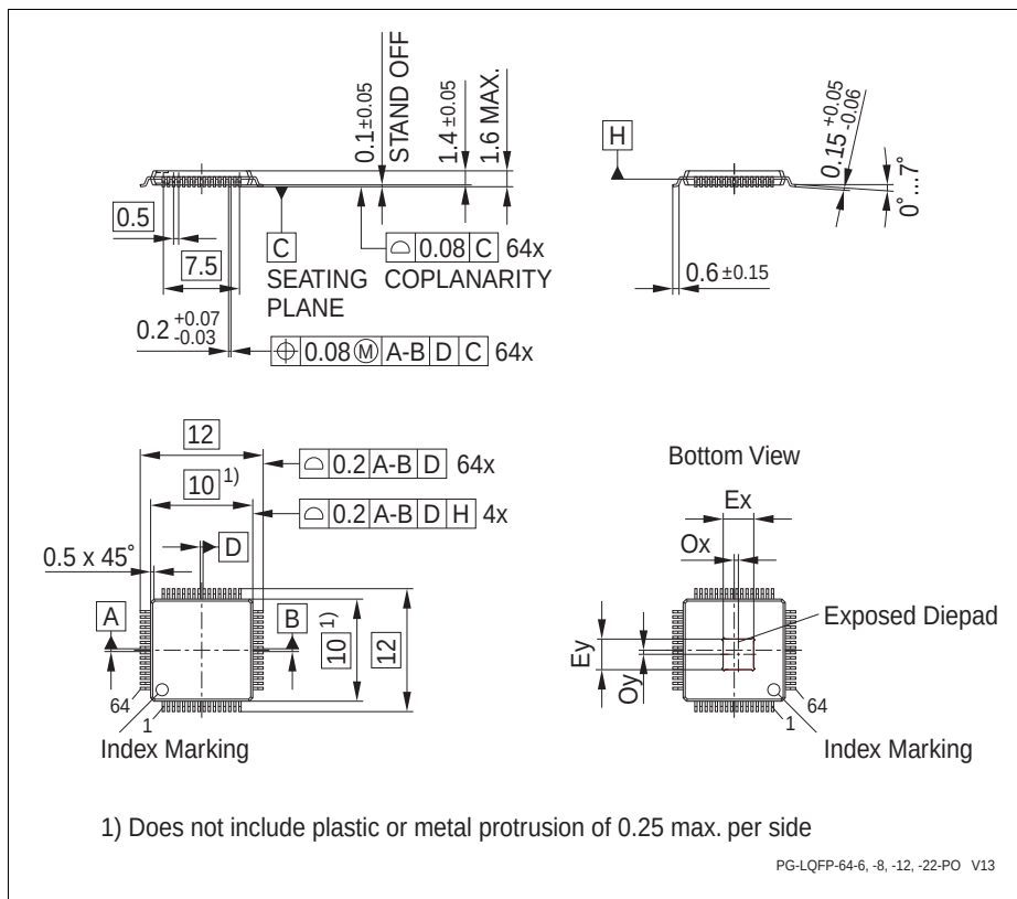
Figure 43 PG-LQFP-64-19 (Plastic Green Low Profile Quad Flat Package)
