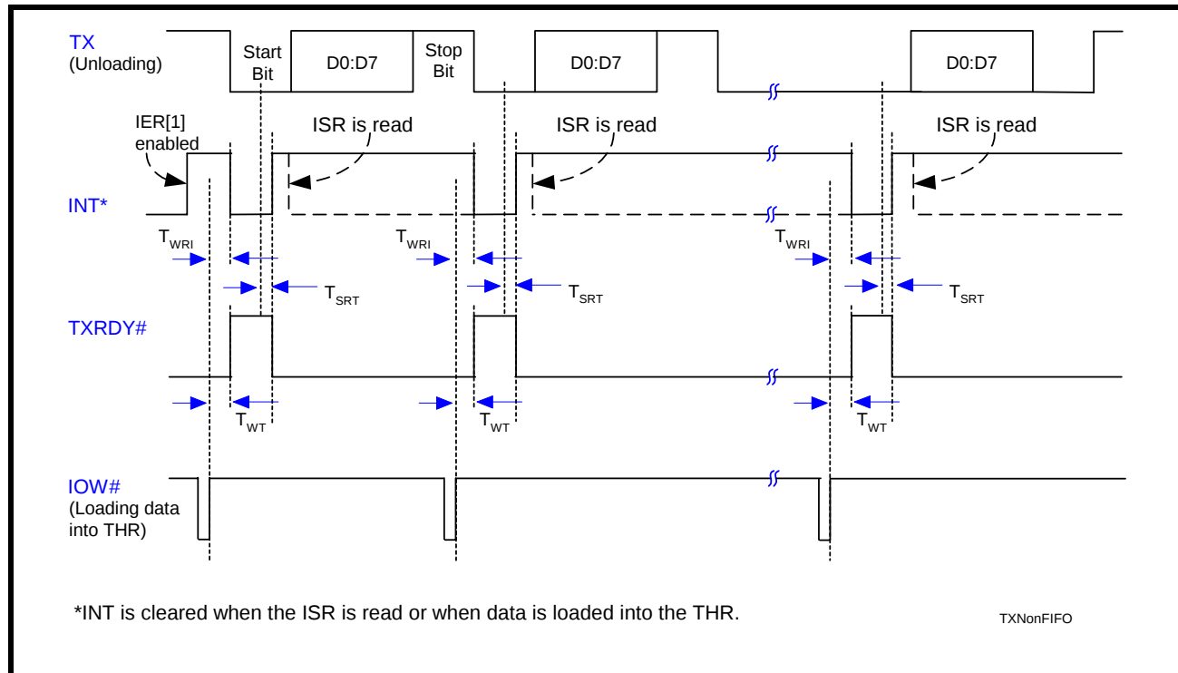
FIGURE 23. TRANSMIT READY &amp; INTERRUPT TIMING [NON-FIFO MODE]
