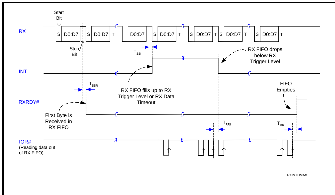
FIGURE 24. RECEIVE READY &amp; INTERRUPT TIMING [FIFO MODE]
