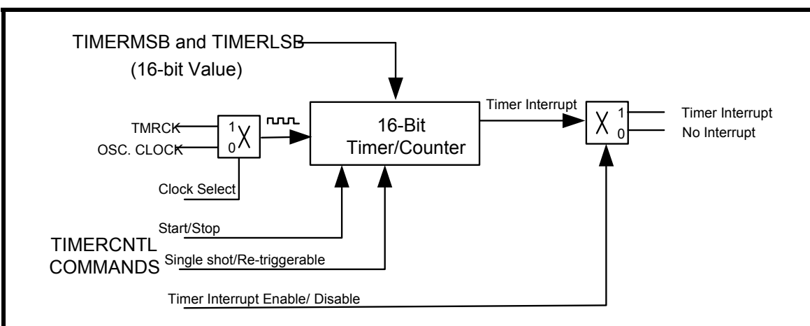
FIGURE 14. TIMER/COUNTER CIRCUIT
