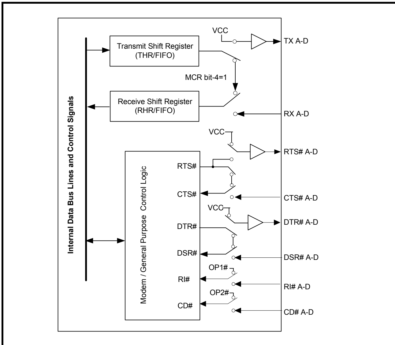
FIGURE 11. INTERNAL LOOPBACK
