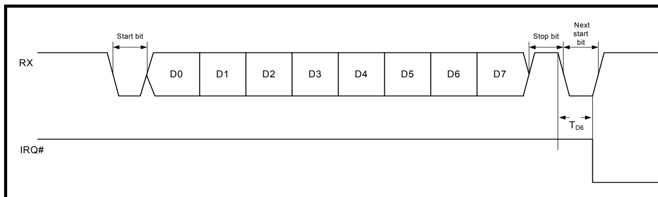
FIGURE 21. RECEIVE INTERRUPT
