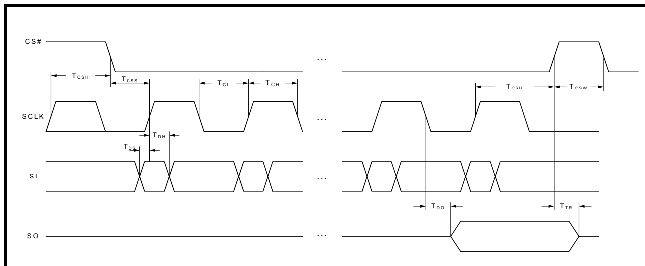
FIGURE 24. SPI-BUS TIMING
