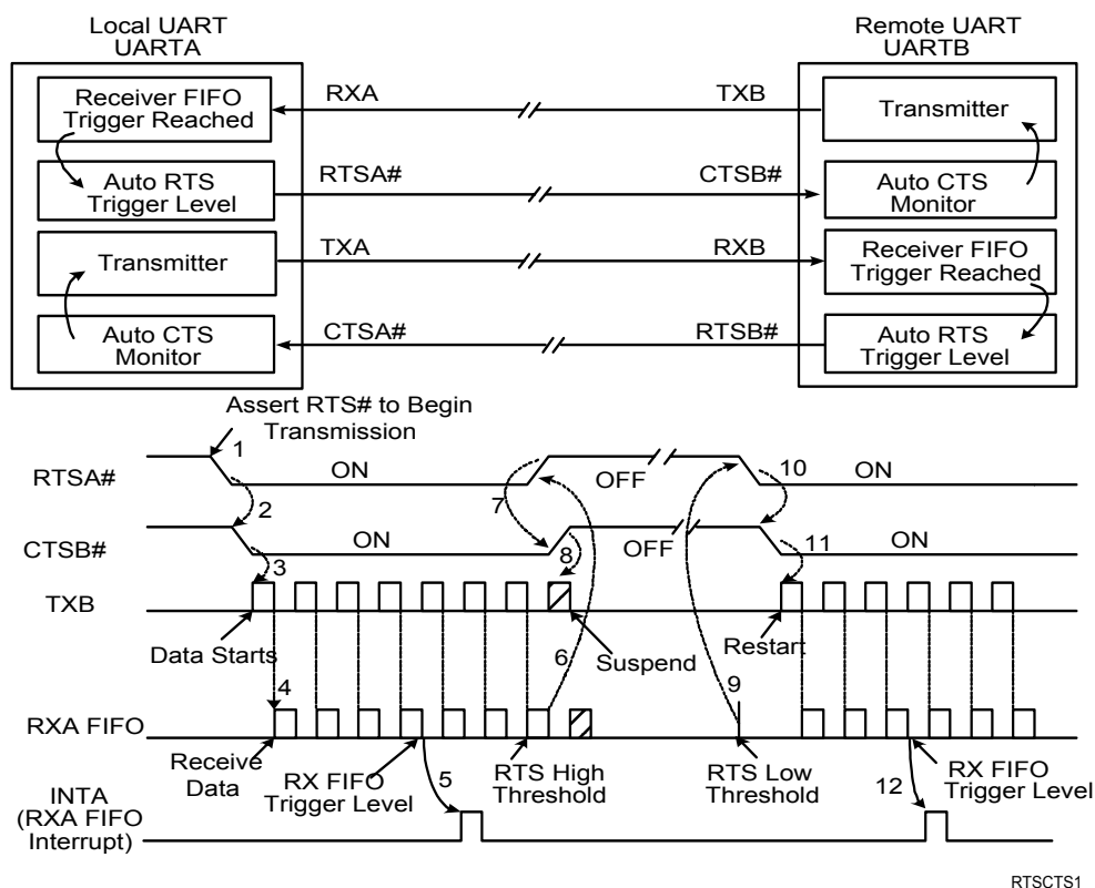
FIGURE 12. AUTO RTS AND CTS FLOW CONTROL OPERATION
