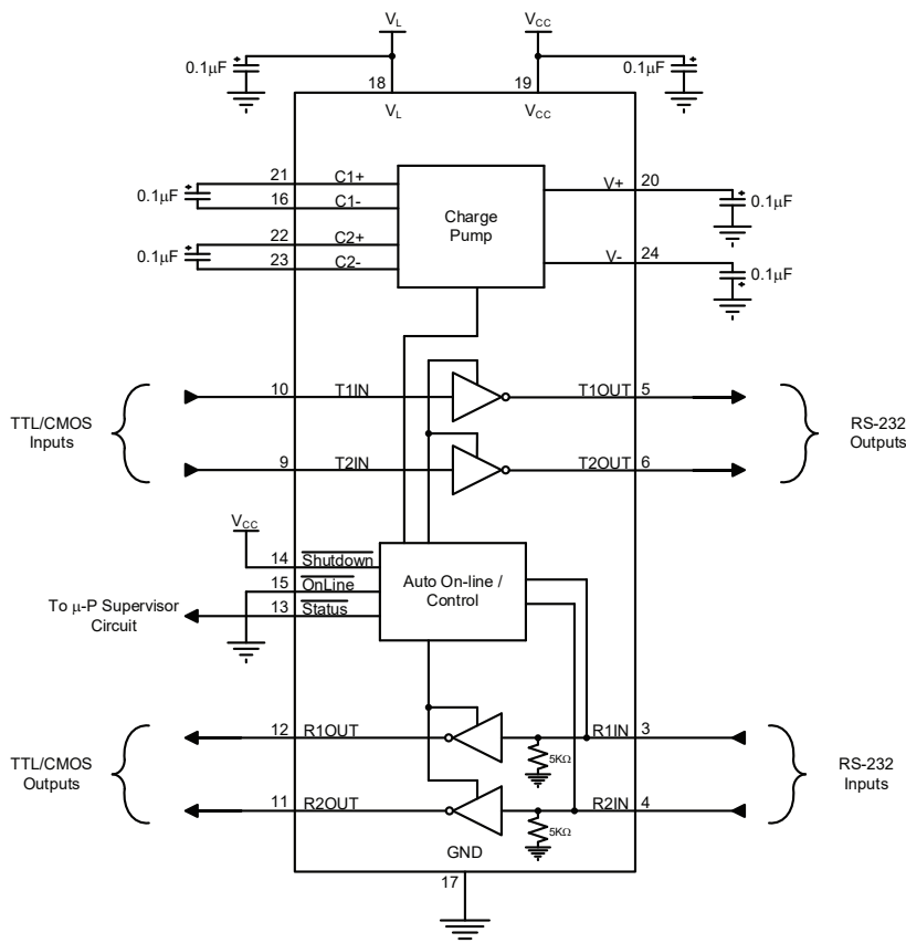
Figure 1. Typical Application
