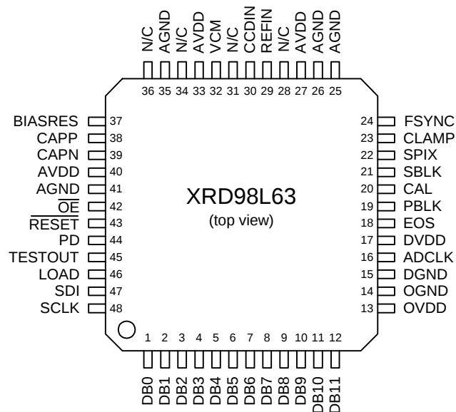
Figure 2. XRD98L63 Pinout
