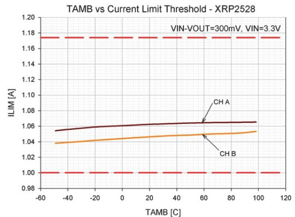
Fig. 21: Current Limit Threshold vs. Temperature (XRP2528)
