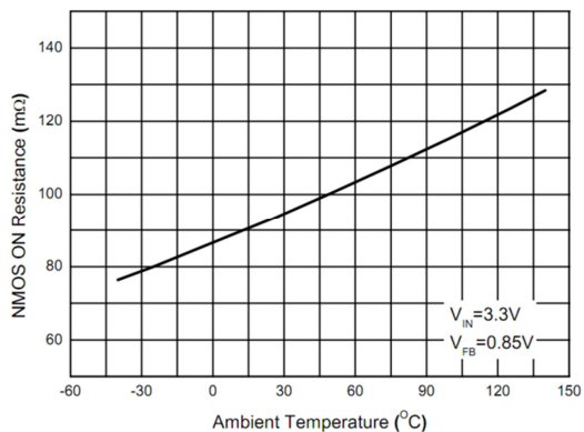
Fig. 8: NMOS R_{DS(on)} Resistance versus Ambient Temperature
