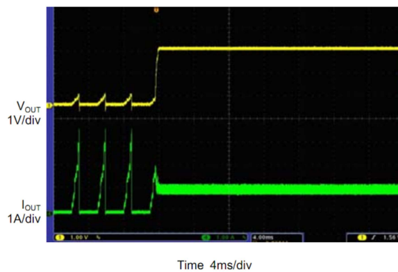
Fig. 15: Short Circuit Recovery V_{IN}=3.3V , V_{OUT}=2.5V
