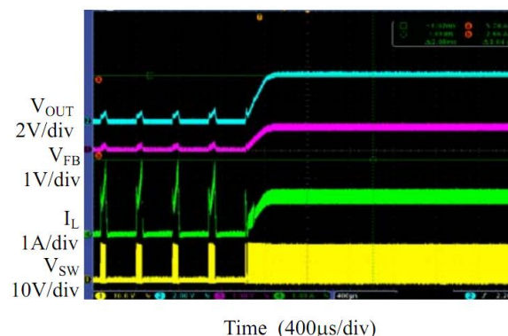
Fig. 15: Short-circuit recovery R_{LOAD}=2.6\Omega
