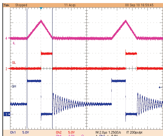
Figure 15 PFM Zero Current Accuracy
