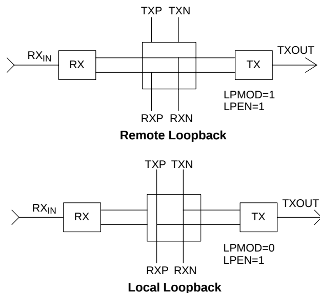
Figure 5. Loopback Configurations
