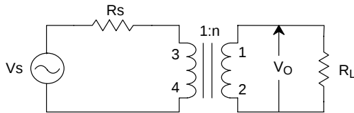
Figure 6. Equivalent Impedance Schematic
