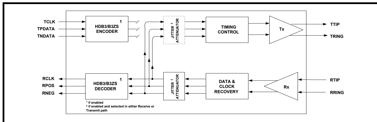
FIGURE 27. REMOTE LOOPBACK
