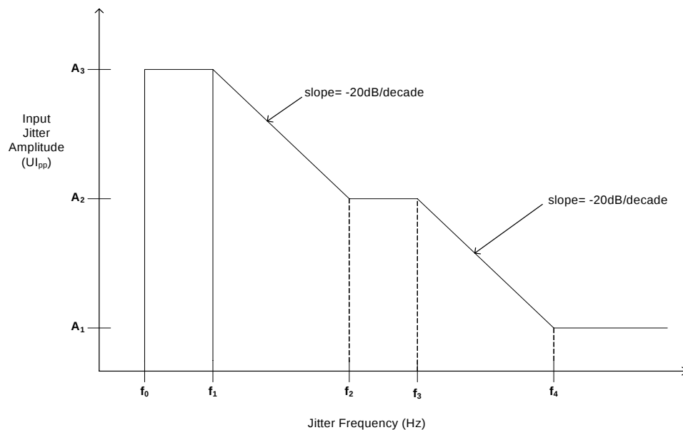
FIGURE 5. GR-253/G.783 JITTER TOLERANCE MASK
