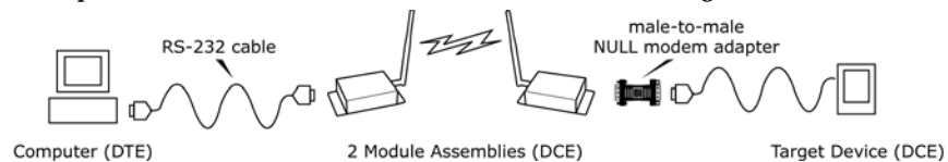
Figure B-02. Example of a MaxStream Radio Modem (DCE Device) connecting to another DCE device
