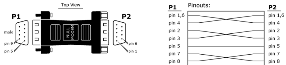
Figure B-02. Example of a MaxStream Radio Modem (DCE Device) connecting to another DCE device
