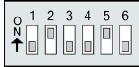
Figure 2-12. RS-485 (2-wire) w/ Termination (optional)
