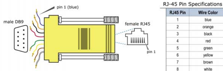
Figure B-05. Male DB-9 to RJ-45 Adapter and pinouts
