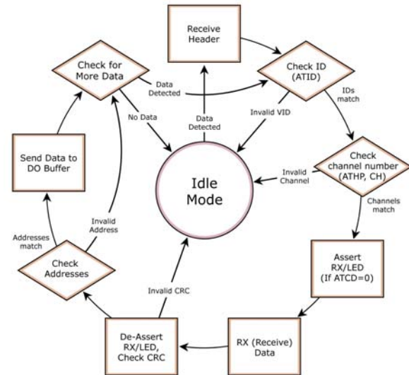
Figure 3-06. Receive Mode Data Flow
