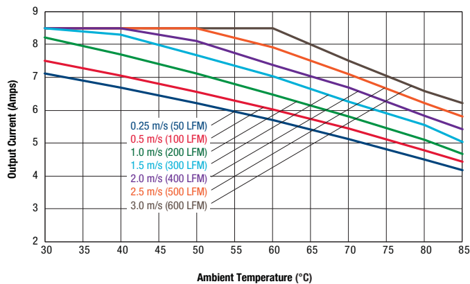
Maximum Current Temperature Derating at sea level ( V_{in}=48V , transverse airflow, on 10'' \times 10'' PCB with baseplate)
