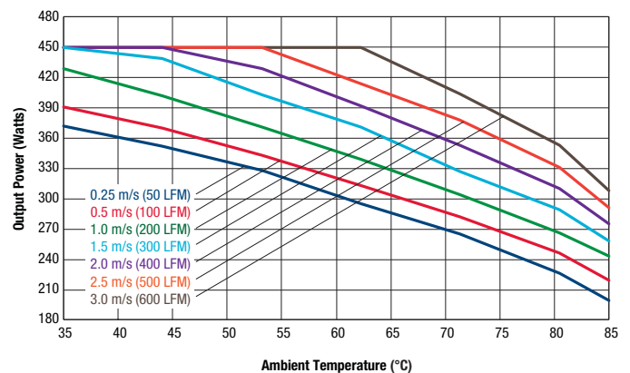
Maximum Power Temperature Derating at sea level ( V_{in}=48V , longitudinal airflow, on 10'' \times 10'' PCB with baseplate)
