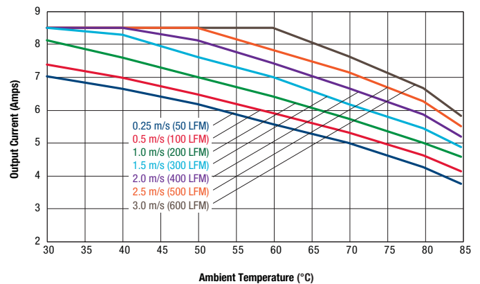
Maximum Current Temperature Derating at sea level ( V_{in}=48V , longitudinal airflow, on 10'' \times 10'' PCB with baseplate)
