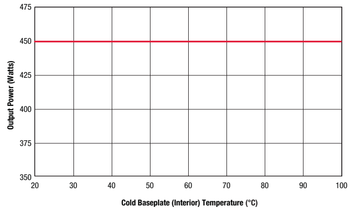
Output Power Derating in Conduction Cooling (Cold Baseplate) Applications ( V_{in}=48V , Ambient Temperature <70^{\circ}C )
