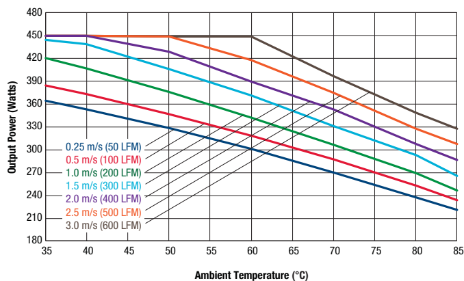
Maximum Power Temperature Derating at sea level ( V_{in}=48V , transverse airflow, on 10'' \times 10'' PCB with baseplate)
