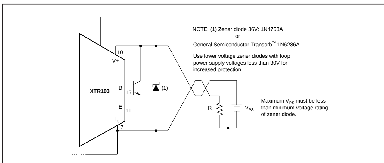
FIGURE 6. Over-Voltage Surge Protection.
