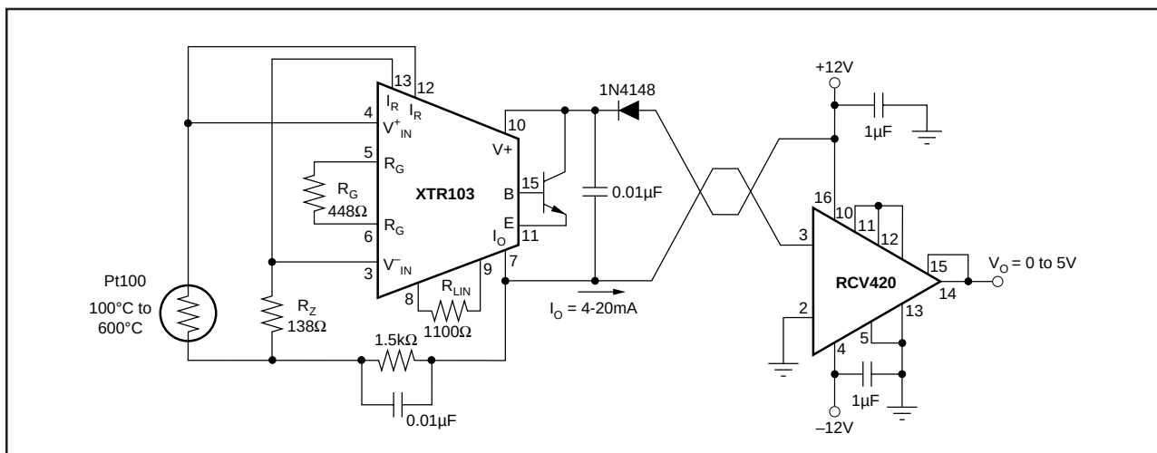
FIGURE 8. ±12V-Powered Transmitter/Receiver Loop.
