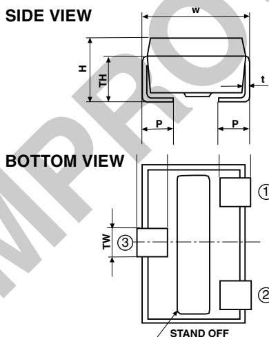
FIGURE 6 - DIMENSIONS AND IMPRINTING
