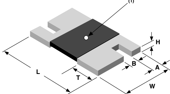
FIGURE 2 - DIMENSIONS AND IMPRINTING in inches (millimeters)
