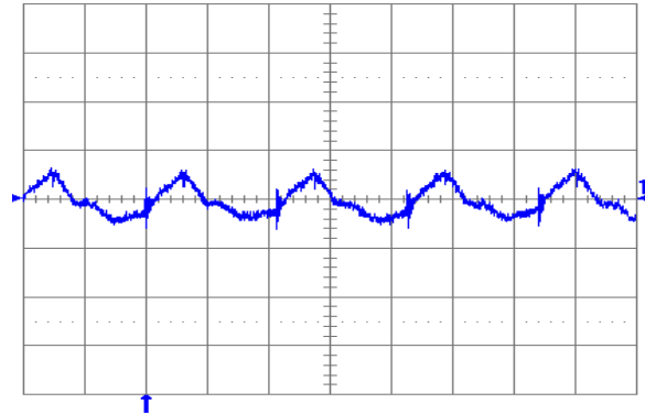
Fig. 3.3V.6: Output voltage ripple (20 mV/div.) at full rated load current into a resistive load with external capacitance 47 \mu F ceramic + 1 \mu F ceramic, and V_{in} = 12 V for V_{out} = 3.3 V. Time scale: 1 \mu s/div.
