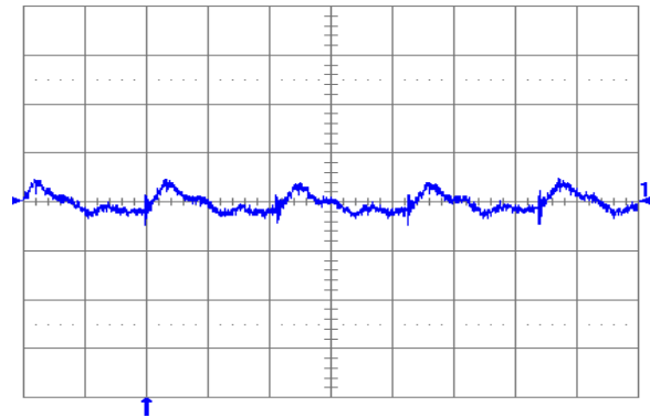
Fig. 1.8V.6: Output voltage ripple (20 mV/div.) at full rated load current into a resistive load with external capacitance 47 \mu F ceramic + 1 \mu F ceramic, and V_{in} = 12 V for V_{out} = 1.8 V. Time scale: 1 \mu s/div.
