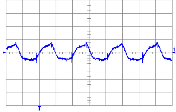
Fig. 5.0V.6: Output voltage ripple (20 mV/div.) at full rated load current into a resistive load with external capacitance 47 \mu F ceramic + 1 \mu F ceramic, and V_{in} = 12 V for V_{out} = 5.0 V. Time scale: 1 \mu s/div.
