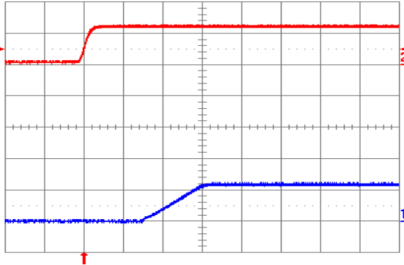
Fig. 1.2V.5: Turn-on transient for V_{out} = 1.2 V with application of V_{in} at full rated load current (resistive) and 47 \mu F external capacitance at V_{in} = 12 V. Top trace: V_{in} (10 V/div.); Bottom trace: output voltage (1 V/div.); Time scale: 5 ms/div.
