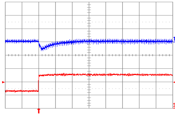
Fig. 1.8V.7: Output voltage response for V_{out} = 1.8 V to positive load current step change from 2.5 A to 5 A with slew rate of 5 A/ \mu s at V_{in} = 12 V. Top trace: output voltage (100 mV/div.); Bottom trace: load current (2 A/div.). C_o = 47 \mu F ceramic. Time scale: 20 \mu s/div.
