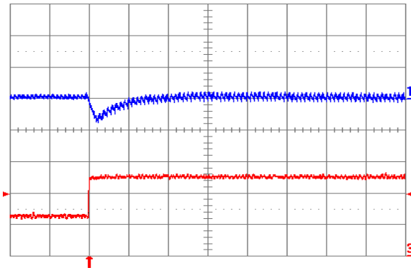
Fig. 3.3V.7: Output voltage response for V_{out} = 3.3 V to positive load current step change from 2.5 A to 5 A with slew rate of 5 A/ \mu s at V_{in} = 12 V. Top trace: output voltage (100 mV/div.); Bottom trace: load current (2 A/div.). C_o = 47 \mu F ceramic. Time scale: 20 \mu s/div.
