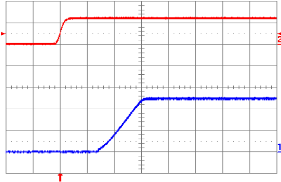
Fig. 2.5V.5: Turn-on transient for V_{out} = 2.5 V with application of V_{in} at full rated load current (resistive) and 47 \mu F external capacitance at V_{in} = 12 V. Top trace: V_{in} (10 V/div.); Bottom trace: output voltage (1 V/div.); Time scale: 5 ms/div.
