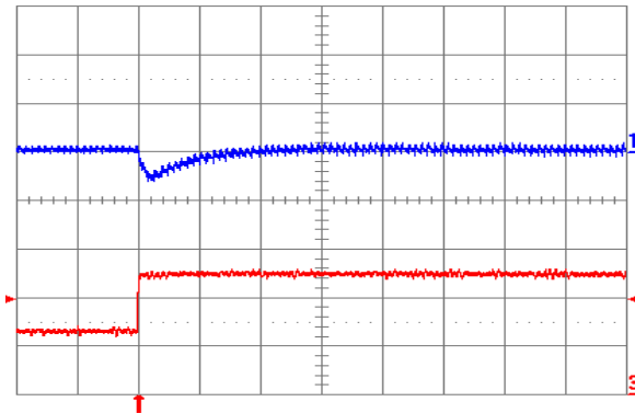
Fig. 2.0V.7: Output voltage response for V_{out} = 2.0 V to positive load current step change from 2.5 A to 5 A with slew rate of 5\text{ A}/\mu\text{s} at V_{in} = 12 V. Top trace: output voltage (100 mV/div.); Bottom trace: load current (2 A/div.). C_o = 47\text{ }\mu\text{F} ceramic. Time scale: 20 \mu\text{s} /div.
