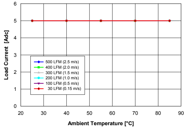
Fig. 1.8V.1: Available load current vs. ambient temperature and airflow rates for V_{out} = 1.8 V converter mounted vertically with V_{in} = 12 V, and maximum MOSFET temperature \leq 120 °C.
