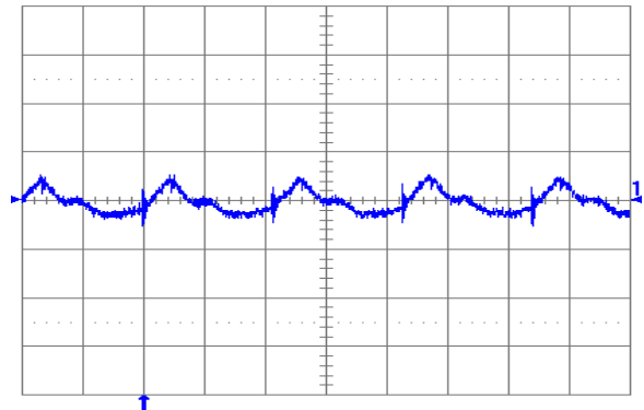
Fig. 2.5V.6: Output voltage ripple (20 mV/div.) at full rated load current into a resistive load with external capacitance 47 \mu F ceramic + 1 \mu F ceramic, and V_{in} = 12 V for V_{out} = 2.5 V. Time scale: 1 \mu s/div.
