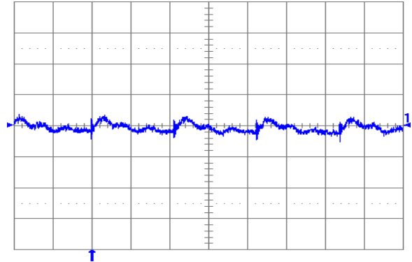
Fig. 1.2V.6: Output voltage ripple (20 mV/div.) at full rated load current into a resistive load with external capacitance 47 \mu F ceramic + 1 \mu F ceramic, and V_{in} = 12 V for V_{out} = 1.2 V. Time scale: 1 \mu s/div.
