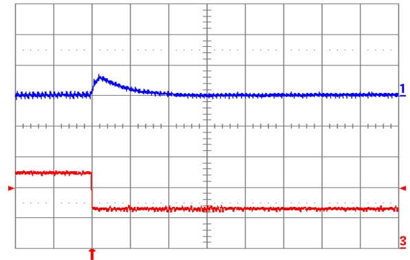
Fig. 2.0V.8: Output voltage response for V_{out} = 2.0 V to negative load current step change from 5 A to 2.5 A with slew rate of -5\text{ A}/\mu\text{s} at V_{in} = 12 V. Top trace: output voltage (100 mV/div.); Bottom trace: load current (2 A/div.). C_o = 47\text{ }\mu\text{F} ceramic. Time scale: 20 \mu\text{s} /div.
