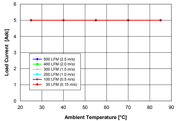
Fig. 2.5V.2: Available load current vs. ambient temperature and airflow rates for V_{out} = 2.5 V converter mounted horizontally with V_{in} = 12 V, and maximum MOSFET temperature \leq 120 °C.
