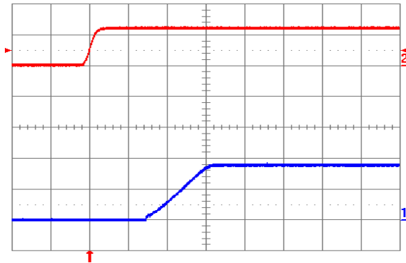
Fig. 1.8V.5: Turn-on transient for V_{out} = 1.8 V with application of V_{in} at full rated load current (resistive) and 47 \mu F external capacitance at V_{in} = 12 V. Top trace: V_{in} (10 V/div.); Bottom trace: output voltage (1 V/div.); Time scale: 5 ms/div.
