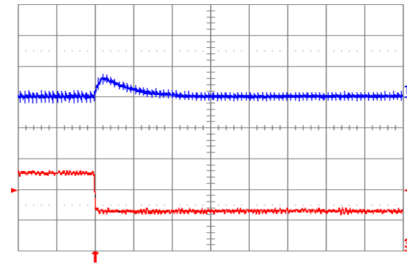
Fig. 1.8V.8: Output voltage response for V_{out} = 1.8 V to negative load current step change from 5 A to 2.5 A with slew rate of -5 A/ \mu s at V_{in} = 12 V. Top trace: output voltage (100 mV/div.); Bottom trace: load current (2 A/div.). C_o = 47 \mu F ceramic. Time scale: 20 \mu s/div.
