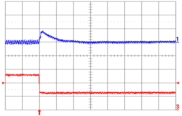
Fig. 5.0V.8: Output voltage response for V_{out} = 5.0 V to negative load current step change from 5 A to 2.5 A with slew rate of -5 A/ \mu s at V_{in} = 12 V. Top trace: output voltage (100 mV/div.); Bottom trace: load current (2 A/div.). C_o = 47 \mu F ceramic. Time scale: 20 \mu s/div.
