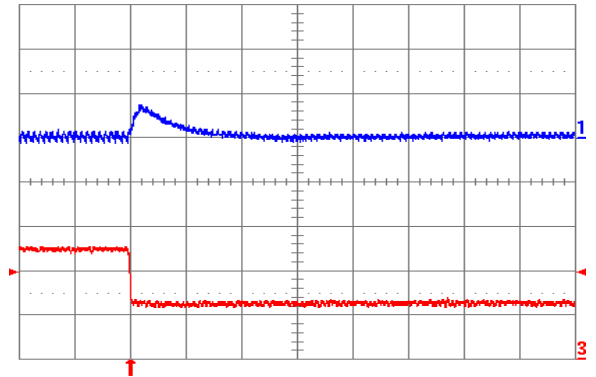
Fig. 3.3V.8: Output voltage response for V_{out} = 3.3 V to negative load current step change from 5 A to 2.5 A with slew rate of -5 A/ \mu s at V_{in} = 12 V. Top trace: output voltage (100 mV/div.); Bottom trace: load current (2 A/div.). C_o = 47 \mu F ceramic. Time scale: 20 \mu s/div.
