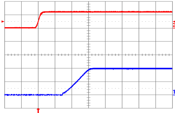
Fig. 2.0V.5: Turn-on transient for V_{out} = 2.0 V with application of V_{in} at full rated load current (resistive) and 47\text{ }\mu\text{F} external capacitance at V_{in} = 12 V. Top trace: V_{in} (10 V/div.); Bottom trace: output voltage (1 V/div.); Time scale: 5 ms/div.
