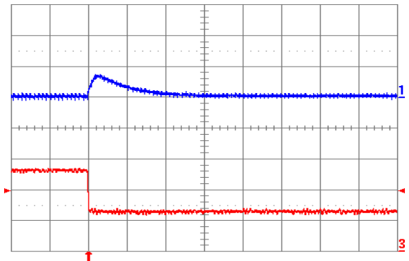
Fig. 1.2V.8: Output voltage response for V_{out} = 1.2 V to negative load current step change from 5 A to 2.5 A with slew rate of -5 A/ \mu s at V_{in} = 12 V. Top trace: output voltage (100 mV/div.); Bottom trace: load current (2 A/div.). C_o = 47 \mu F ceramic. Time scale: 20 \mu s/div.
