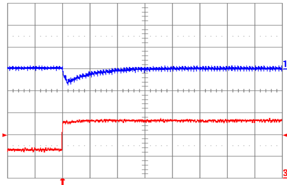
Fig. 1.2V.7: Output voltage response for V_{out} = 1.2 V to positive load current step change from 2.5 A to 5 A with slew rate of 5 A/ \mu s at V_{in} = 12 V. Top trace: output voltage (100 mV/div.); Bottom trace: load current (2 A/div.). C_o = 47 \mu F ceramic. Time scale: 20 \mu s/div.
