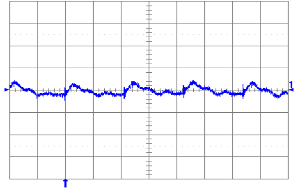
Fig. 1.5V.6: Output voltage ripple (20 mV/div.) at full rated load current into a resistive load with external capacitance 47 \mu F ceramic + 1 \mu F ceramic, and V_{in} = 12 V for V_{out} = 1.5 V. Time scale: 1 \mu s/div.
