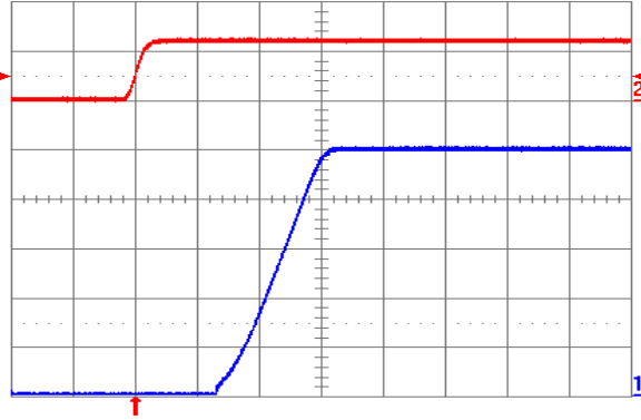
Fig. 5.0V.5: Turn-on transient for V_{out} = 5.0 V with application of V_{in} at full rated load current (resistive) and 47 \mu F external capacitance at V_{in} = 12 V. Top trace: V_{in} (10 V/div.); Bottom trace: output voltage (1 V/div.); Time scale: 5 ms/div.
