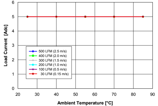
Fig. 2.0V.2: Available load current vs. ambient temperature and airflow rates for Vout = 2.0 V converter mounted horizontally with Vin = 12 V, and maximum MOSFET temperature ≤ 120 °C.
