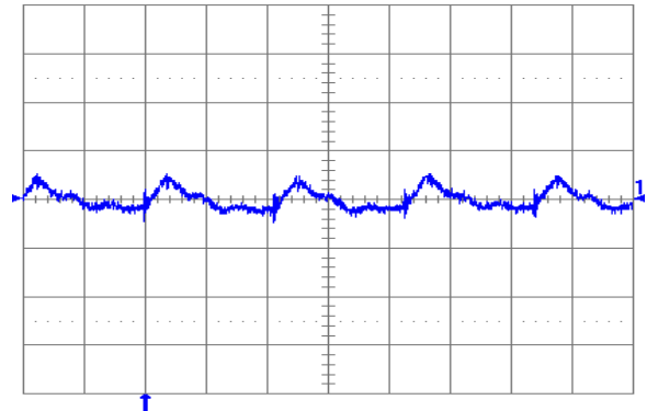
Fig. 2.0V.6: Output voltage ripple (20 mV/div.) at full rated load current into a resistive load with external capacitance 47\text{ }\mu\text{F} ceramic + 1\text{ }\mu\text{F} ceramic, and V_{in} = 12 V for V_{out} = 2.0 V. Time scale: 1 \mu\text{s} /div.
