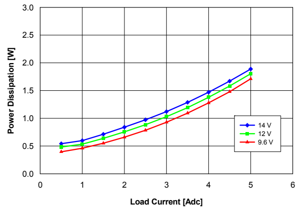
Fig. 1.8V.4: Power Loss vs. load current and input voltage for V_{out} = 1.8 V converter mounted vertically with air flowing at a rate of 200 LFM (1 m/s) and T_a = 25 °C.
