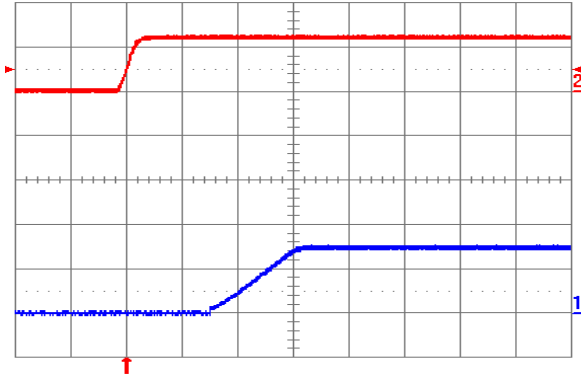
Fig. 1.5V.5: Turn-on transient for V_{out} = 1.5 V with application of V_{in} at full rated load current (resistive) and 47 \mu F external capacitance at V_{in} = 12 V. Top trace: V_{in} (10 V/div.); Bottom trace: output voltage (1 V/div.); Time scale: 5 ms/div.
