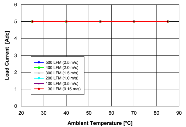
Fig. 3.3V.2: Available load current vs. ambient temperature and airflow rates for V_{out} = 3.3 V converter mounted horizontally with V_{in} = 12 V, and maximum MOSFET temperature \leq 120 °C.
