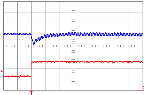
Fig. 5.0V.7: Output voltage response for V_{out} = 5.0 V to positive load current step change from 2.5 A to 5 A with slew rate of 5 A/ \mu s at V_{in} = 12 V. Top trace: output voltage (100 mV/div.); Bottom trace: load current (2 A/div.). C_o = 47 \mu F ceramic. Time scale: 20 \mu s/div.
