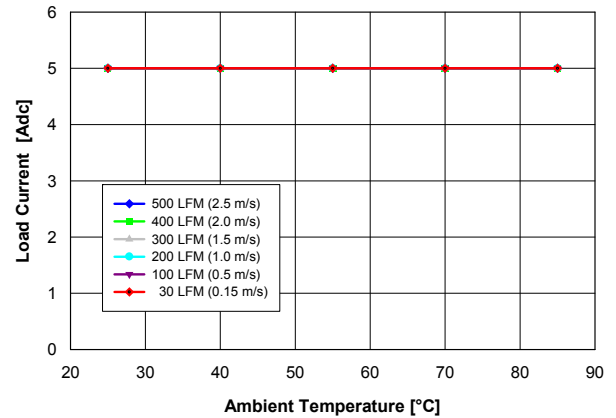
Fig. 1.8V.2: Available load current vs. ambient temperature and airflow rates for V_{out} = 1.8 V converter mounted horizontally with V_{in} = 12 V, and maximum MOSFET temperature \leq 120 °C.
