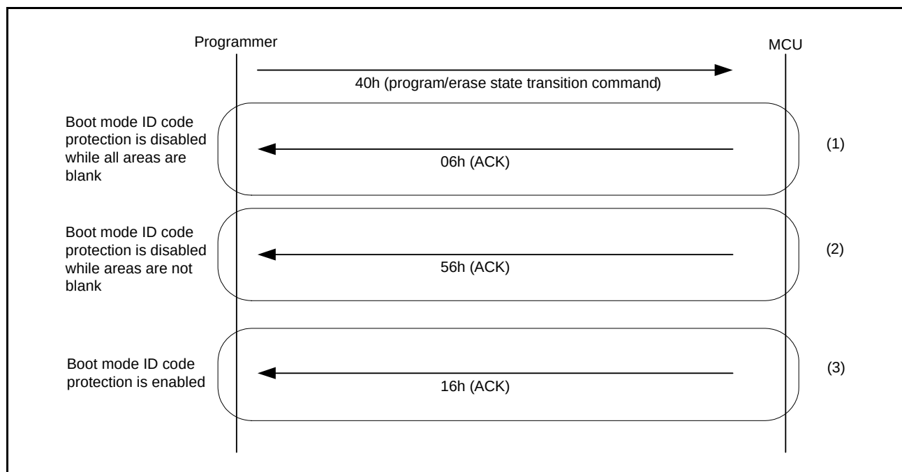
Figure 35.32 Procedure to Enter the Program/Erase State
