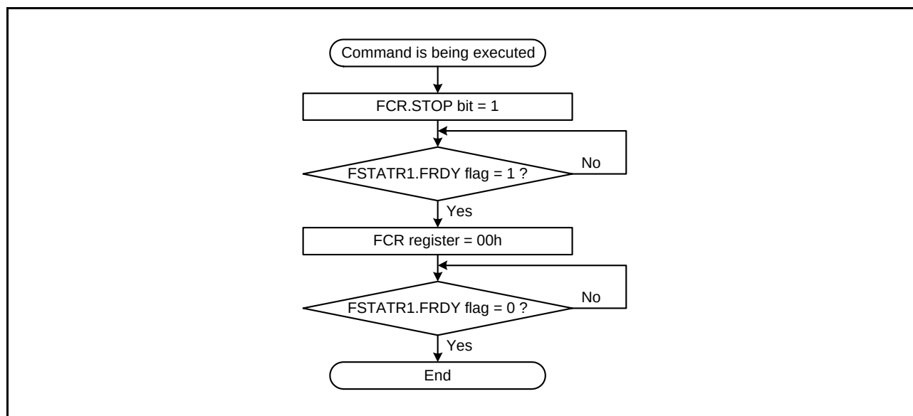
Figure 35.19 Procedure for Forced Stop of Software Commands
