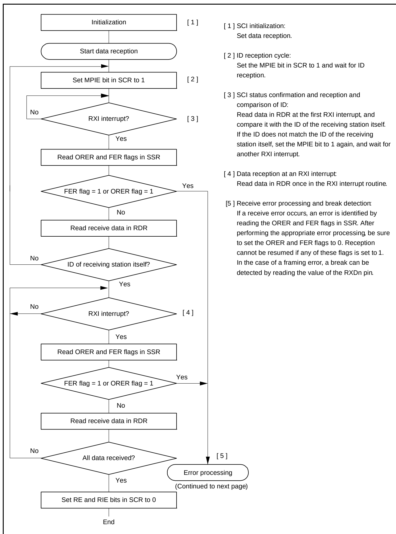
Figure 26.20 Example of Multi-Processor Serial Reception Flowchart (1)
