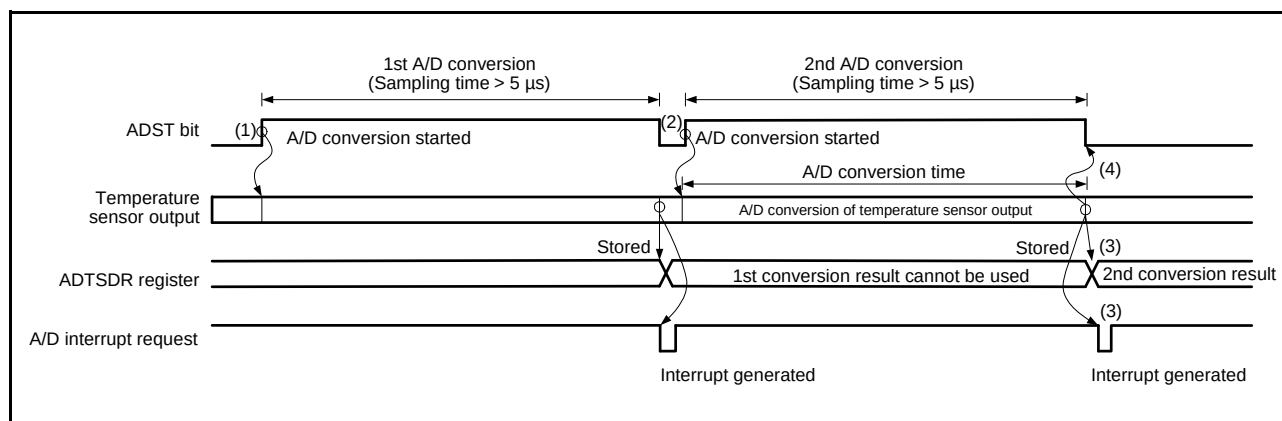
Figure 32.3 Example of Temperature Sensor Operation
