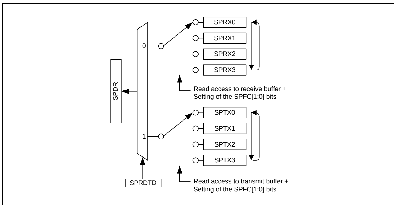
Figure 28.4 Configuration of SPDR (Reading)
