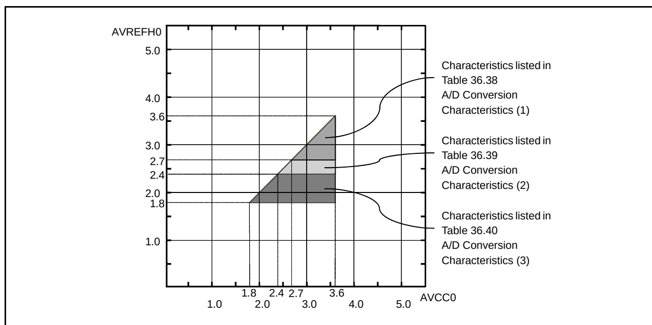
Figure 36.51 AVCC0 to AVREFH0 Voltage Range
