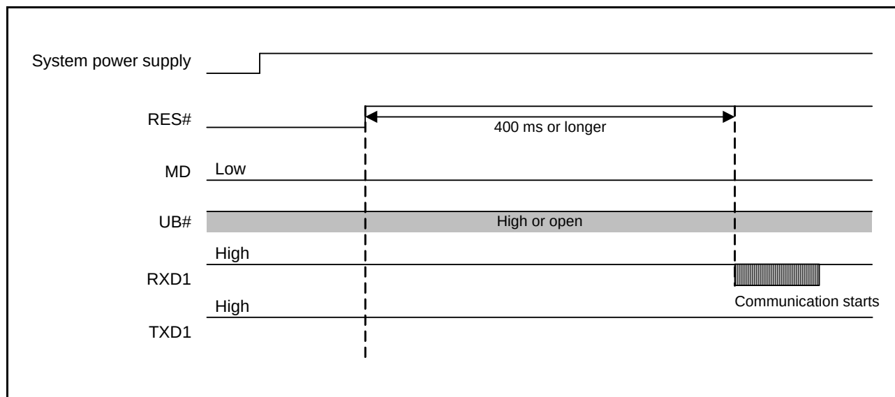
Figure 35.24 Pin States until Communication Becomes Possible in Boot Mode (SCI)
