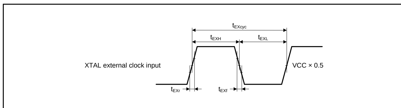
Figure 36.18 XTAL External Clock Input Timing
