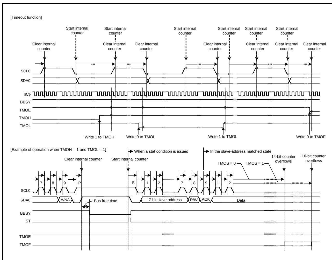
Figure 27.39 Timeout Function (ICMR1.CKS[2:0] = 000b)
