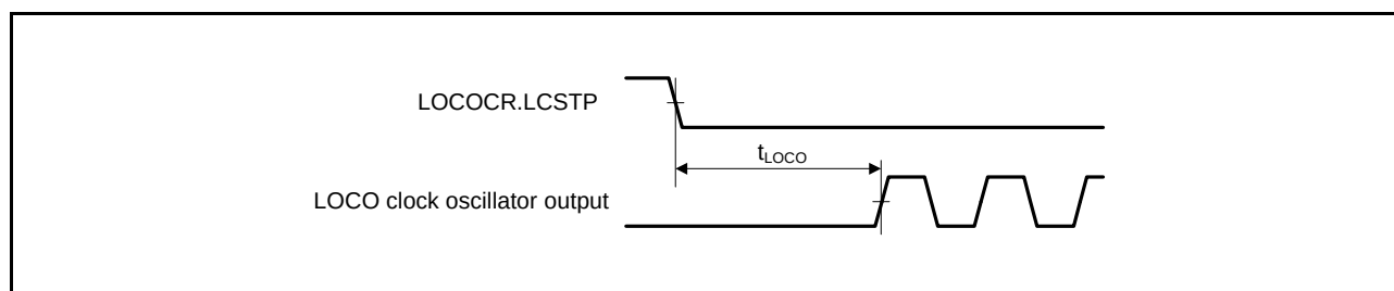
Figure 36.21 LOCO Clock Oscillation Start Timing
