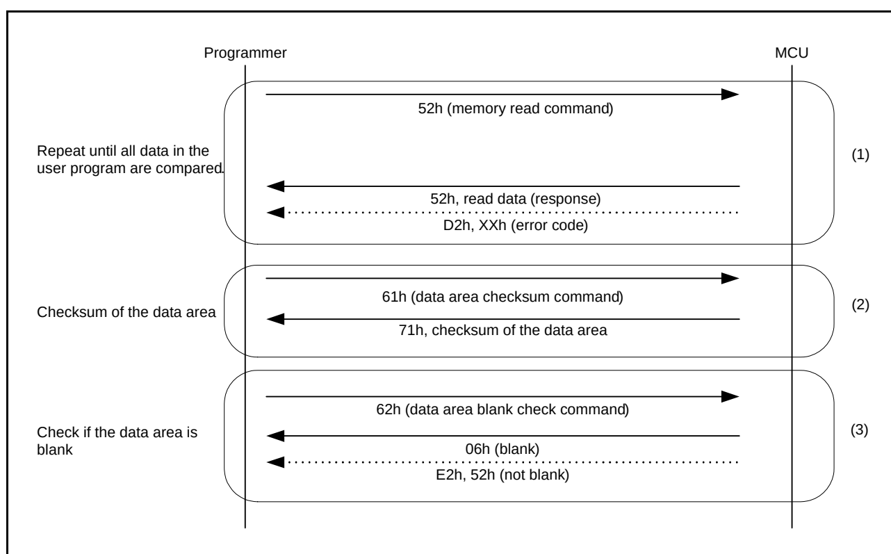
Figure 35.38 Procedure to Check Data in the Data Area
