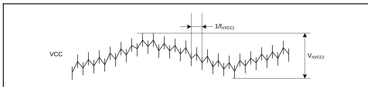
Figure 36.6 Ripple Waveform
