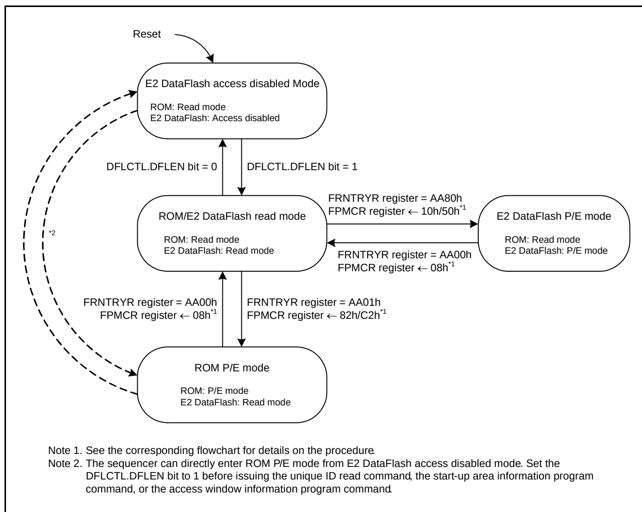
Figure 35.5 Mode Transitions of the Flash Memory
