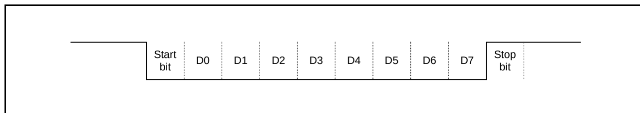
Figure 35.23 Communication Format
