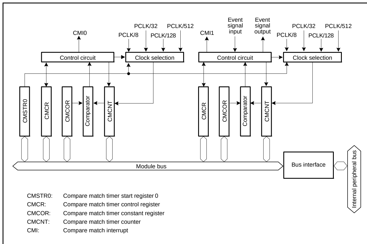
Figure 22.1 CMT (Unit 0) Block Diagram
