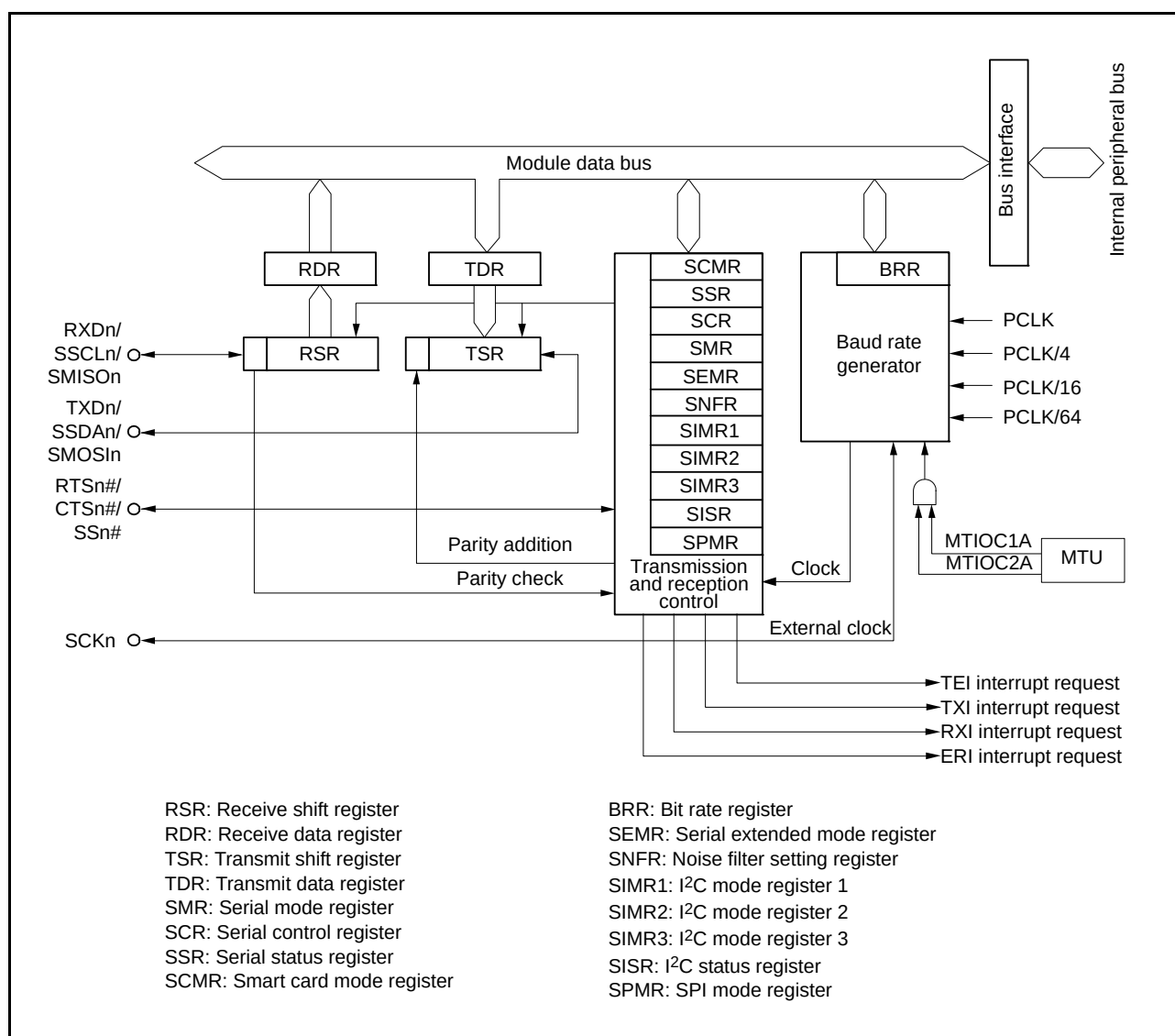
Figure 26.1 Block Diagram of SCIe (SCI1)
