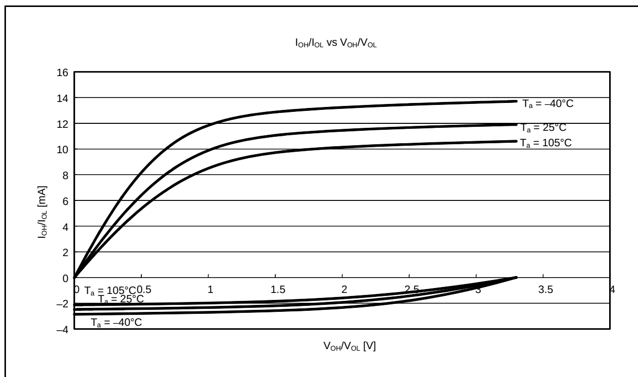
Figure 36.17 V_{OH}/V_{OL} and I_{OH}/I_{OL} Temperature Characteristics of Port 4 and Port J at V_{CC} = 3.3\text{ V} (Reference Data)
