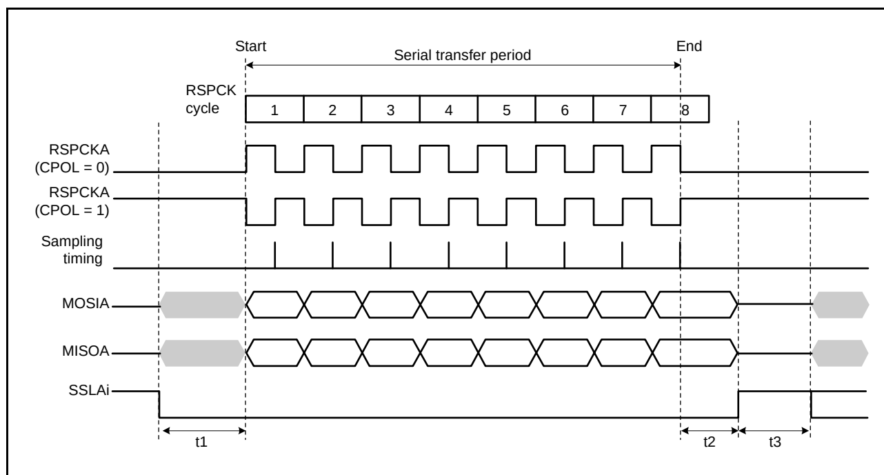
Figure 28.23 RSPI Transfer Format (CPHA = 1)
