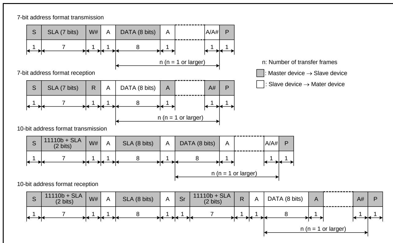
Figure 26.44 I 2 C Bus Format
