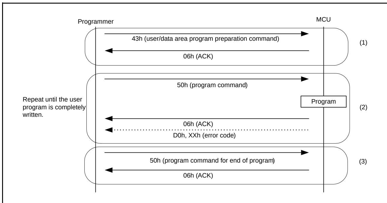
Figure 35.36 Procedure to Program the User Area and Data Area
