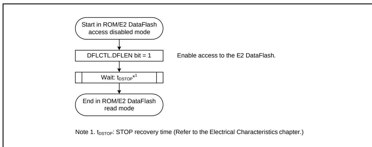
Figure 35.6 Procedure for Transition from E2 DataFlash Access Disabled Mode to ROM/E2 DataFlash Read Mode
