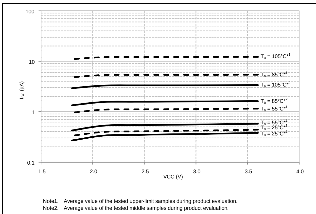
Figure 36.4 Voltage Dependency in Software Standby Mode (Reference Data)
