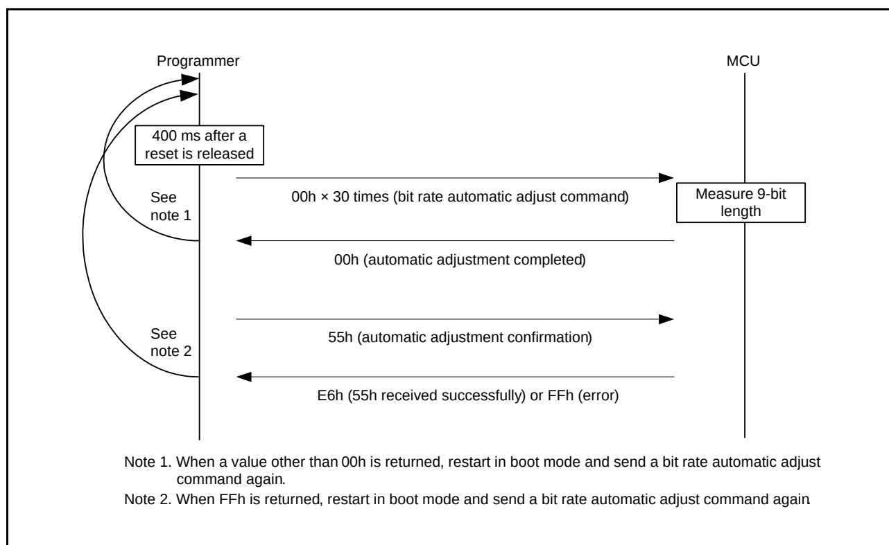
Figure 35.29 Bit Rate Automatic Adjustment Procedure
