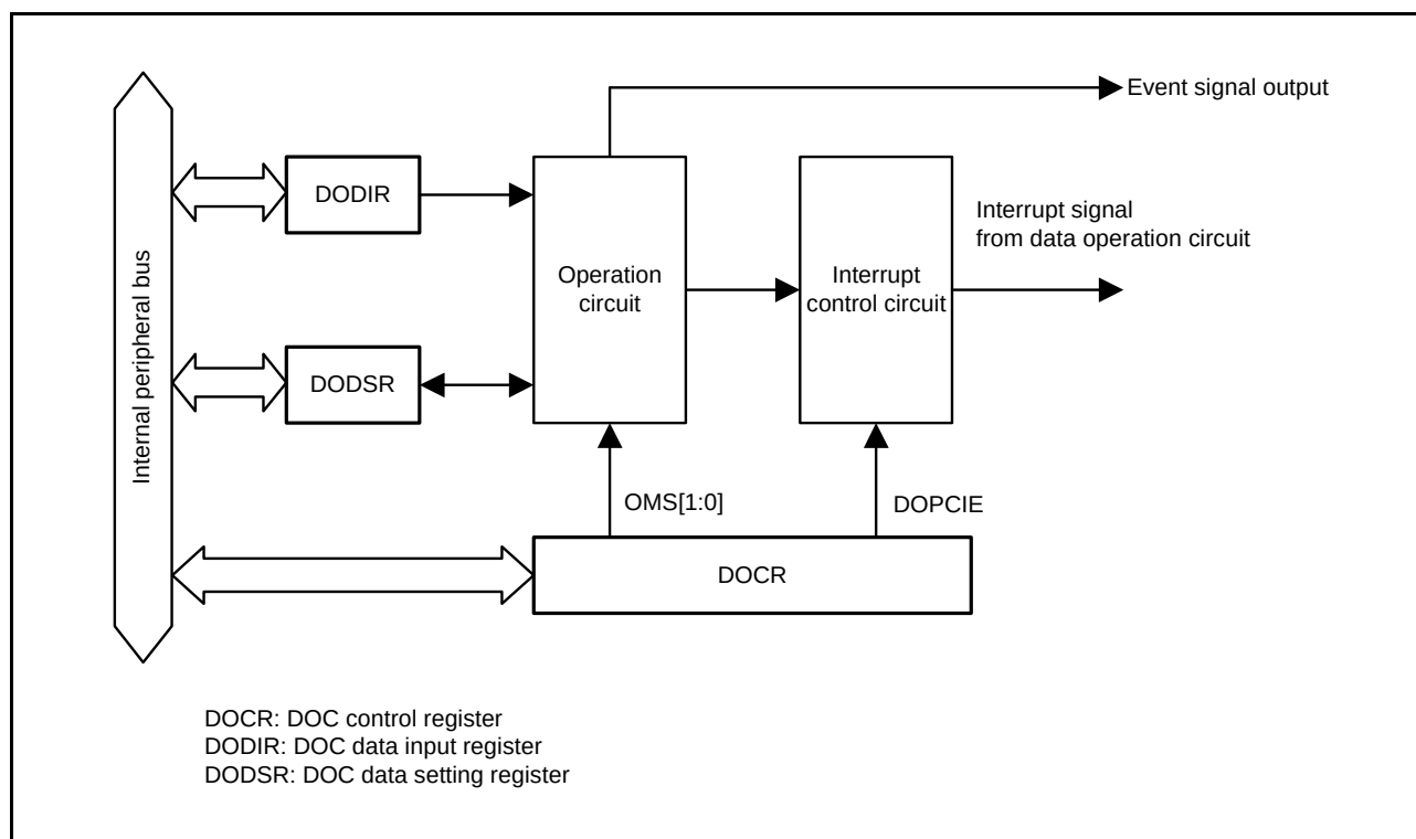
Figure 33.1 DOC Block Diagram
