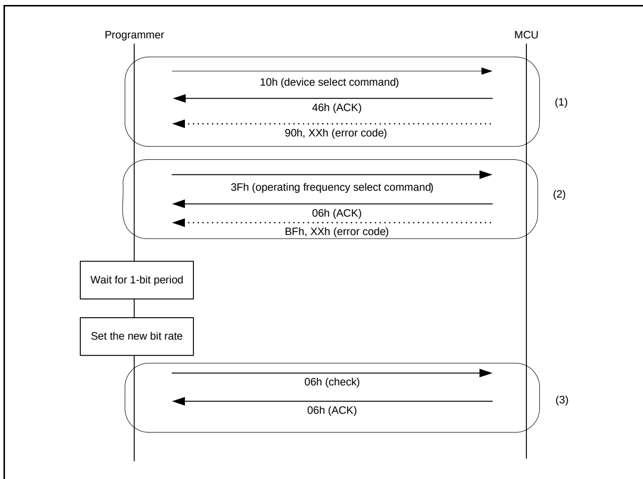
Figure 35.31 Procedure to Select the Device and Change the Bit Rate
