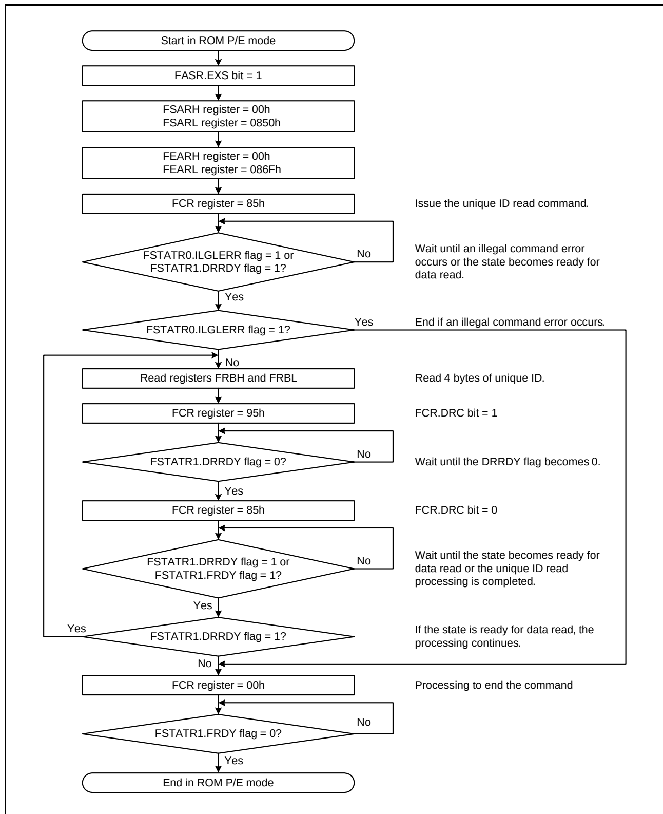
Figure 35.18 Procedure to Issue the Unique ID Read Command
