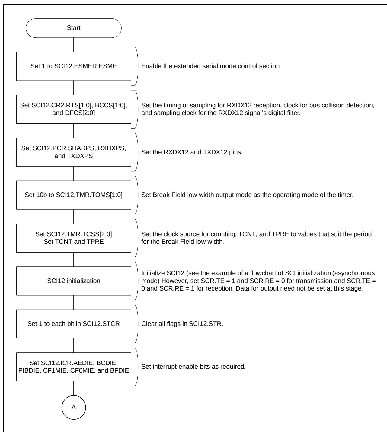
Figure 26.59 Example of Start Frame Transmission (1/2)
