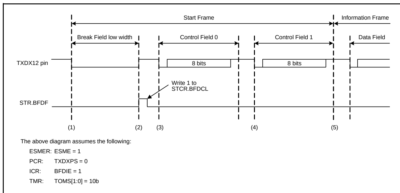
Figure 26.58 Example of Operations When Transmitting a Start Frame
