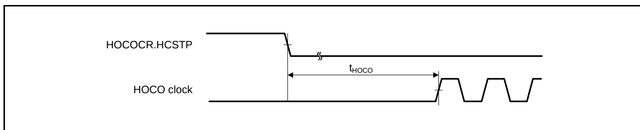
Figure 36.23 HOCO Clock Oscillation Start Timing (Oscillation is Started by Setting HOCOCR.HCSTP Bit)
