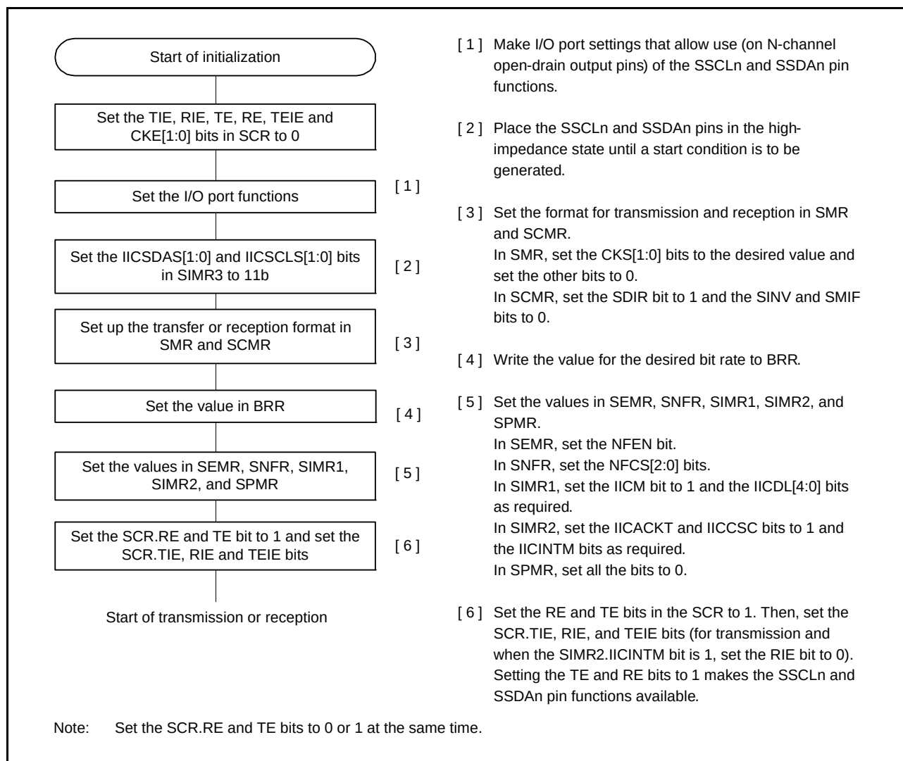
Figure 26.49 Example of the Flowchart of SCI Initialization (for Simple I 2 C Mode)
