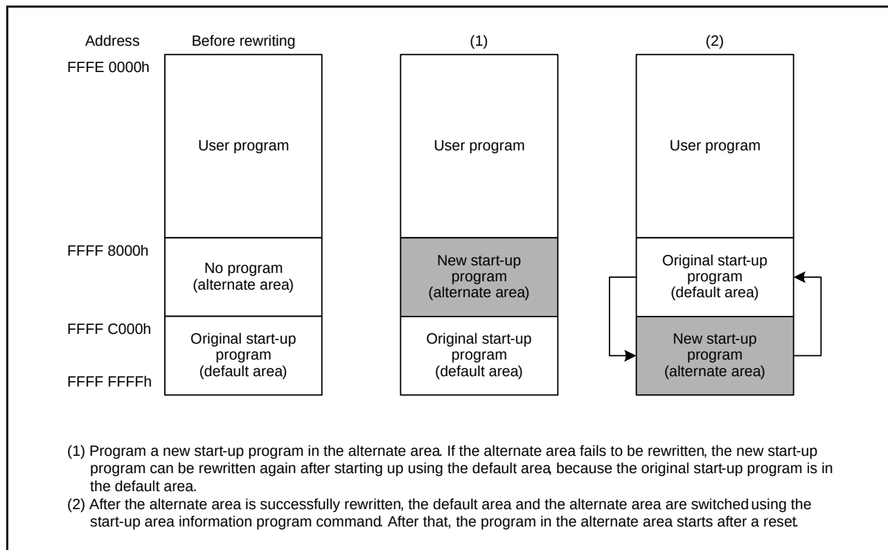
Figure 35.3 Overview of the Start-Up Program Protection
