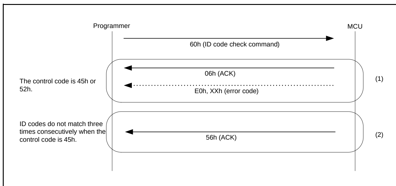
Figure 35.33 Procedure to Check ID Codes
