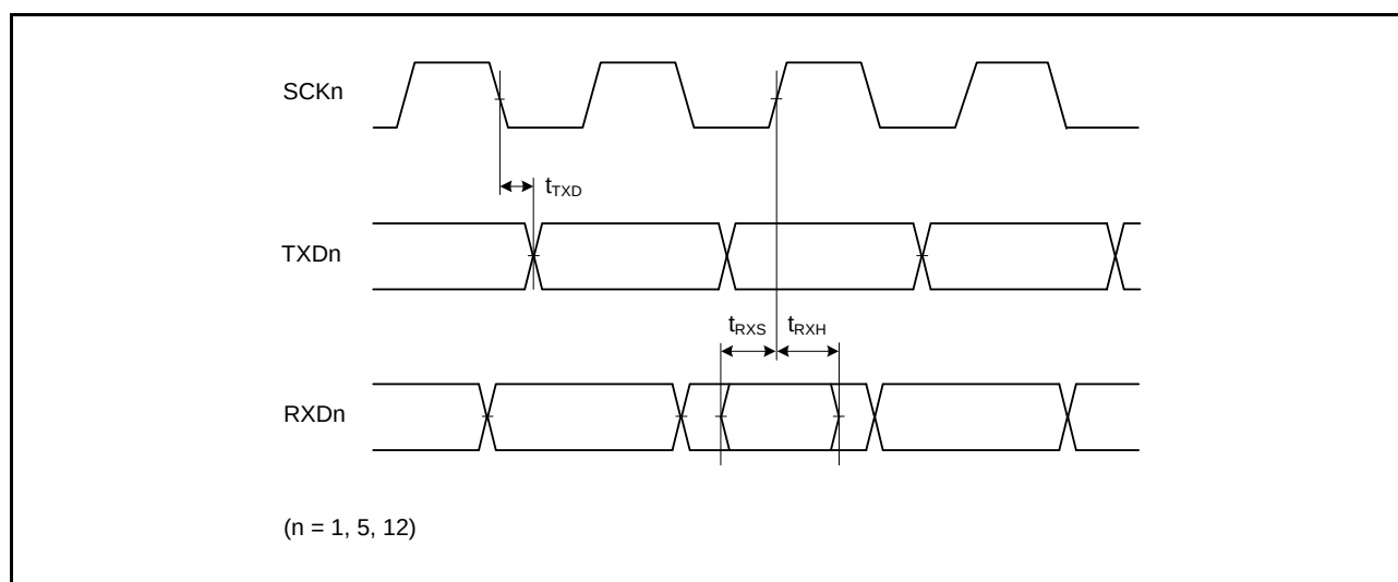
Figure 36.38 SCI Input/Output Timing: Clock Synchronous Mode
