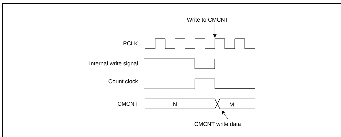
Figure 22.6 Conflict between CMCNT Counter Writing and Incrementing
