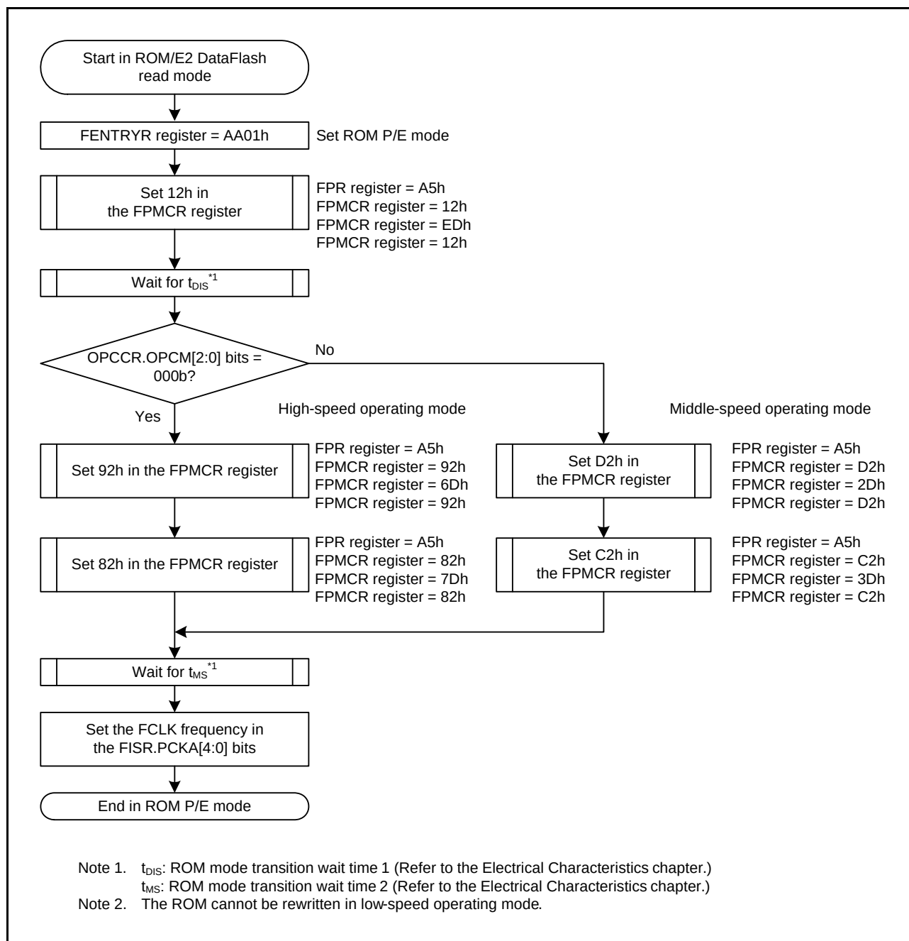
Figure 35.7 Procedure for Transition from ROM/E2 DataFlash Read Mode to ROM P/E Mode
