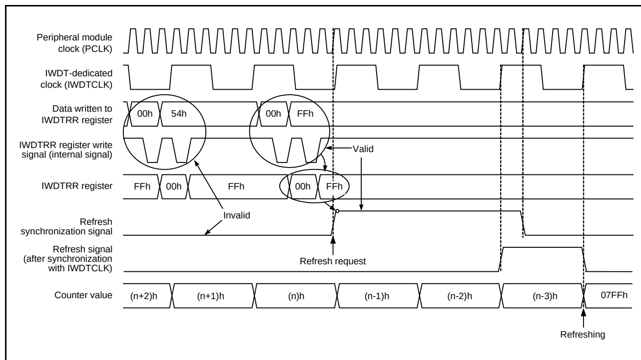
Figure 24.6 IWDt Refresh Operation Waveforms (IWDtCR.CKS[3:0] = 0000b, IWDtCR.TOPS[1:0] = 11b)
