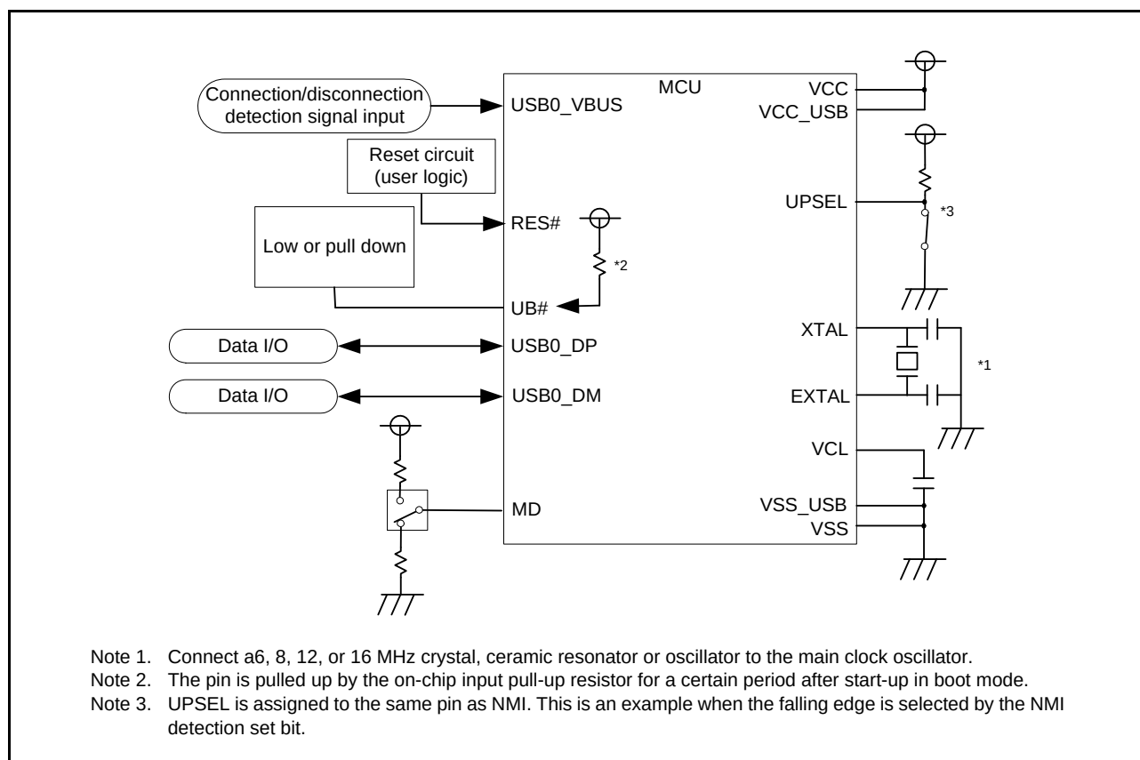
Figure 35.20 Example of Pin Connections in Boot Mode (USB Interface) When Self-Powered
