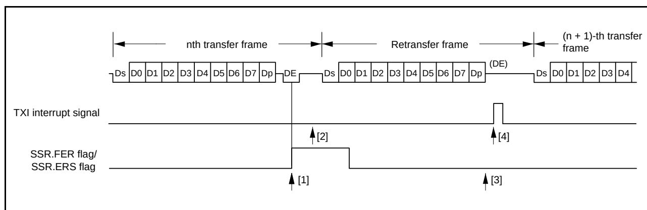
Figure 26.38 Data Retransfer Operation in SCI Transmission Mode
