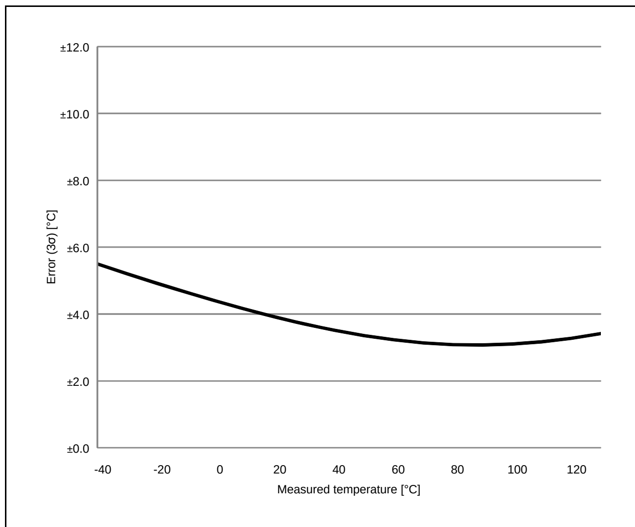
Figure 32.2 Error in the Measured Temperature (Designed Value)
