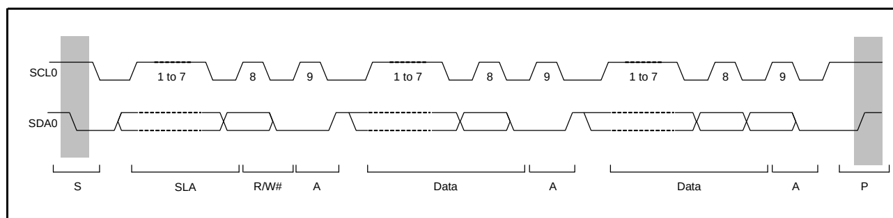
Figure 27.4 I 2 C Bus Timing (SLA = 7 Bits)
