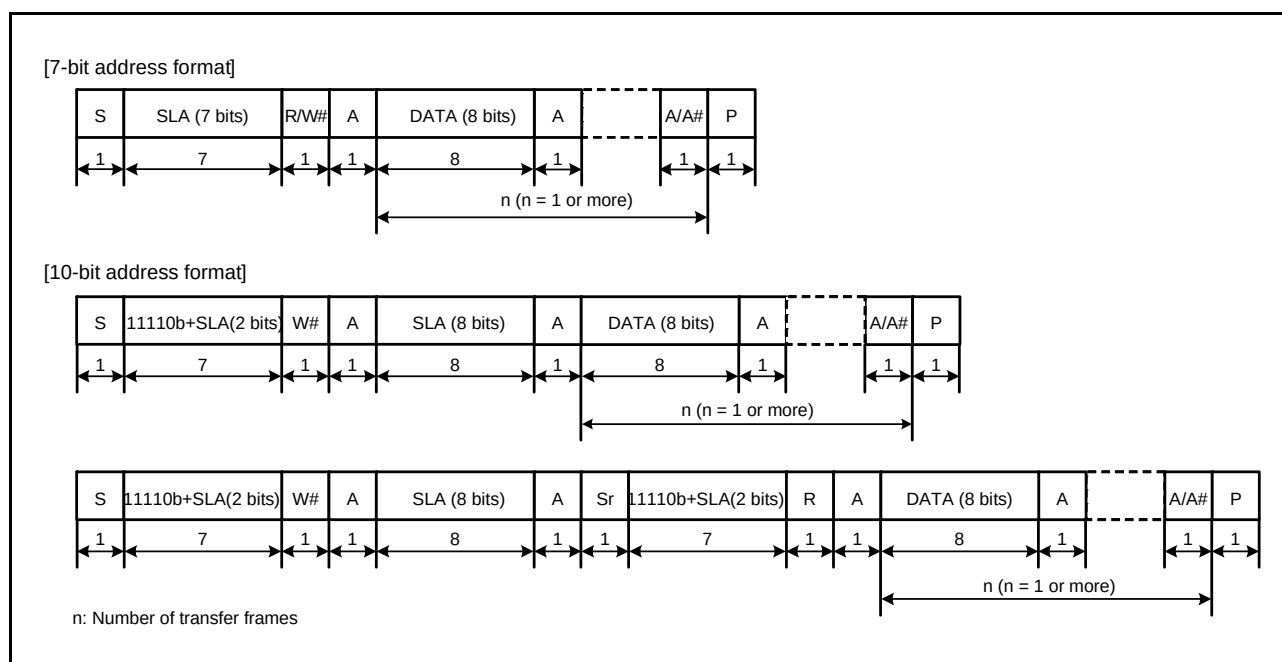
Figure 27.3 I 2 C Bus Format
