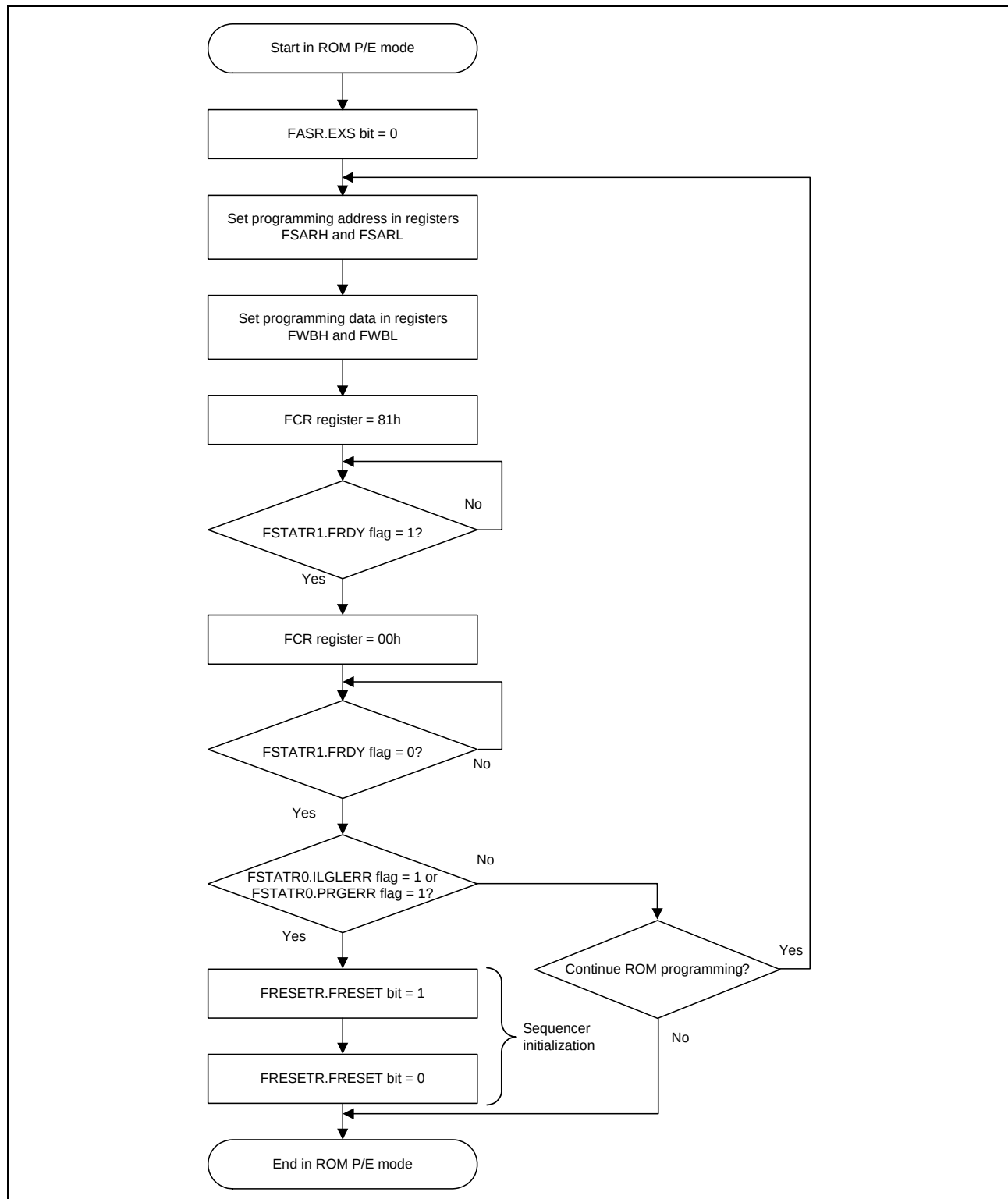
Figure 35.11 Procedure to Issue the Program Command for the ROM
