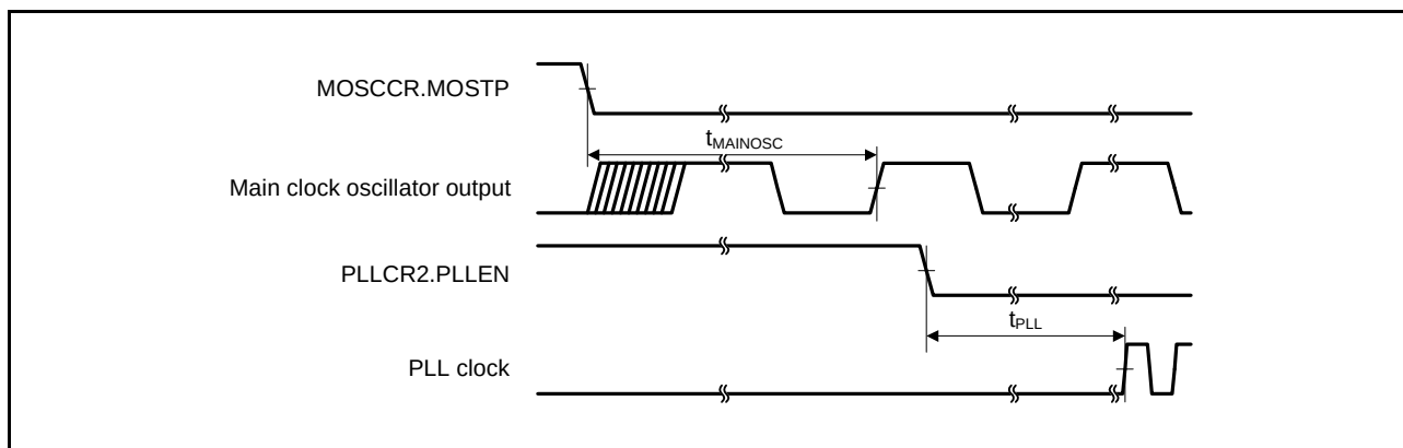
Figure 36.24 PLL Clock Oscillation Start Timing (PLL is Operated after Main Clock Oscillation Has Settled)
