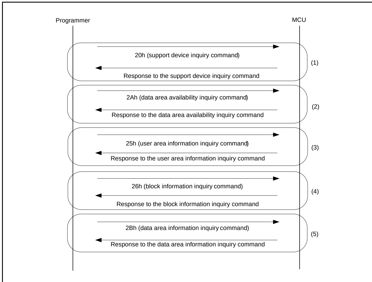
Figure 35.30 Procedure to Send Inquiry Commands
