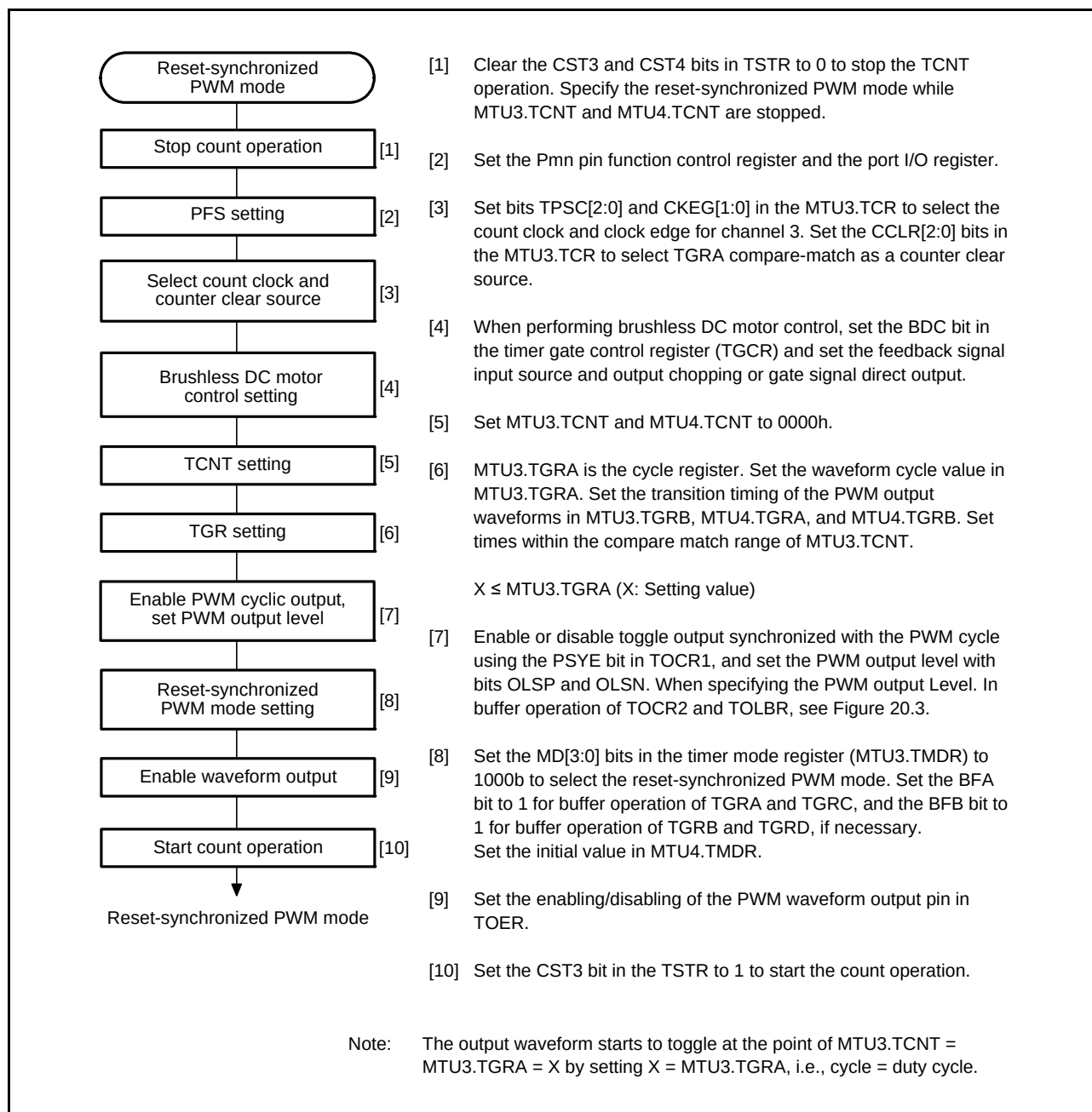
Figure 20.35 Procedure for Selecting Reset-Synchronized PWM Mode
