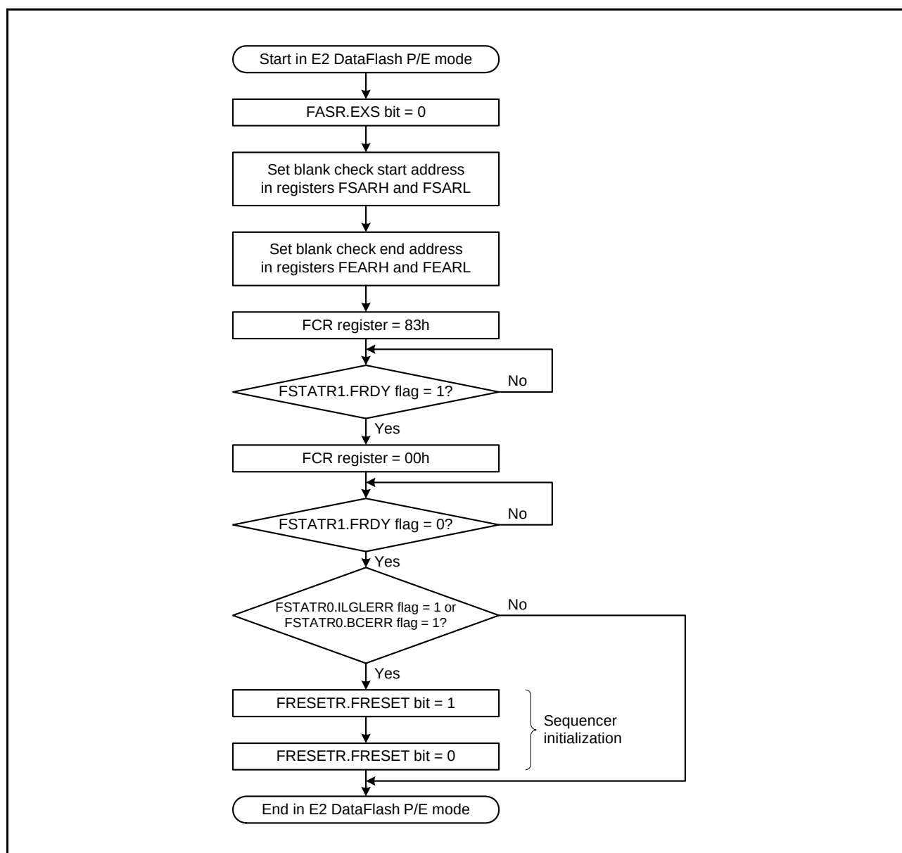
Figure 35.16 Procedure to Issue the Blank Check Command for the E2 DataFlash
