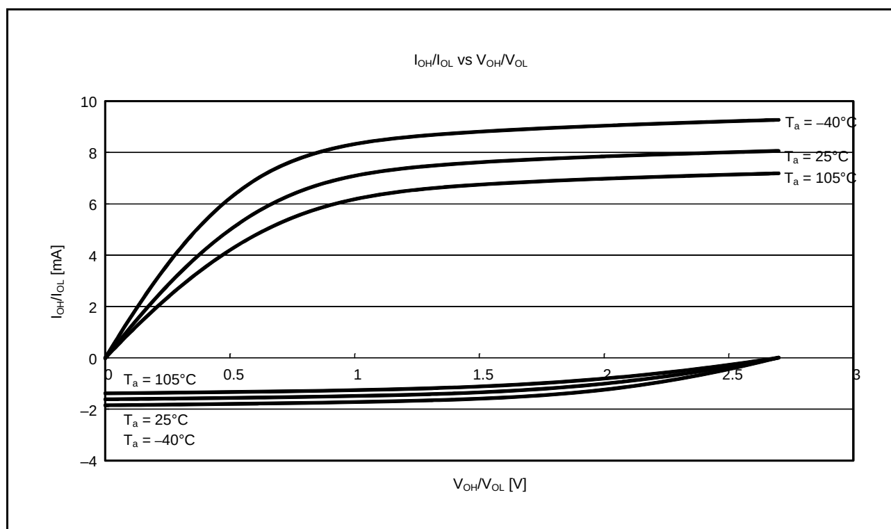
Figure 36.16 V_{OH}/V_{OL} and I_{OH}/I_{OL} Temperature Characteristics of Port 4 and Port J at V_{CC} = 2.7\text{ V} (Reference Data)
