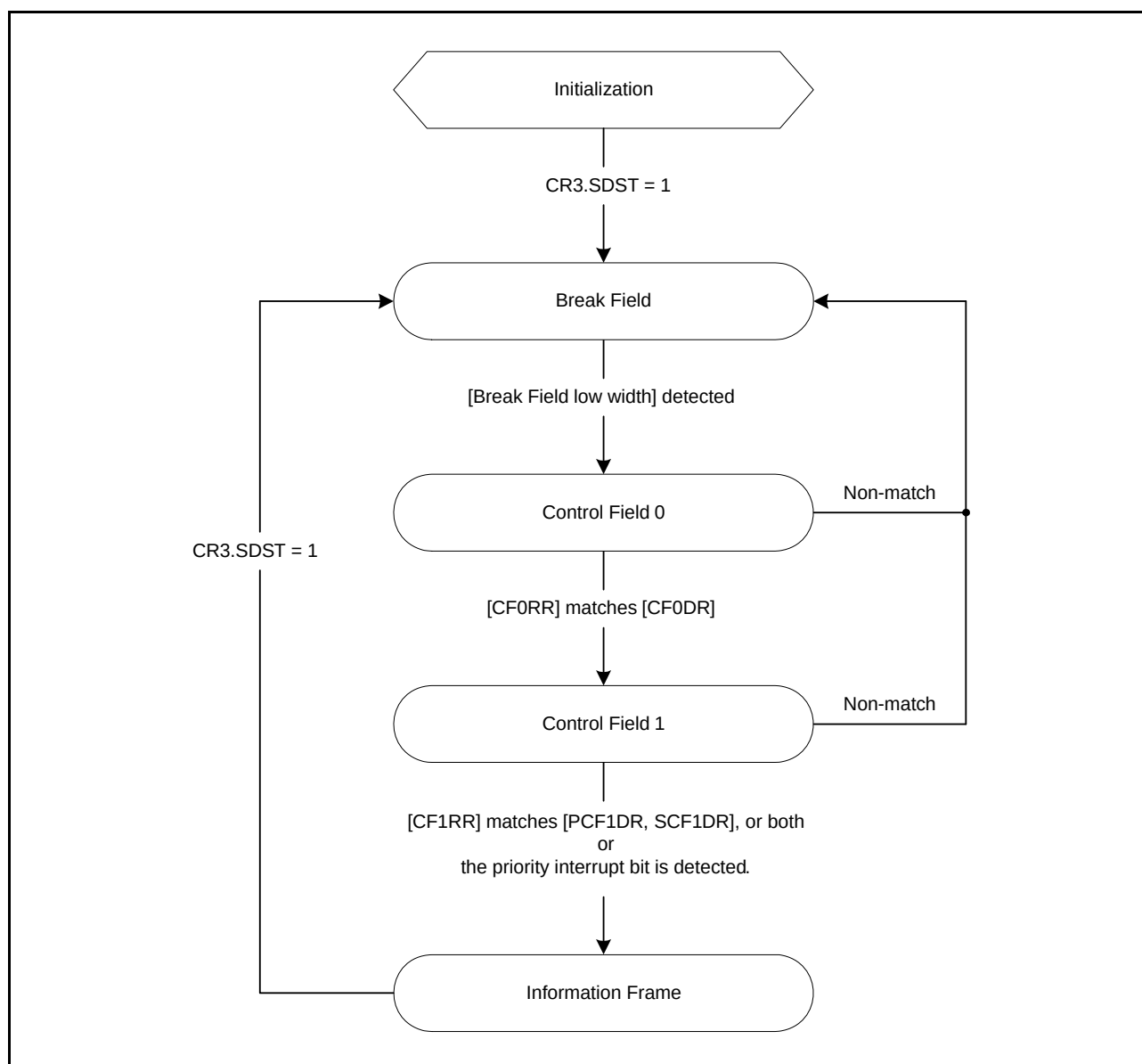
Figure 26.64 State Transitions When Receiving a Start Frame
