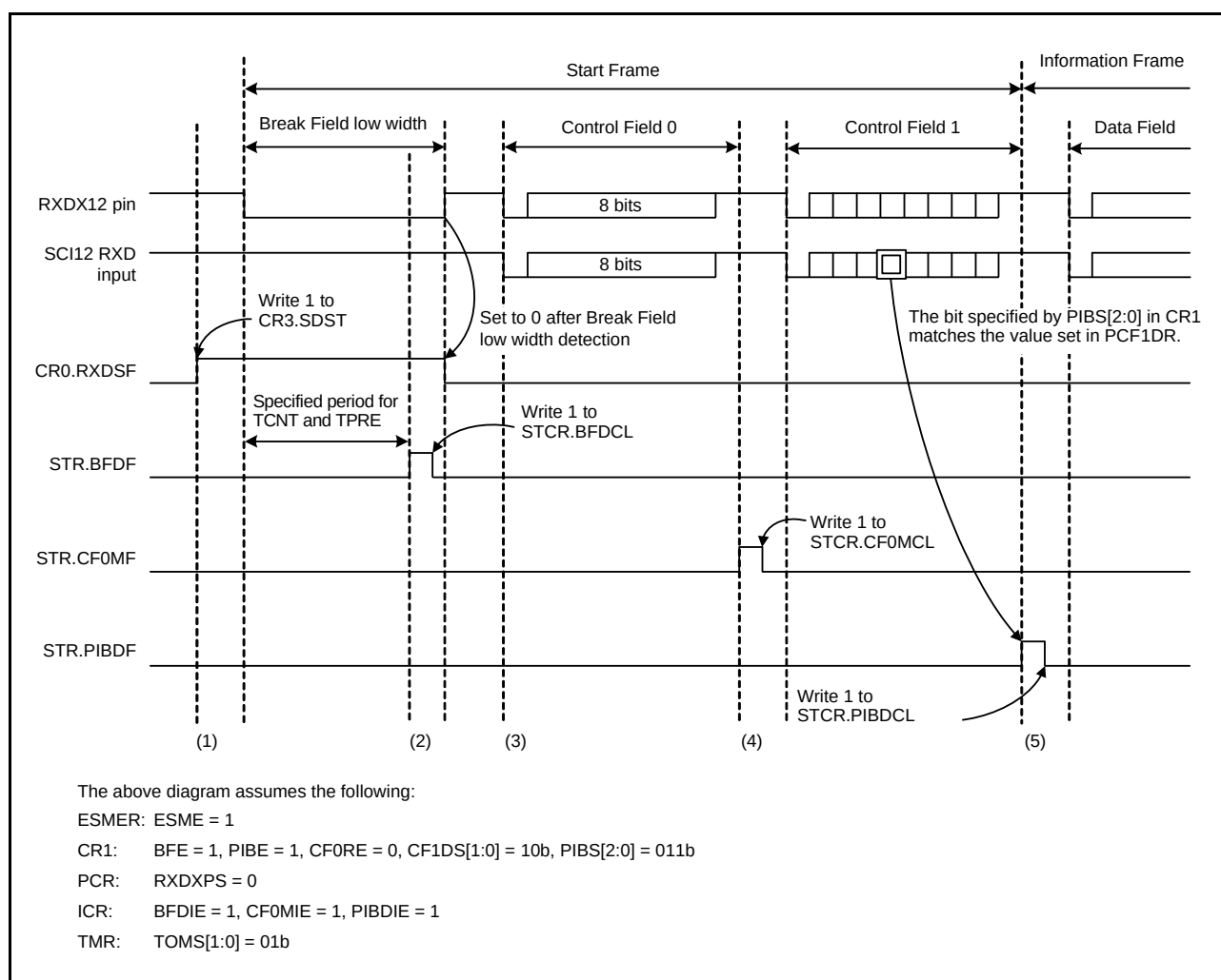
Figure 26.65 Example of Operations When Receiving a Start Frame While the CR1.PIBE Bit is 1
