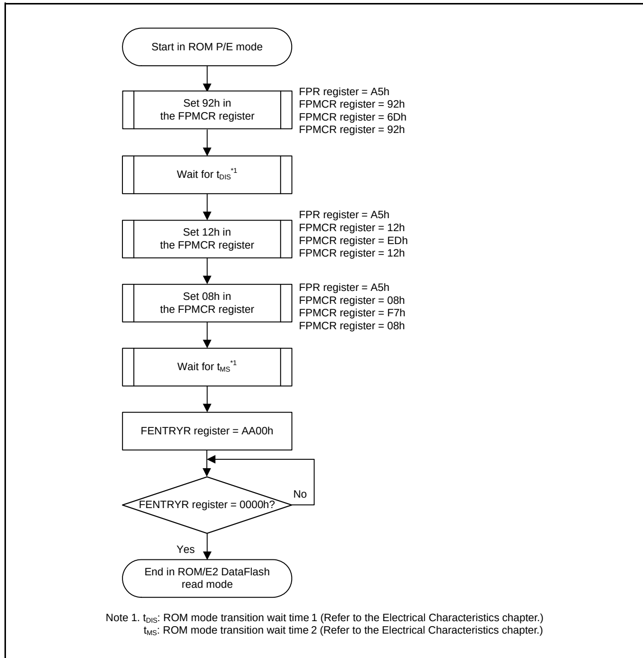
Figure 35.9 Procedure for Transition from ROM P/E Mode to ROM/E2 DataFlash Read Mode
