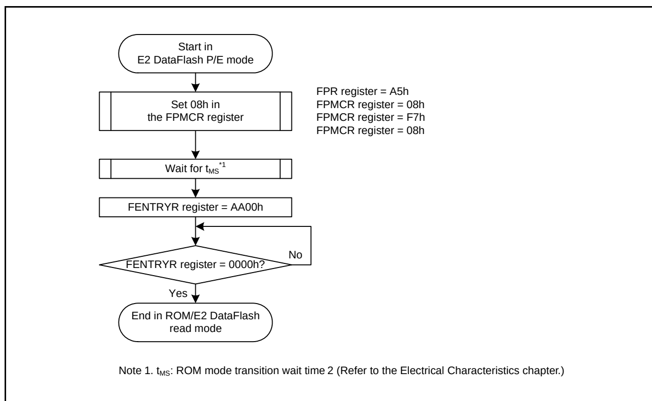
Figure 35.10 Procedure for Transition from E2 DataFlash P/E Mode to ROM/E2 DataFlash Read Mode
