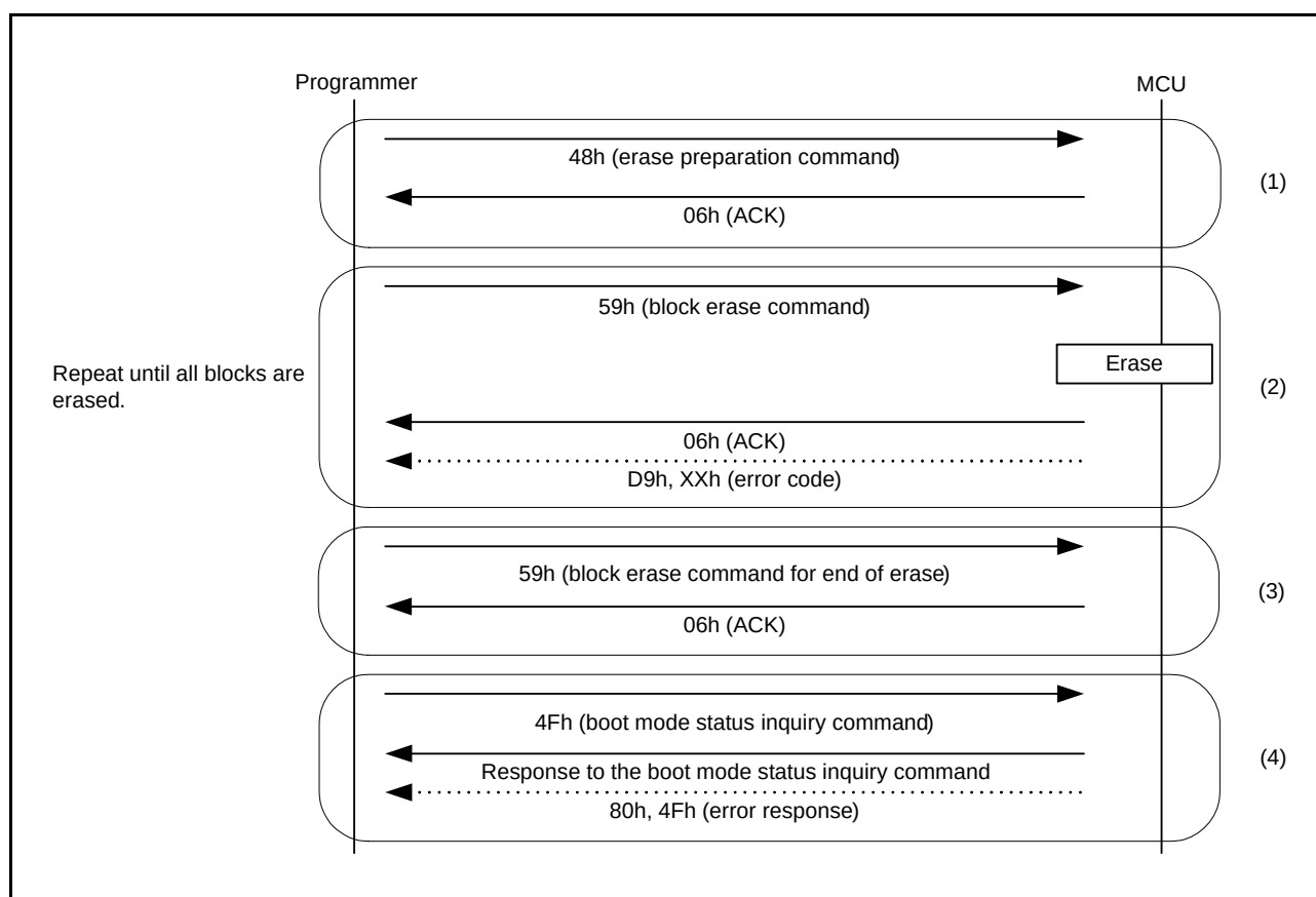
Figure 35.34 Procedure to Send Commands in Erase Ready Operation
