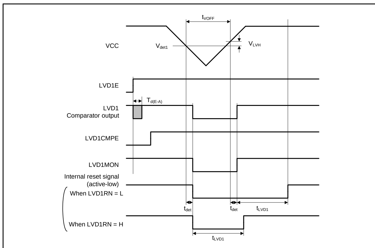
Figure 36.55 Voltage Detection Circuit Timing ( V_{det1} )
