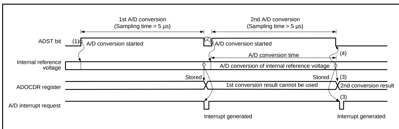
Figure 30.5 Example of Operation in Single Scan Mode (Internal Reference Voltage Selected)
