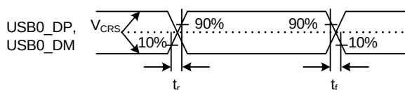
Figure 36.49 USB0_DP and USB0_DM Output Timing
