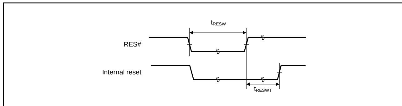
Figure 36.27 Reset Input Timing (1)
