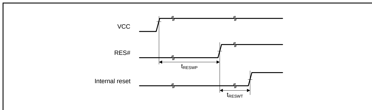
Figure 36.26 Reset Input Timing at Power-On
