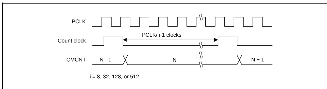
Figure 22.3 CMCNT Count Timing
