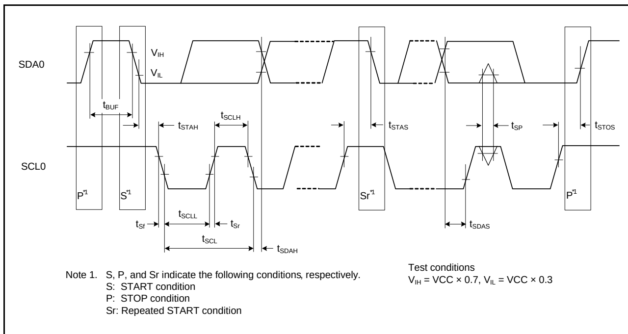
Figure 36.48 RIIC Bus Interface Input/Output Timing and Simple I 2 C Bus Interface Input/Output Timing
