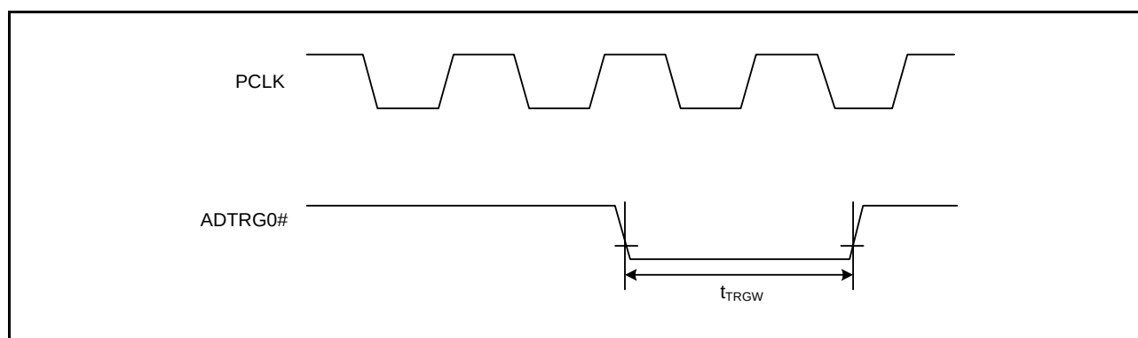
Figure 36.39 A/D Converter External Trigger Input Timing
