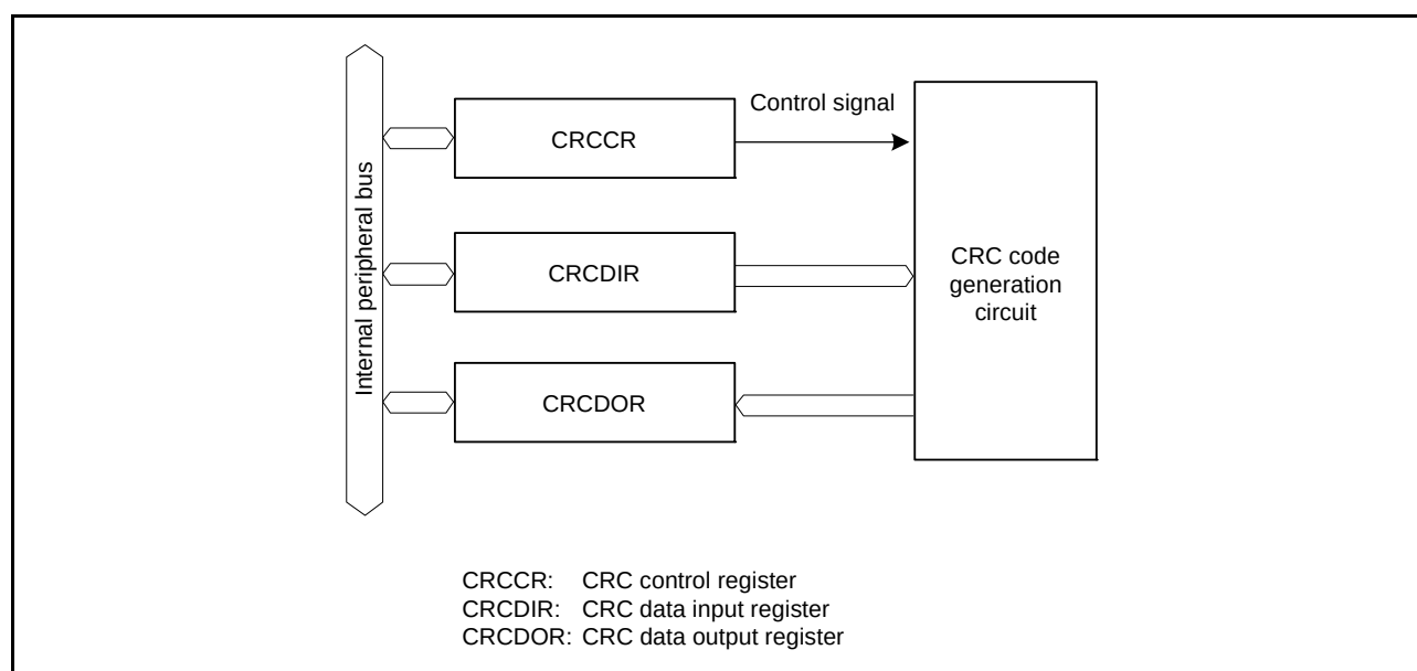
Figure 29.1 CRC Block Diagram
