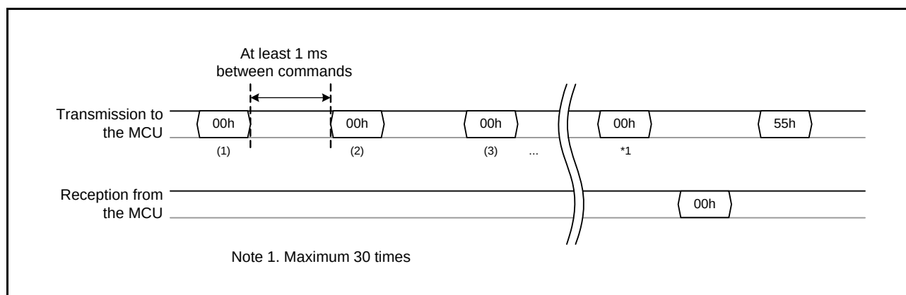
Figure 35.28 Transmit/Receive Data for Bit Rate Automatic Adjustment
