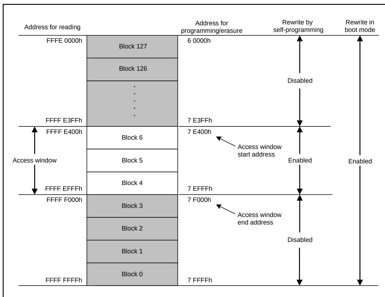
Figure 35.4 Area Protection Overview (When Blocks 4 to 6 are Set as the Access Window in Products with 128-Kbyte ROM)
