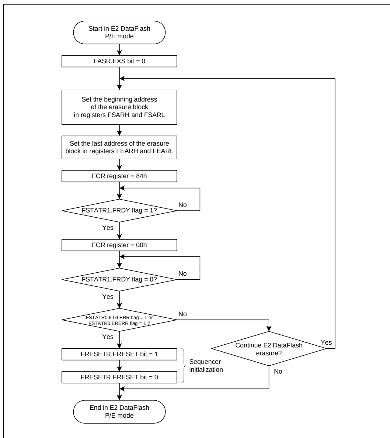
Figure 35.14 Procedure to Issue the Block Erase Command for the E2 DataFlash
