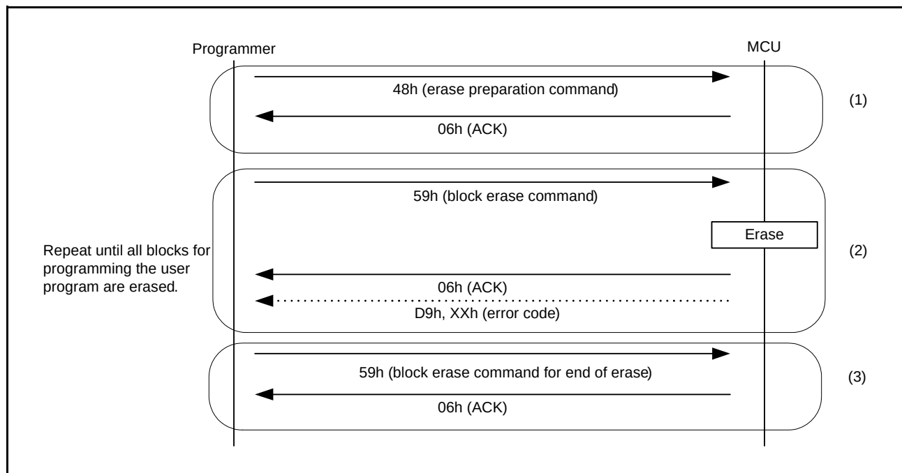
Figure 35.35 Procedure to Erase the User Area and Data Area
