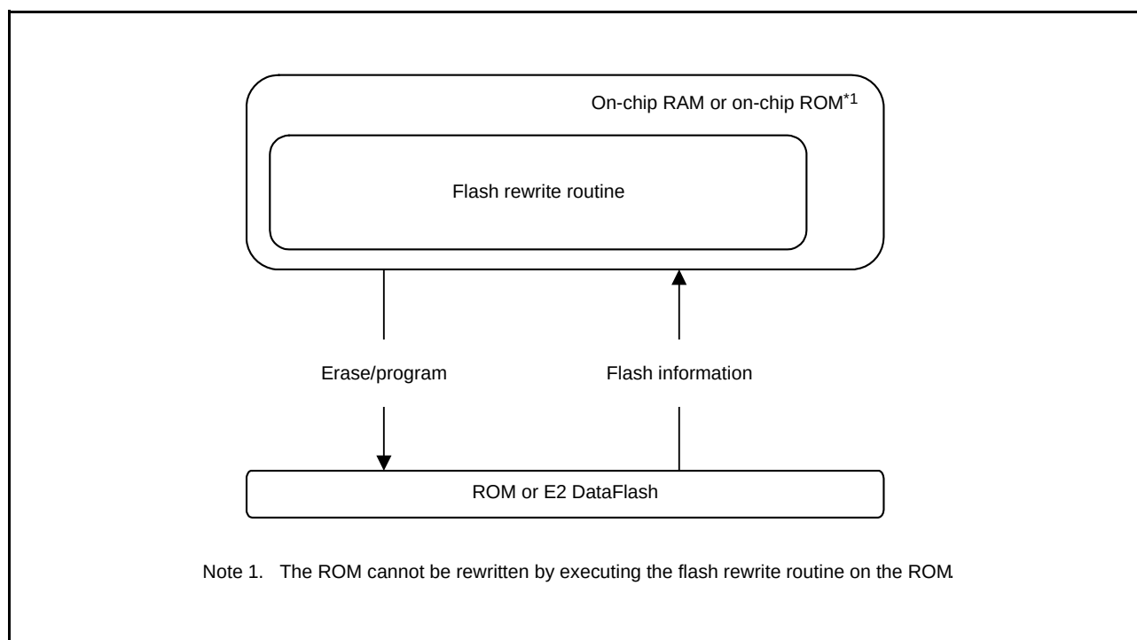
Figure 35.40 Self-Programming Overview
