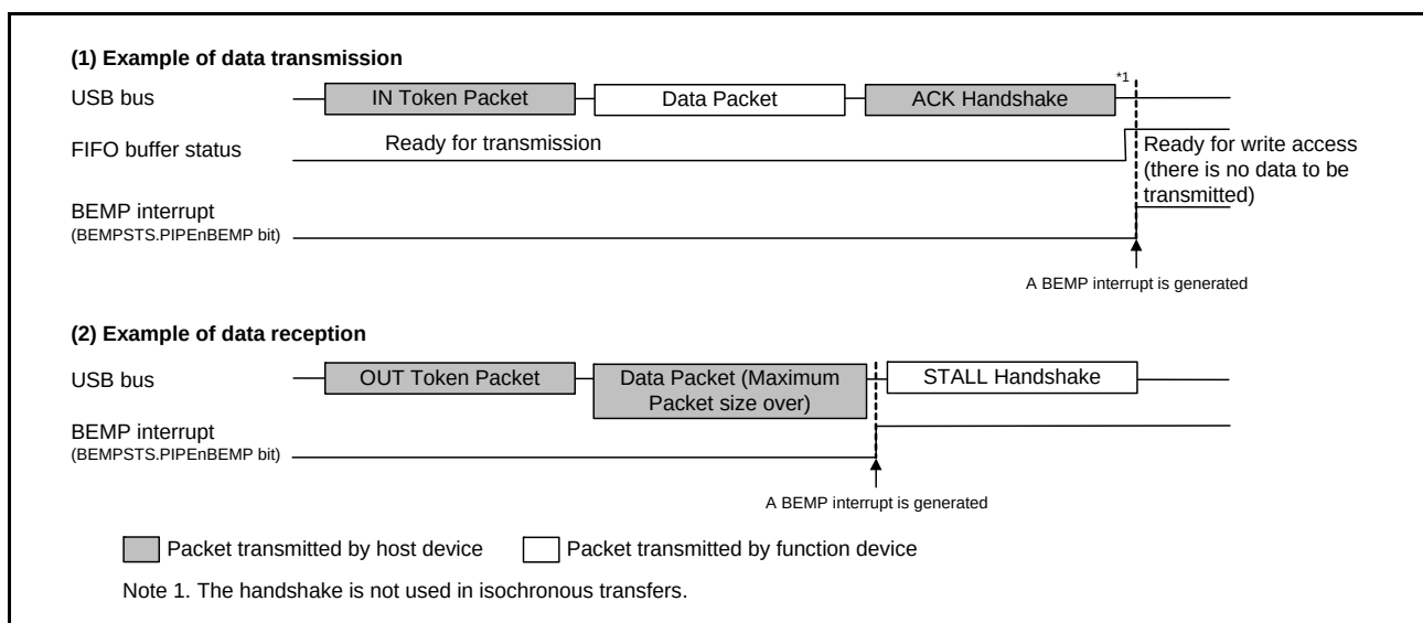
Figure 25.10 Timing of BEMP Interrupt Generation (When Function Controller is Selected)
