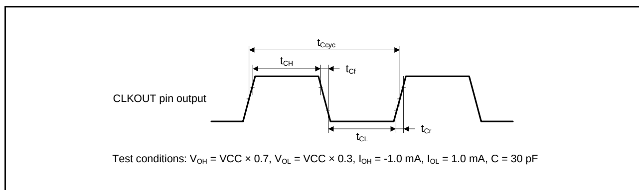
Figure 36.40 CLKOUT Output Timing
