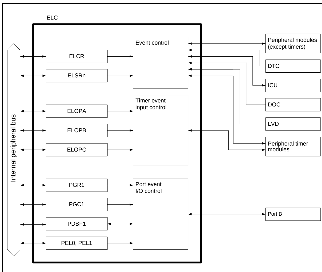
Figure 17.1 ELC Block Diagram (n = 1 to 4, 7, 15, 16, 18, 20, 22, 24, 25)
