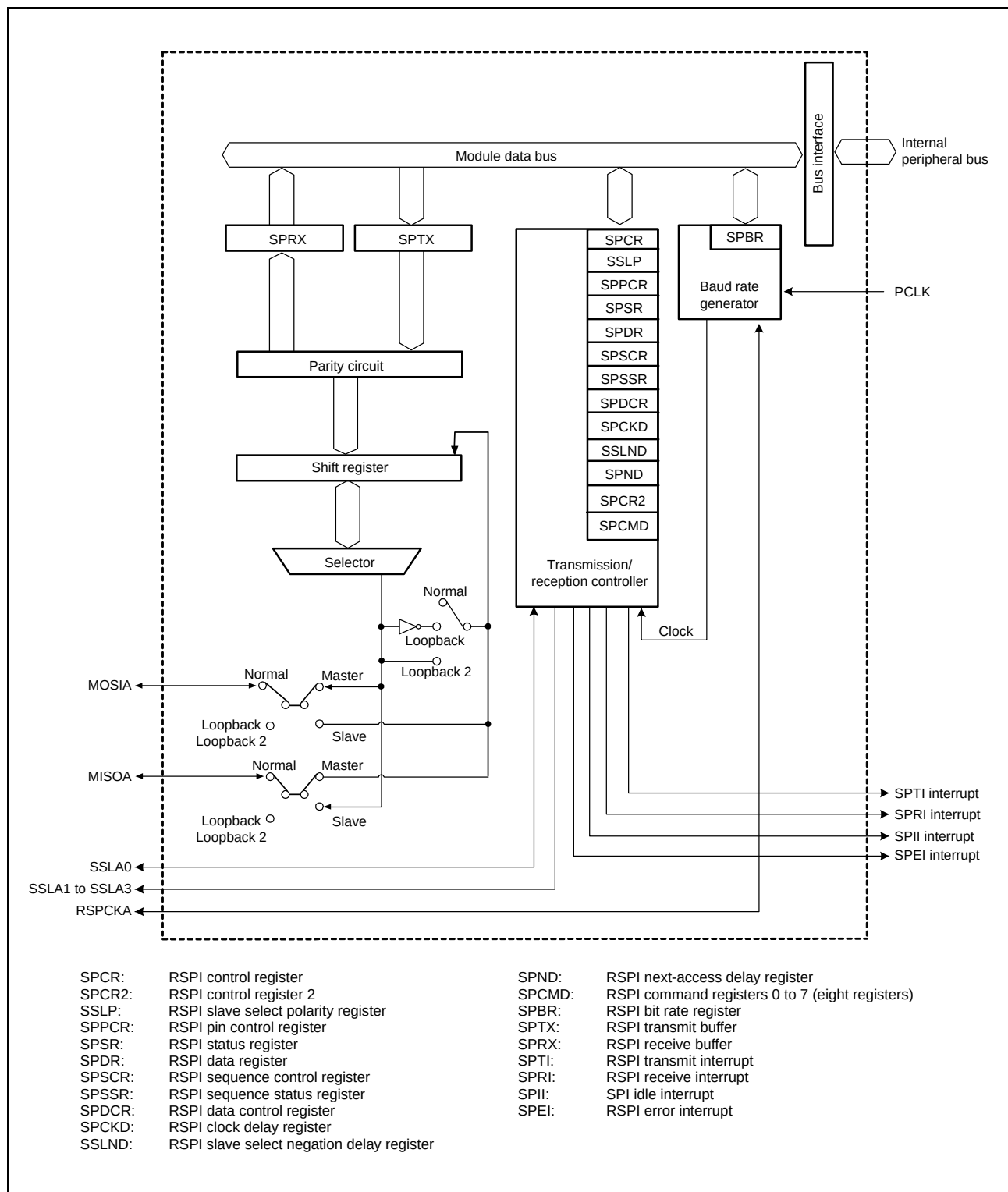
Figure 28.1 RSPI Block Diagram
