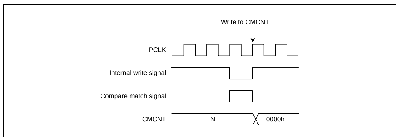
Figure 22.5 Conflict between CMCNT Counter Writing and Compare Match
