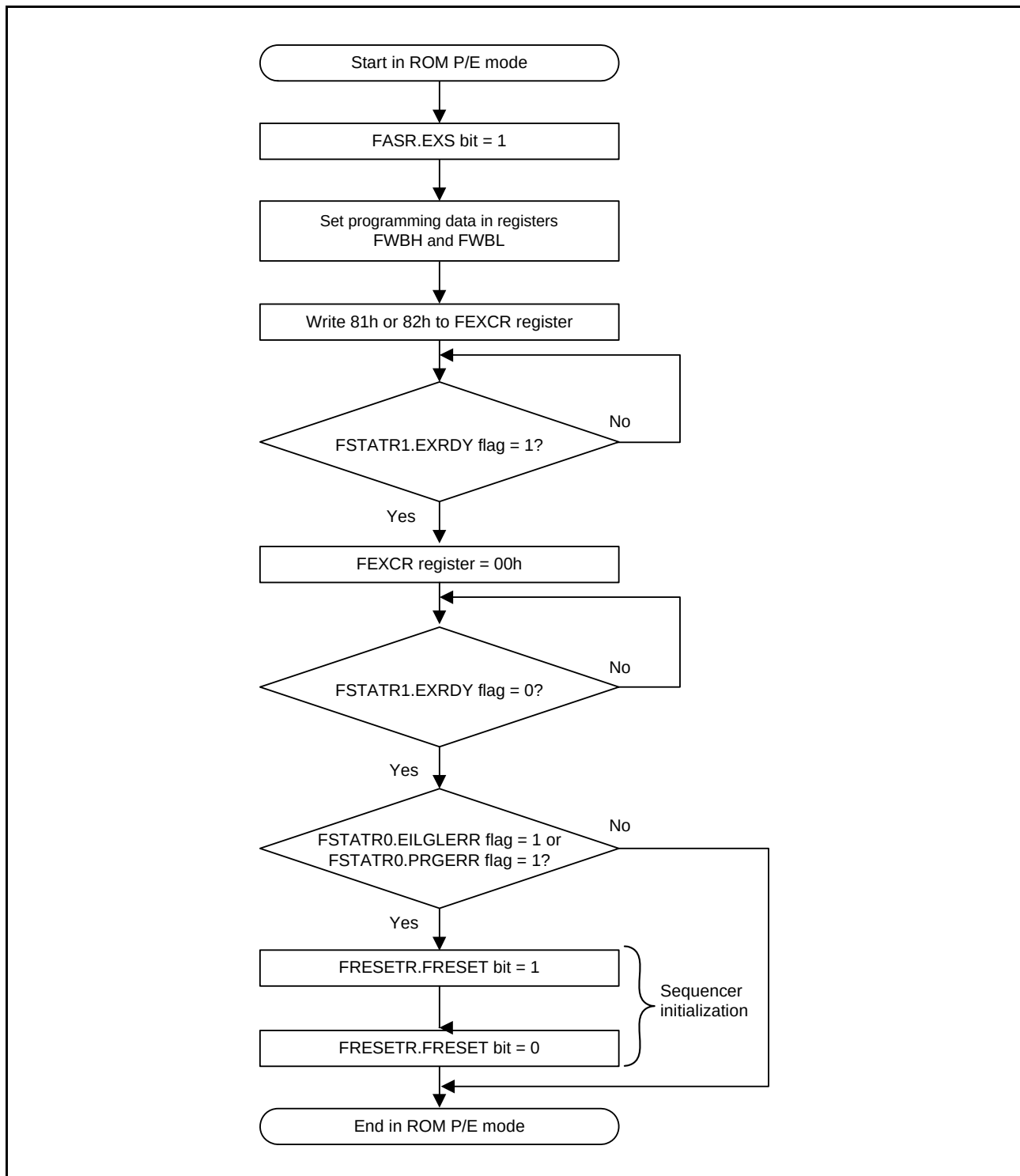
Figure 35.17 Procedure to Issue the Start-Up Area Information Program Command/Access Window Information Program Command
