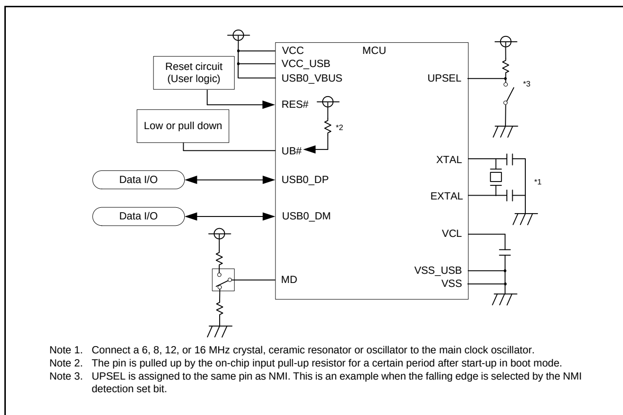
Figure 35.21 Example of Pin Connections in Boot Mode (USB Interface) When Bus-Powered
