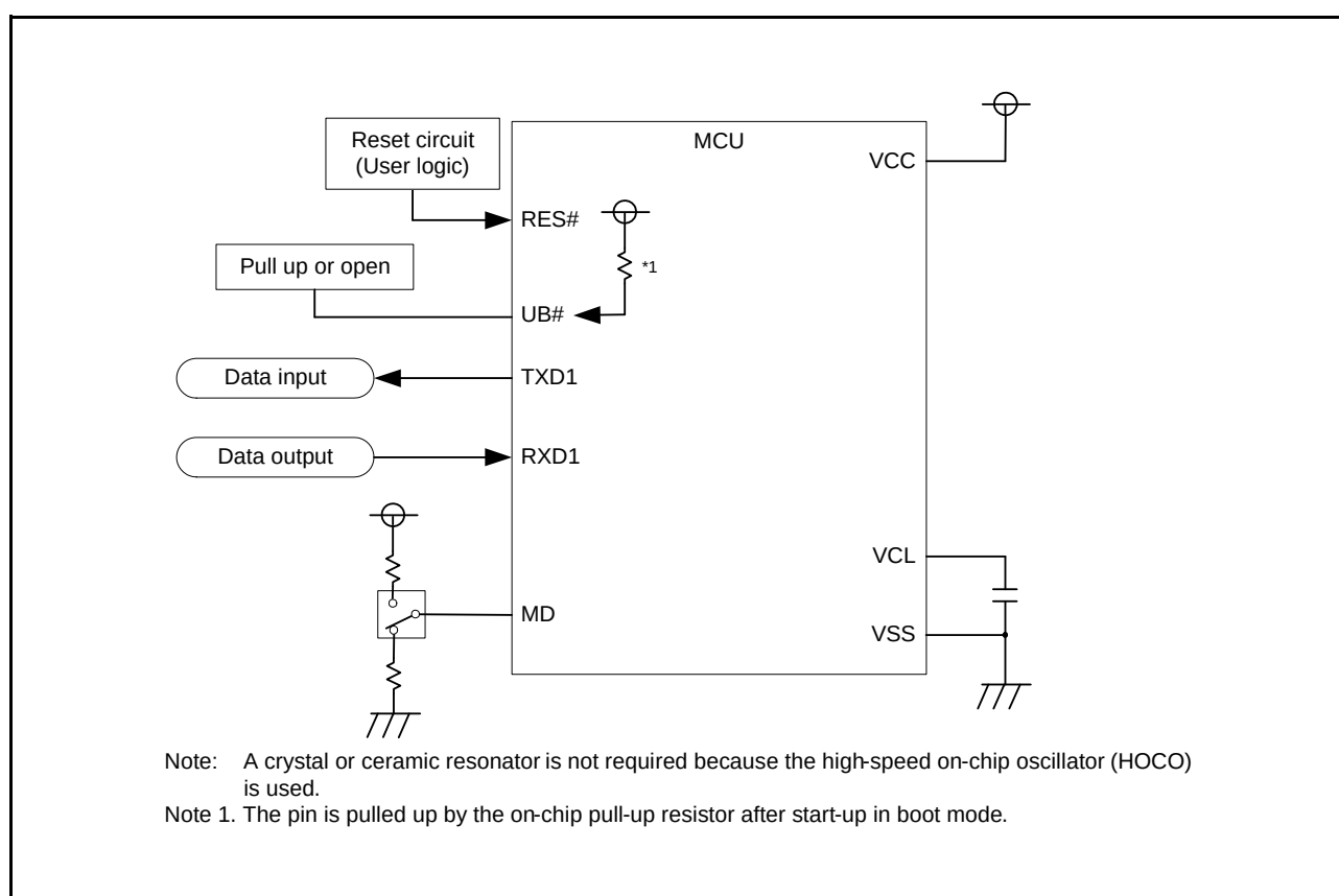
Figure 35.22 Example of Pin Connections in Boot Mode (SCI)
