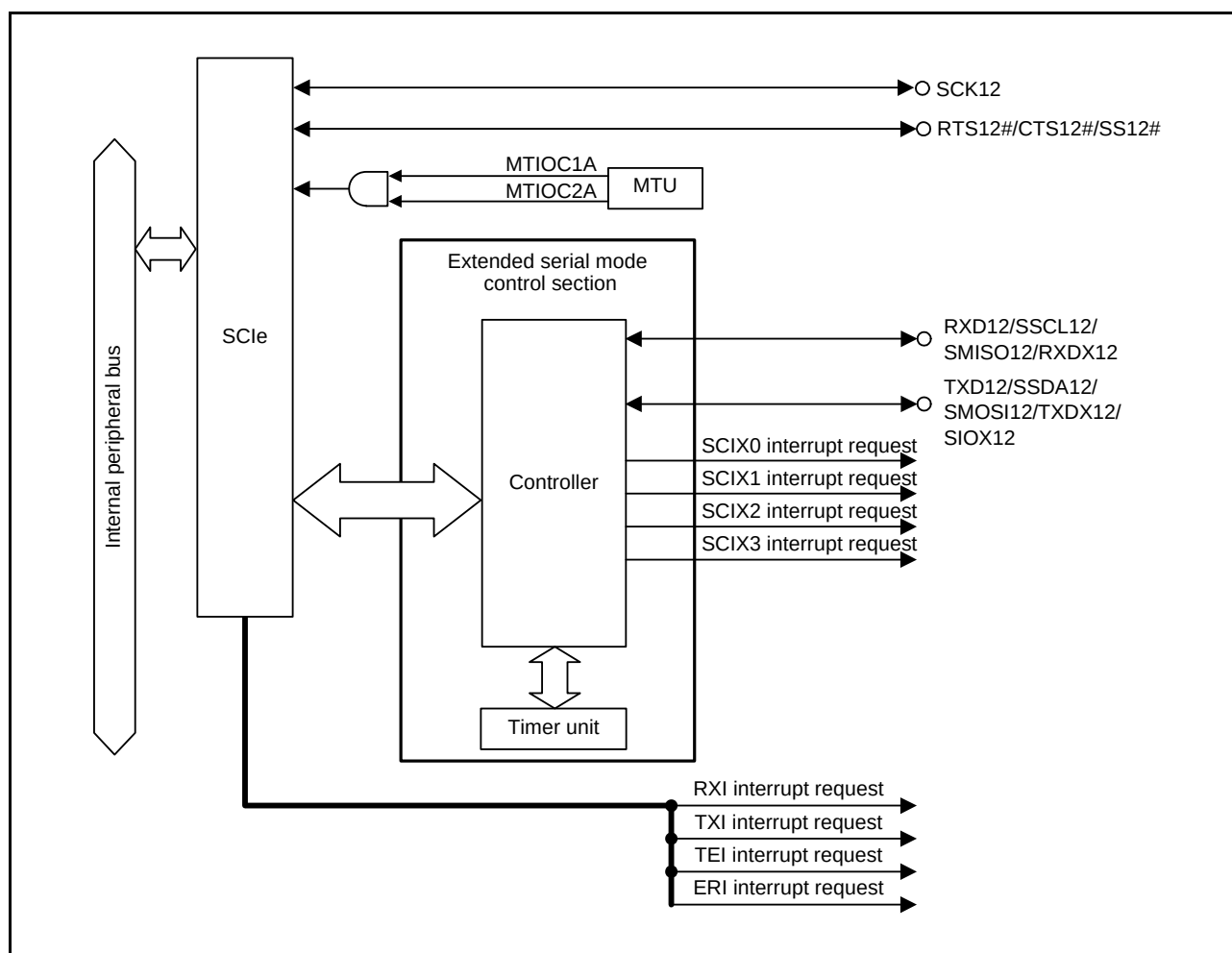
Figure 26.3 Block Diagram of SCIf (SCI12)
