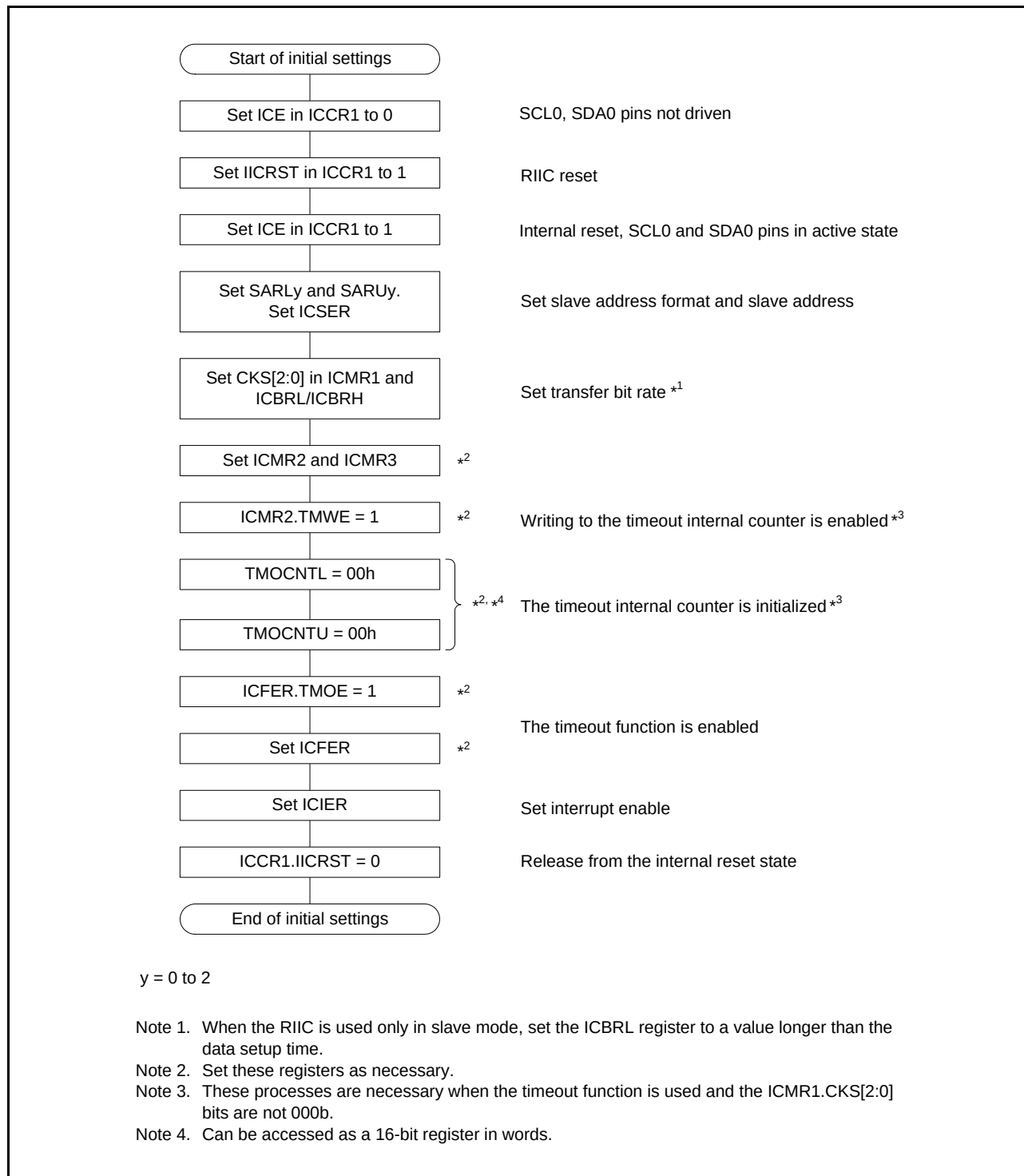
Figure 27.5 Example of RIIC Initialization Flowchart
