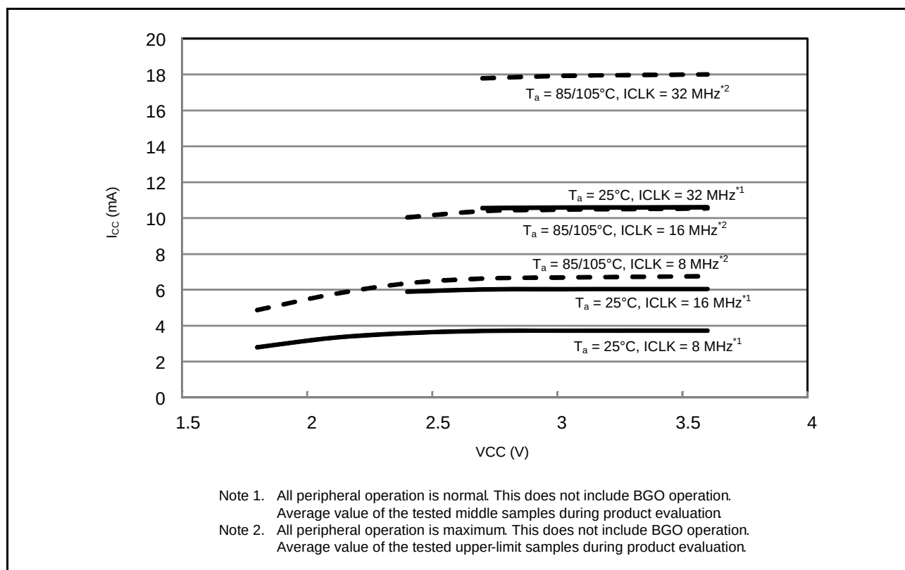
Figure 36.1 Voltage Dependency in High-Speed Operating Mode (Reference Data)
