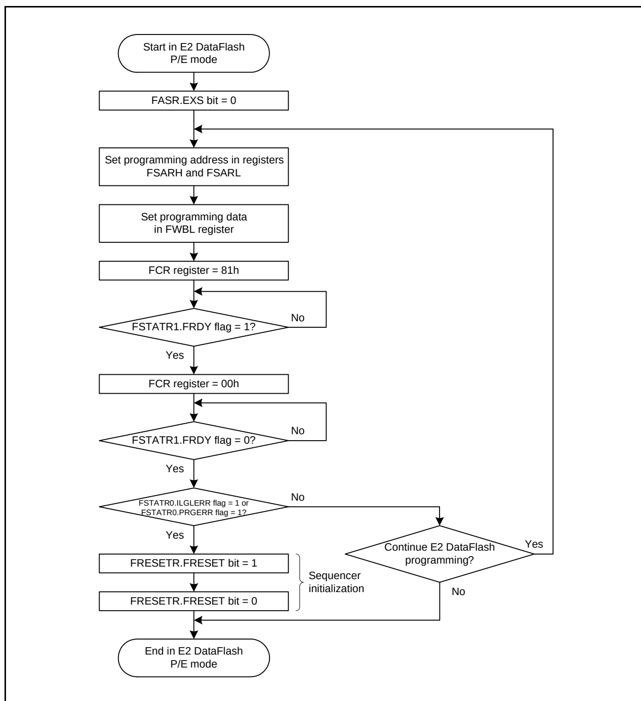
Figure 35.12 Procedure to Issue the Program Command for the E2 DataFlash
