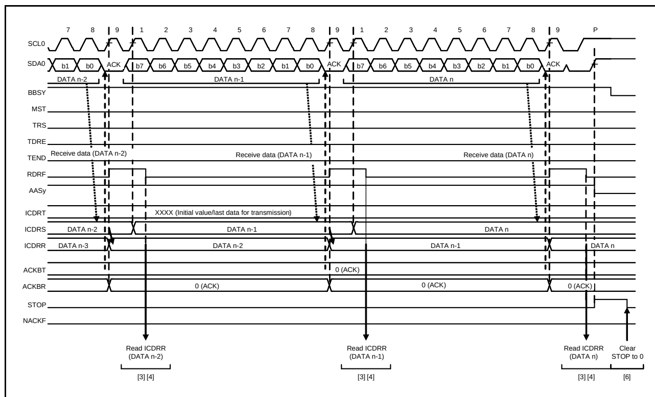
Figure 27.20 Slave Receive Operation Timing (2) (when RDRFS = 0)
