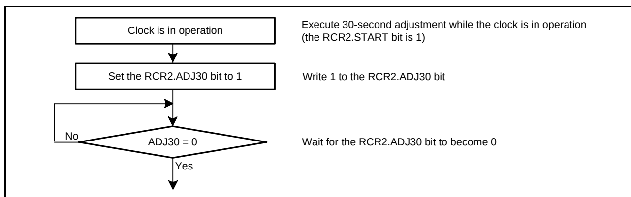
Figure 23.5 30-Second Adjustment
