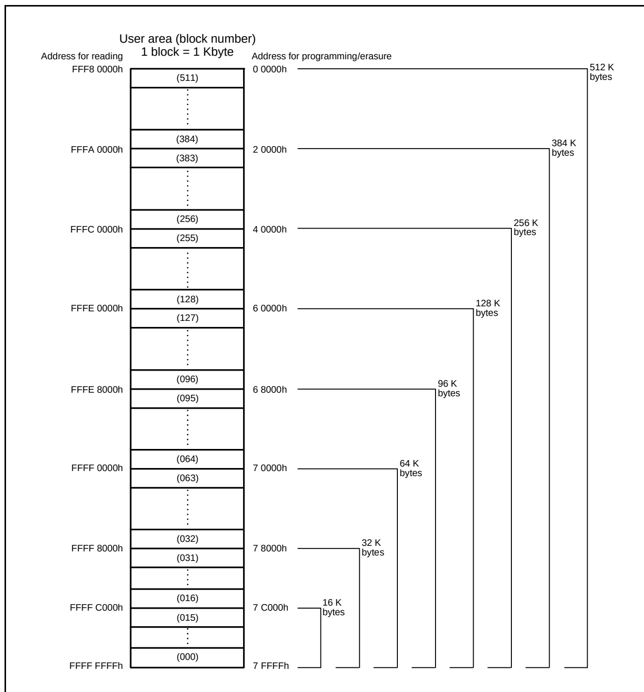
Figure 35.1 ROM Area and Block Configuration
