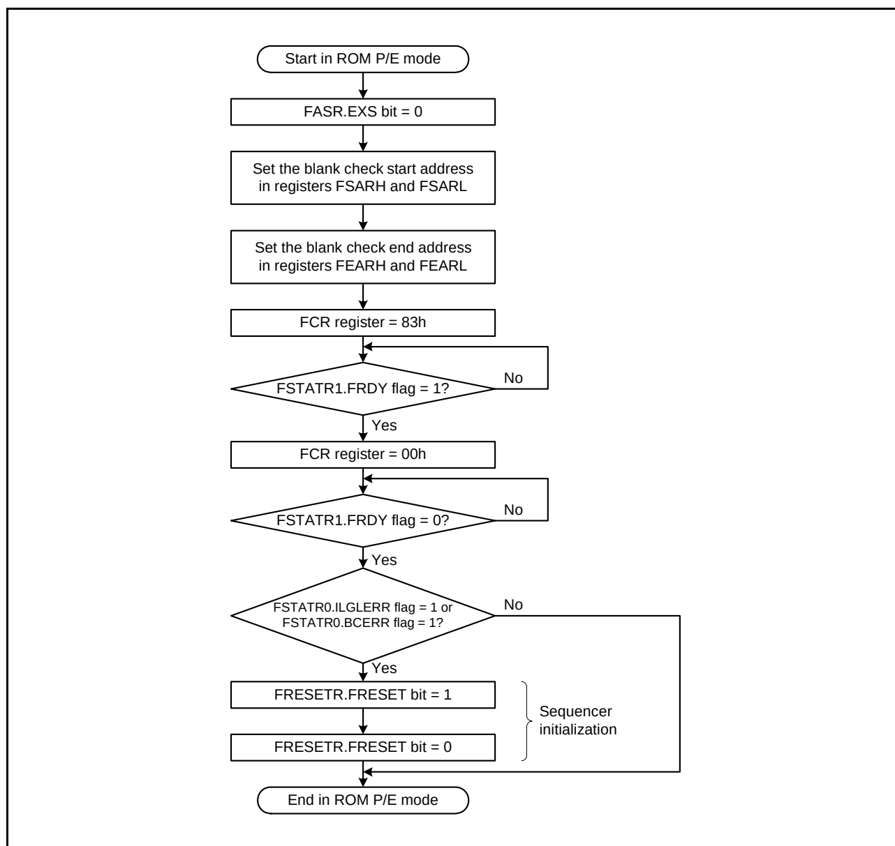
Figure 35.15 Procedure to Issue the Blank Check Command for the ROM
