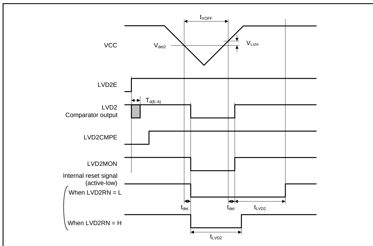
Figure 36.56 Voltage Detection Circuit Timing ( V_{det2} )
