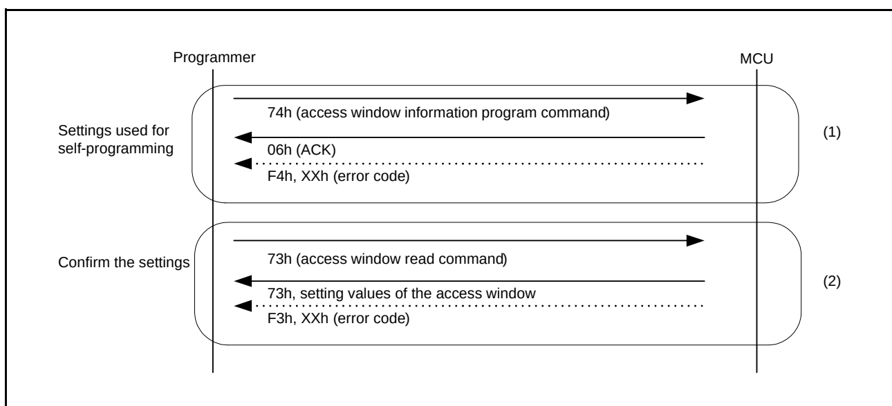
Figure 35.39 Procedure to Set the Access Window in the User Area
