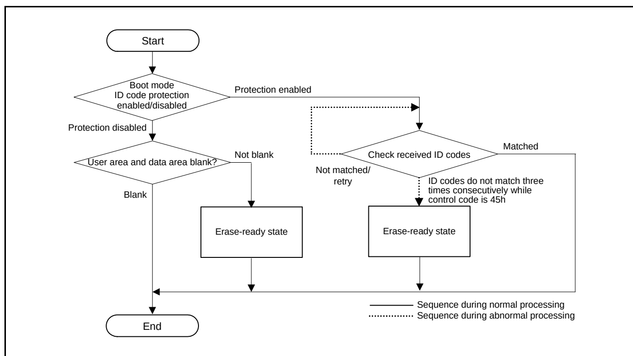
Figure 35.26 Authentication for Boot Mode ID Code Protection
