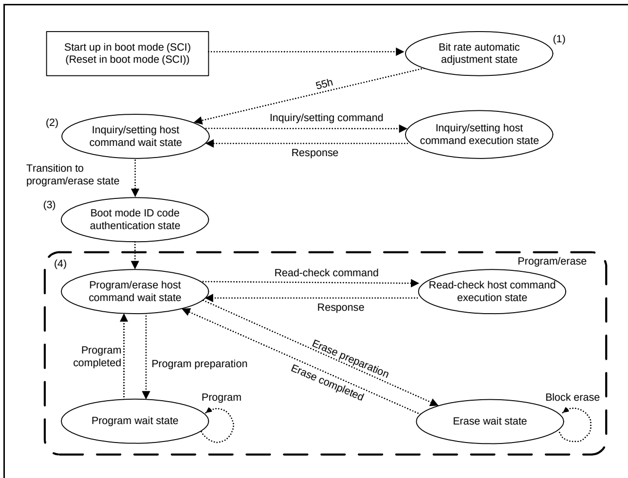
Figure 35.27 Boot Mode (SCI) State Transition
