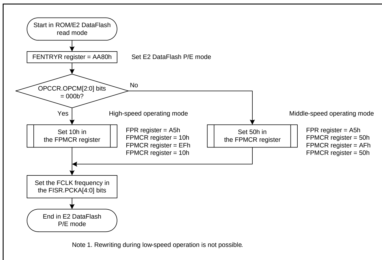
Figure 35.8 Procedure for Transition from ROM/E2 DataFlash Read Mode to E2 DataFlash P/E Mode
