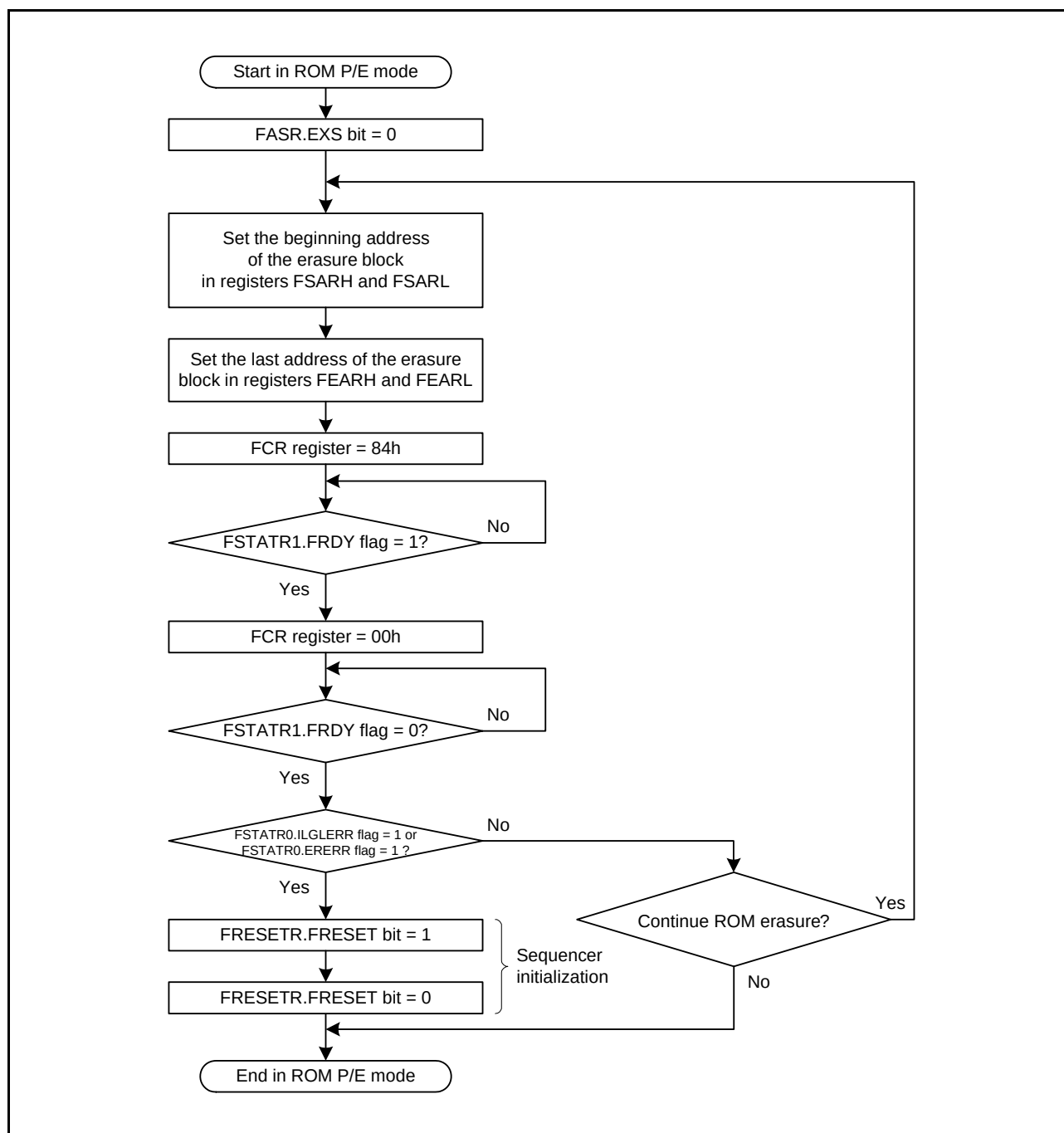
Figure 35.13 Procedure to Issue the Block Erase Command for the ROM
